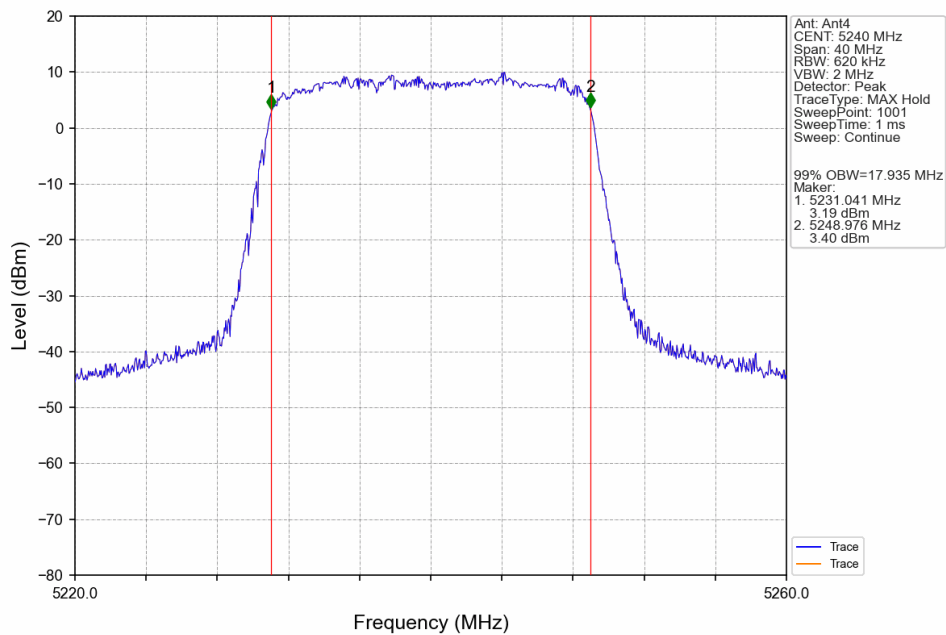
20M_HCH_5240MHz_Ant4_NTNV
