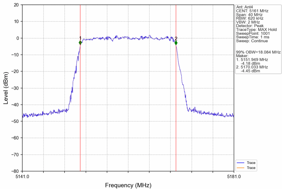
20M_LCH_5161MHz_Ant4_NTNV
