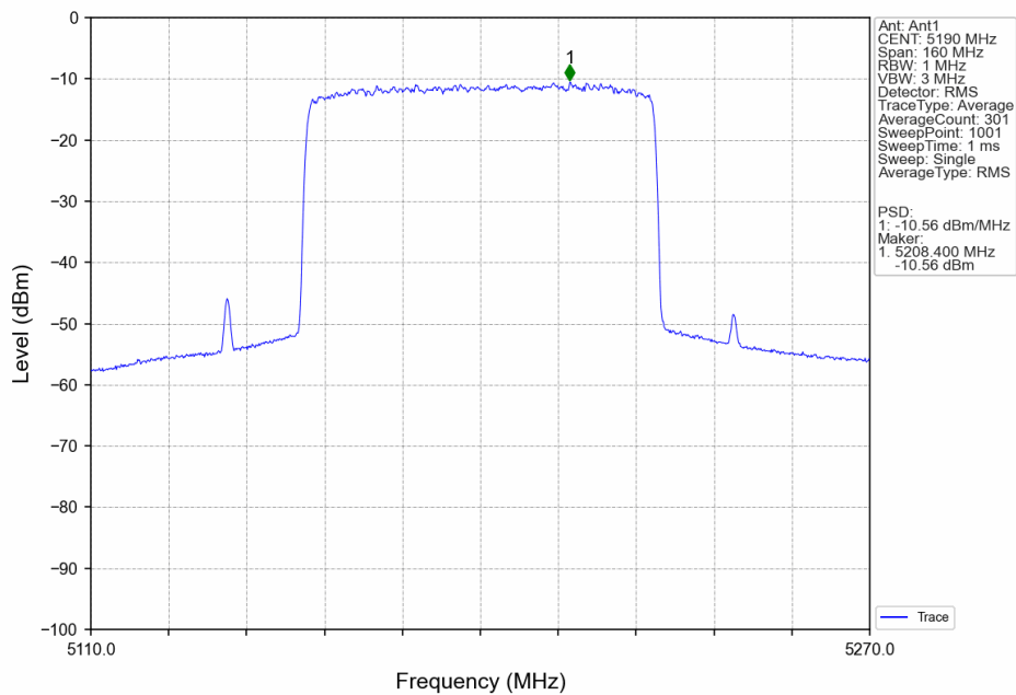
80M_LCH_5190MHz_Ant1_NTNV
