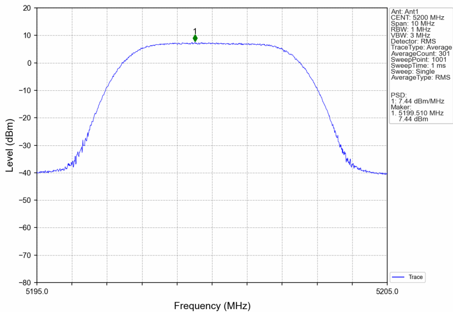
5M_MCH_5200MHz_Ant1_NTNV
