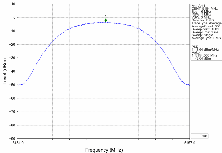
3M_LCH_5154MHz_Ant1_NTNV
