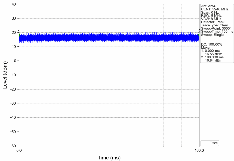
20M_HCH_5240MHz_Ant4_NTNV
