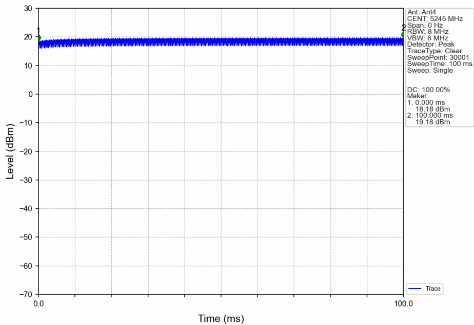
5M_HCH_5245MHz_Ant4_NTNV
