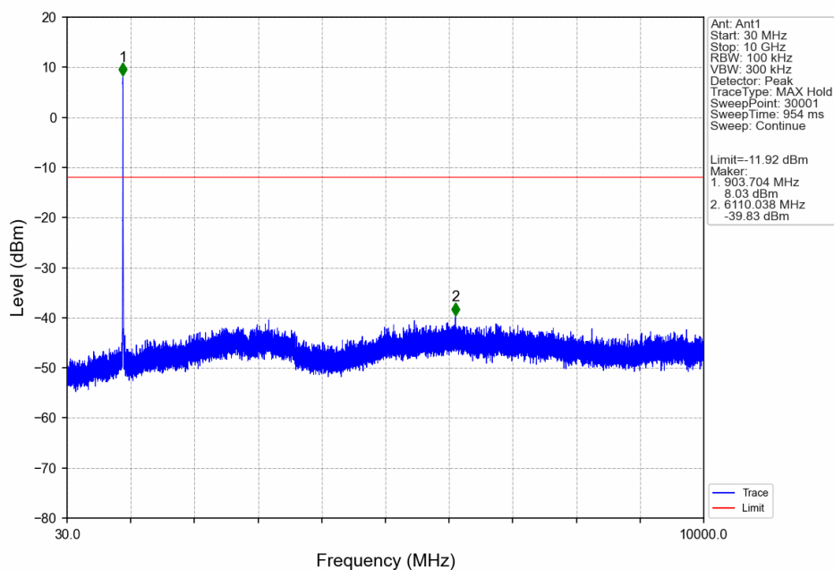
5M_LCH_904.6MHz_Ant1_NTNV
