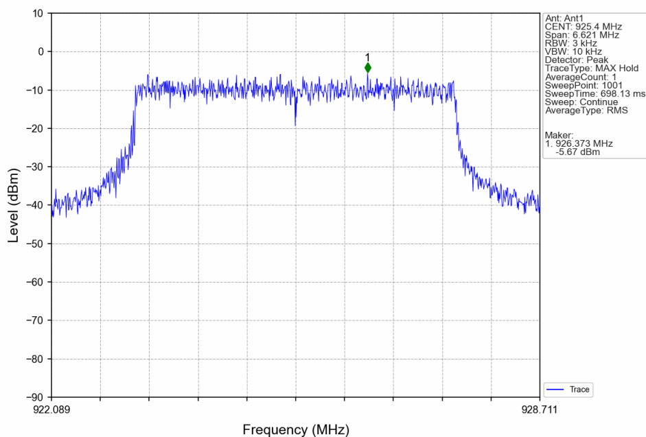
5M_HCH_925.4MHz_Ant1_NTNV
