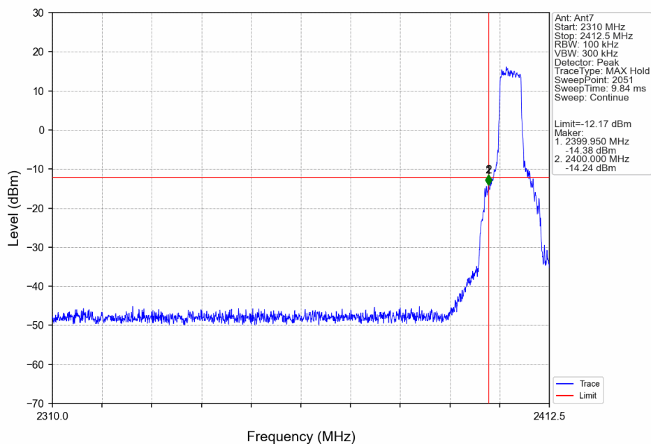
5M_LCH_2404.5MHz_Ant7_NTNV
