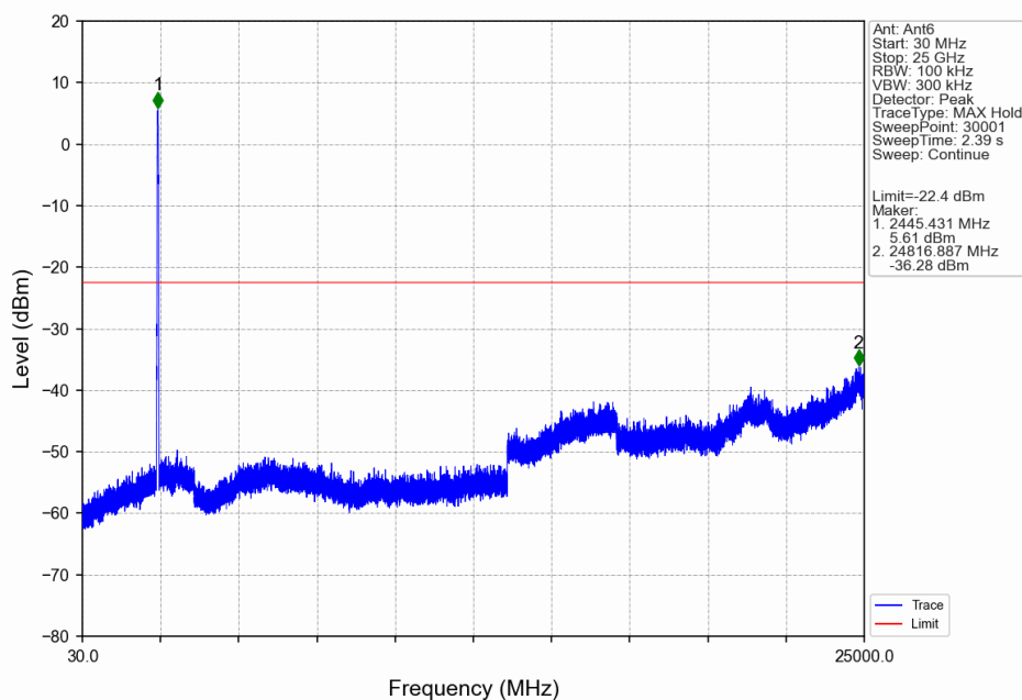
60M_HCH_2442.5MHz_Ant6_NTNV
