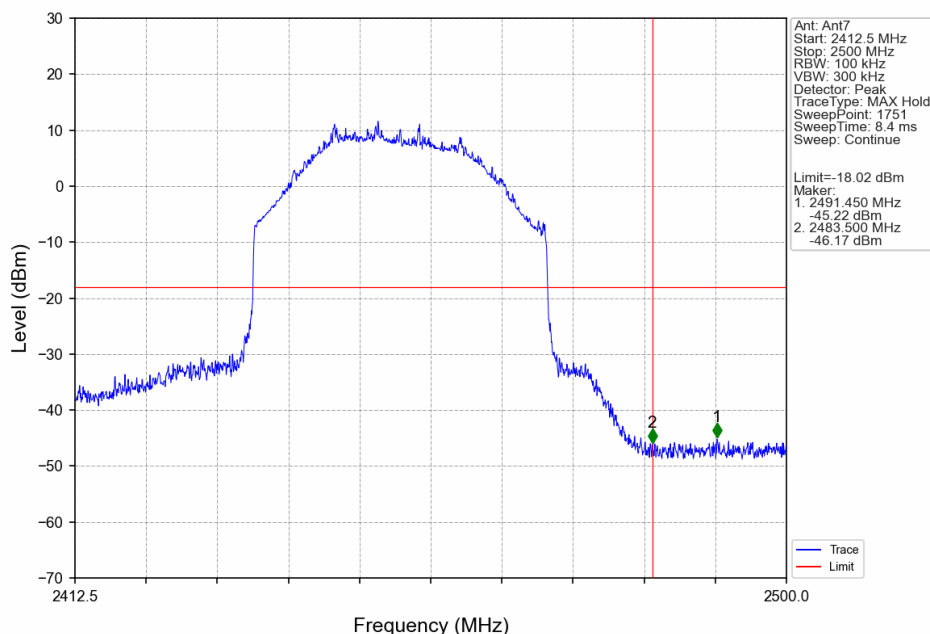
40M_HCH_2452.5MHz_Ant7_NTNV
