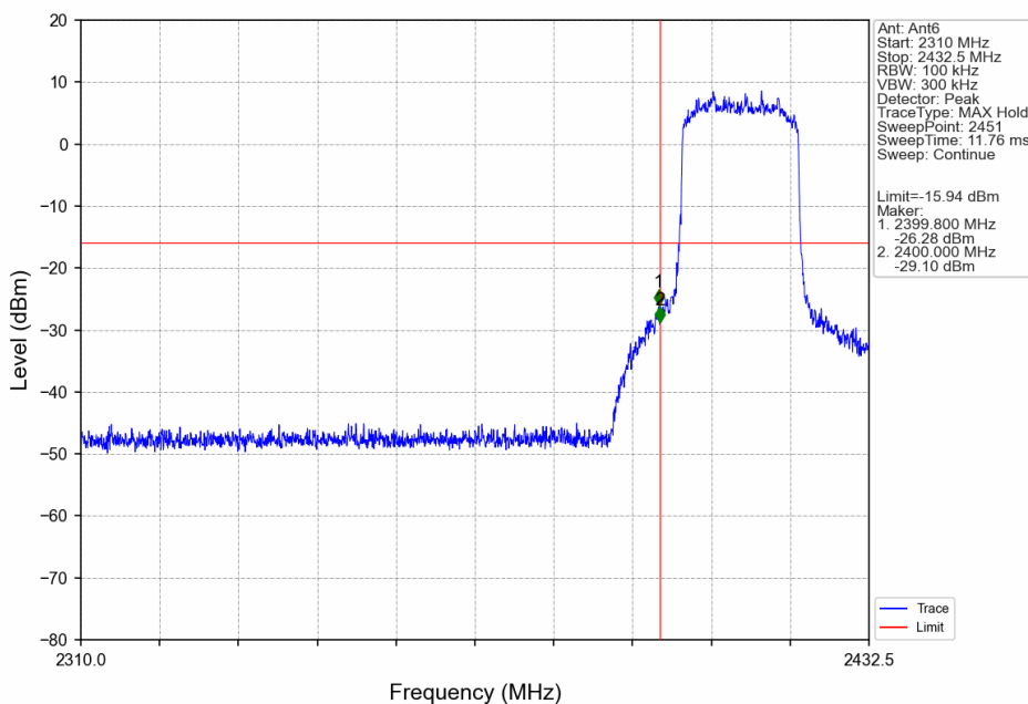
20M_LCH_2412.5MHz_Ant6_NTNV
