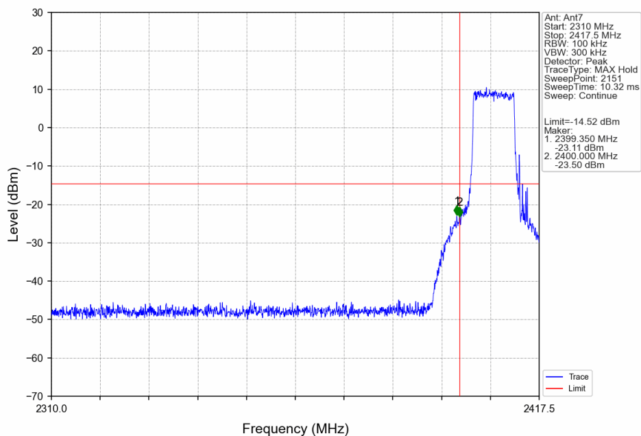
10M_LCH_2407.5MHz_Ant7_NTNV
