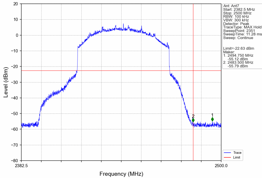
60M_HCH_2442.5MHz_Ant7_NTNV
