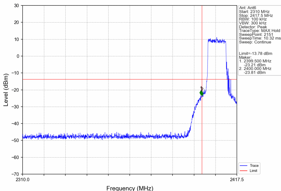
10M_LCH_2407.5MHz_Ant6_NTNV
