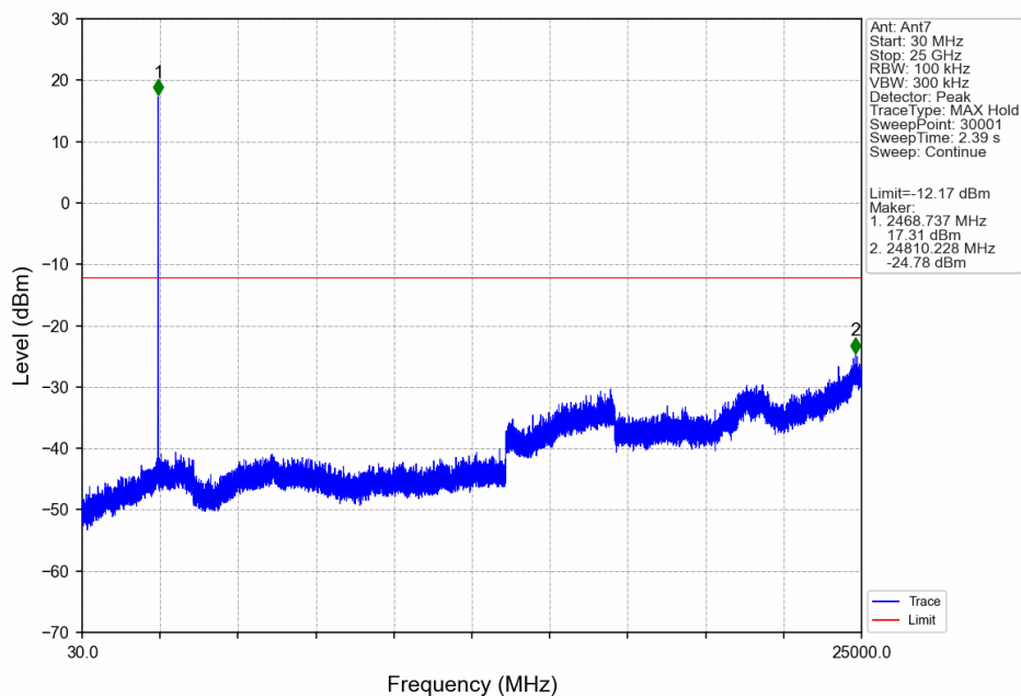
5M_HCH_2469.5MHz_Ant7_NTNV
