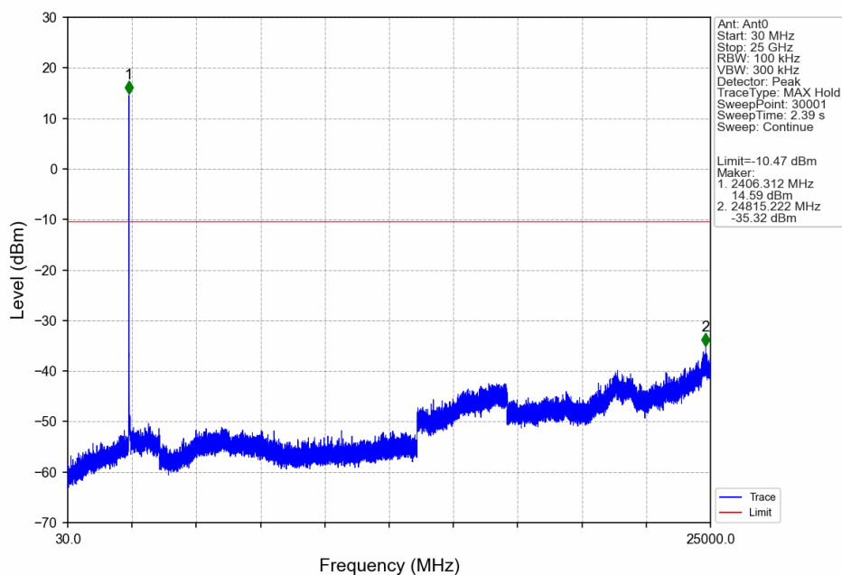
5M_LCH_2404.5MHz_Ant0_NTNV
