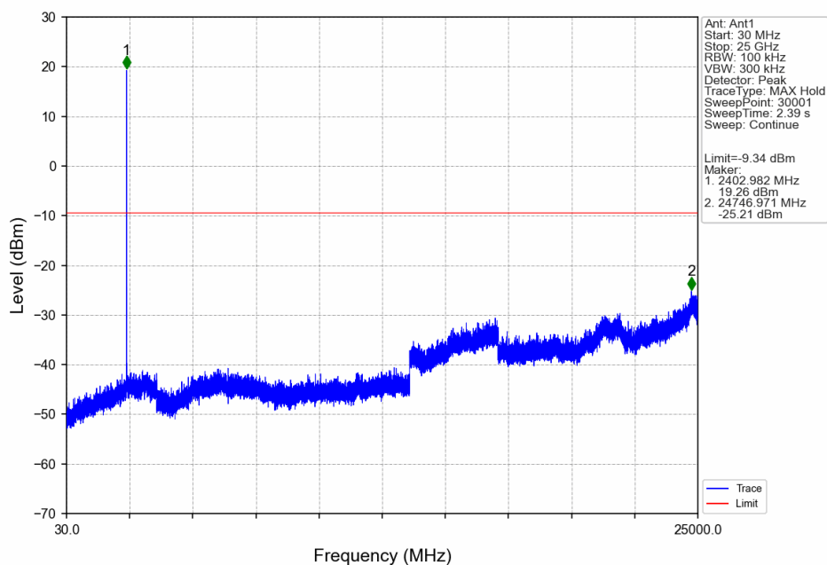
1.4M_LCH_2403.5MHz_Ant1_NTNV
