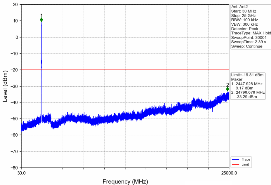
40MHz BW_MCH_2437.5MHz_Ant2_NTNV
