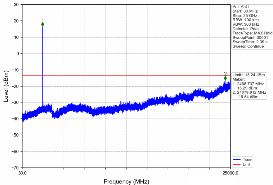
1.4MHz BW_HCH_2469.5MHz_Ant1_NTNV
