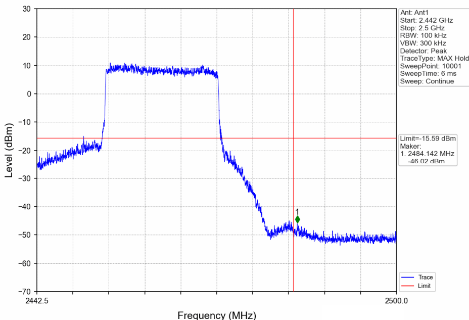
20MHz BW_HCH_2462.5MHz_Ant1_NTNV
