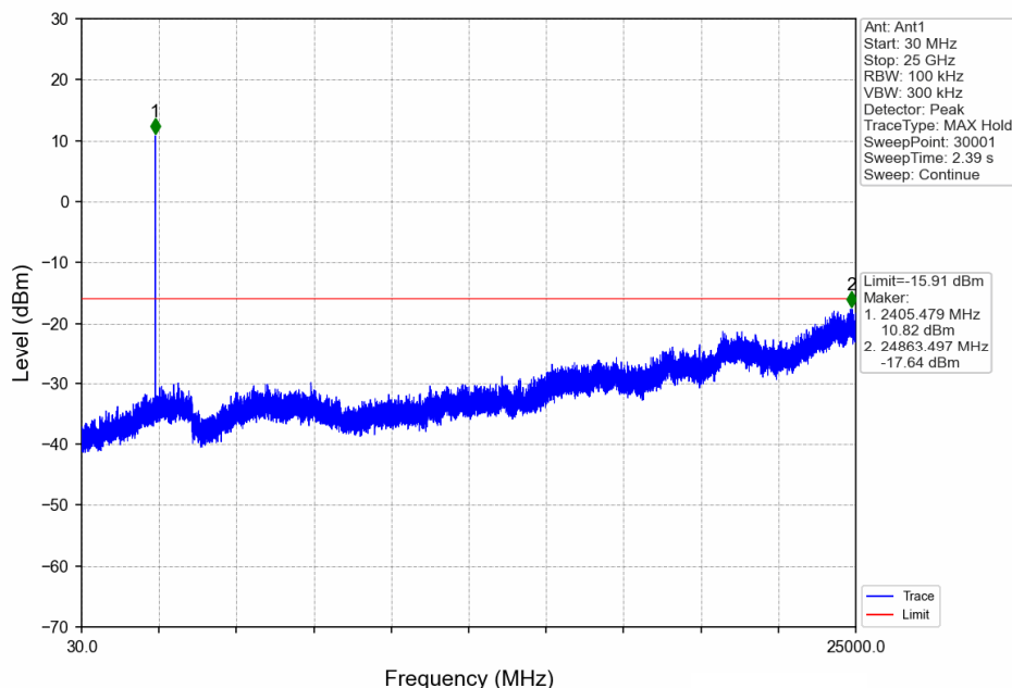
3MHz BW_LCH_2405.5MHz_Ant1_NTNV
