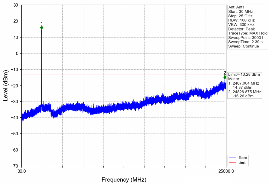
10MHz BW_HCH_2467.5MHz_Ant1_NTNV
