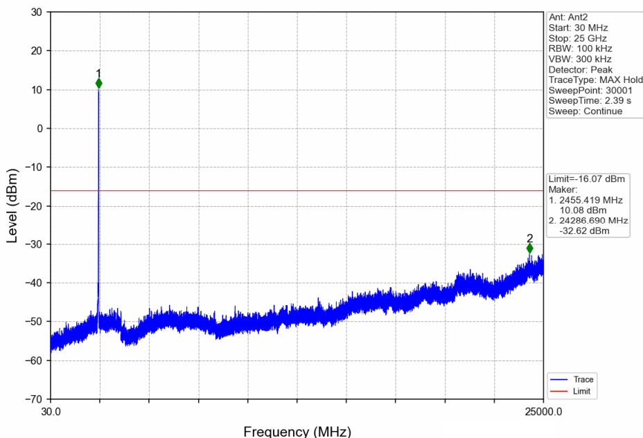
20MHz BW_HCH_2462.5MHz_Ant2_NTNV
