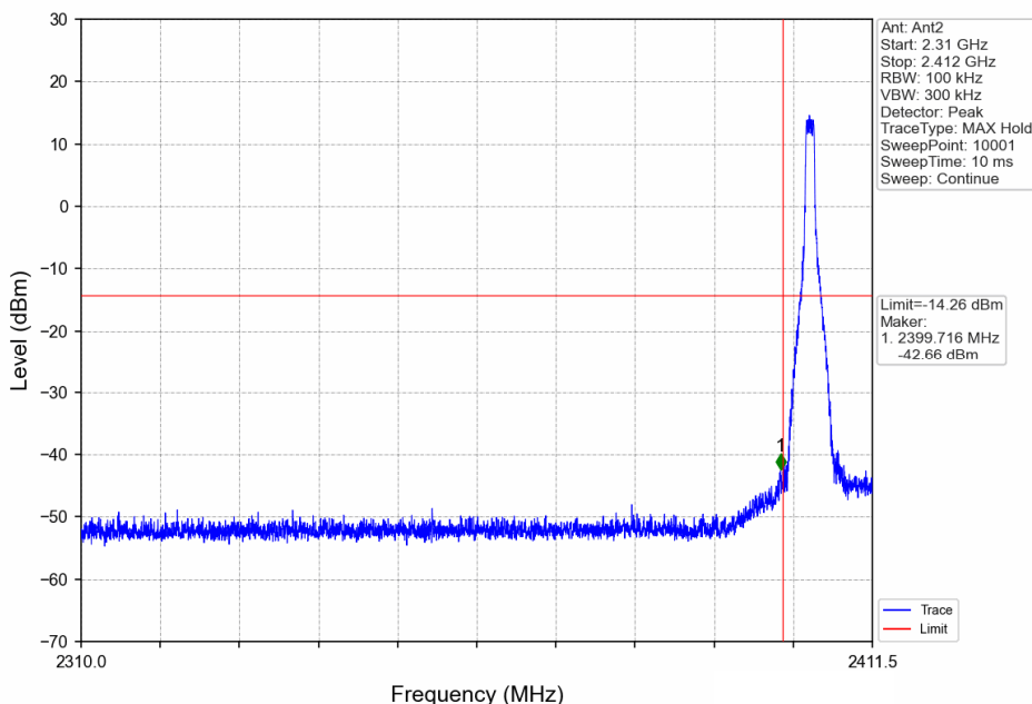
1.4MHz BW_LCH_2403.5MHz_Ant2_NTNV
