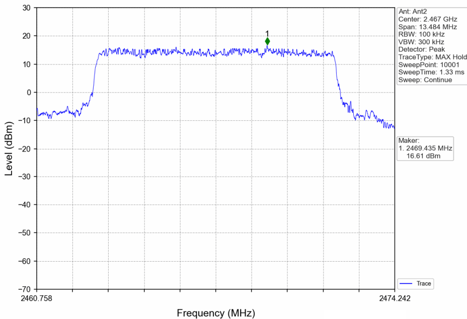
10MHz BW_HCH_2467.5MHz_Ant2_NTNV
