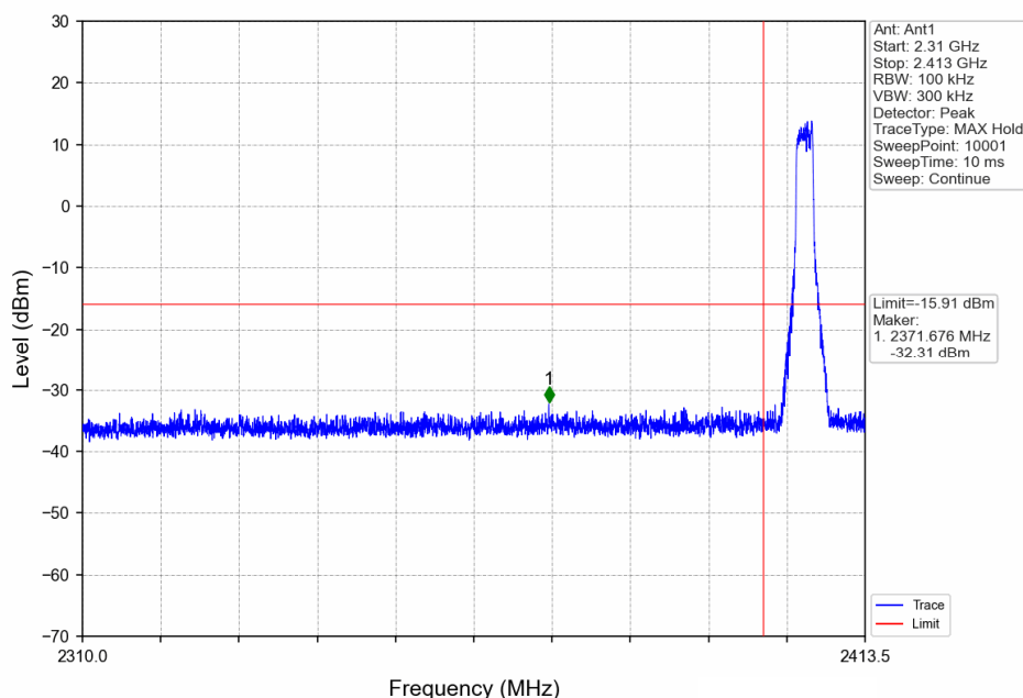
3MHz BW_LCH_2405.5MHz_Ant1_NTNV
