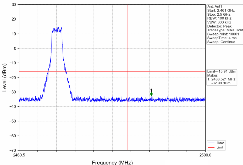
3MHz BW_HCH_2468.5MHz_Ant1_NTNV
