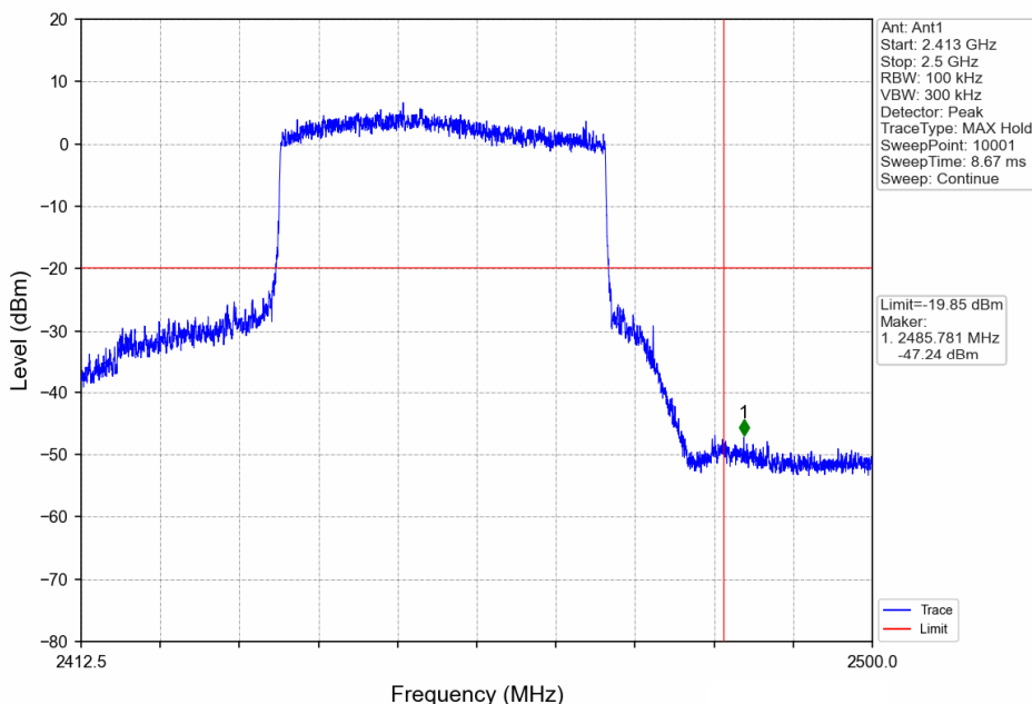
40MHz BW_HCH_2452.5MHz_Ant1_NTNV
