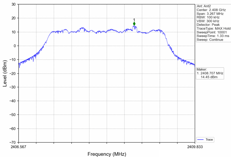
3MHz CA BW_LCH_2408.2MHz_Ant2_NTNV
