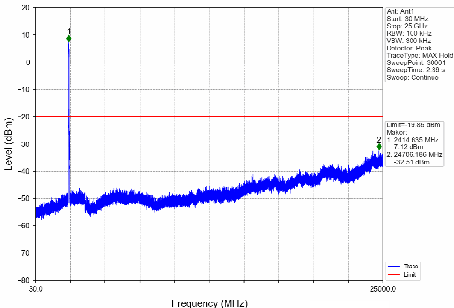
40MHz BW_LCH_2422.5MHz_Ant1_NTNV
