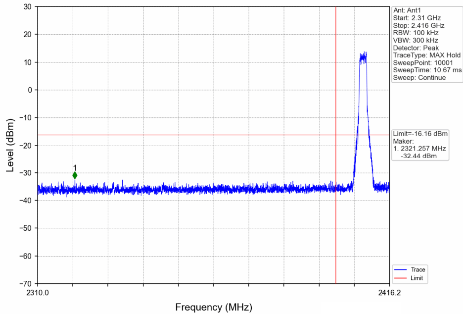
3MHz CA BW_LCH_2408.2MHz_Ant1_NTNV
