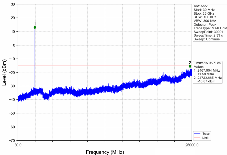
3MHz BW_HCH_2468.5MHz_Ant2_NTNV
