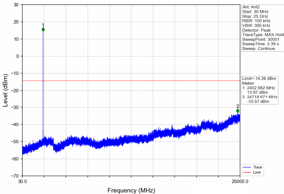
1.4MHz BW_LCH_2403.5MHz_Ant2_NTNV
