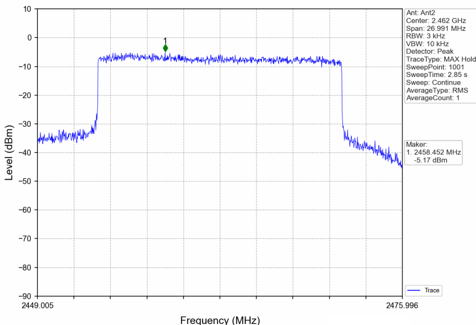
20MHz BW_HCH_2462.5MHz_MIMO_NTNV
