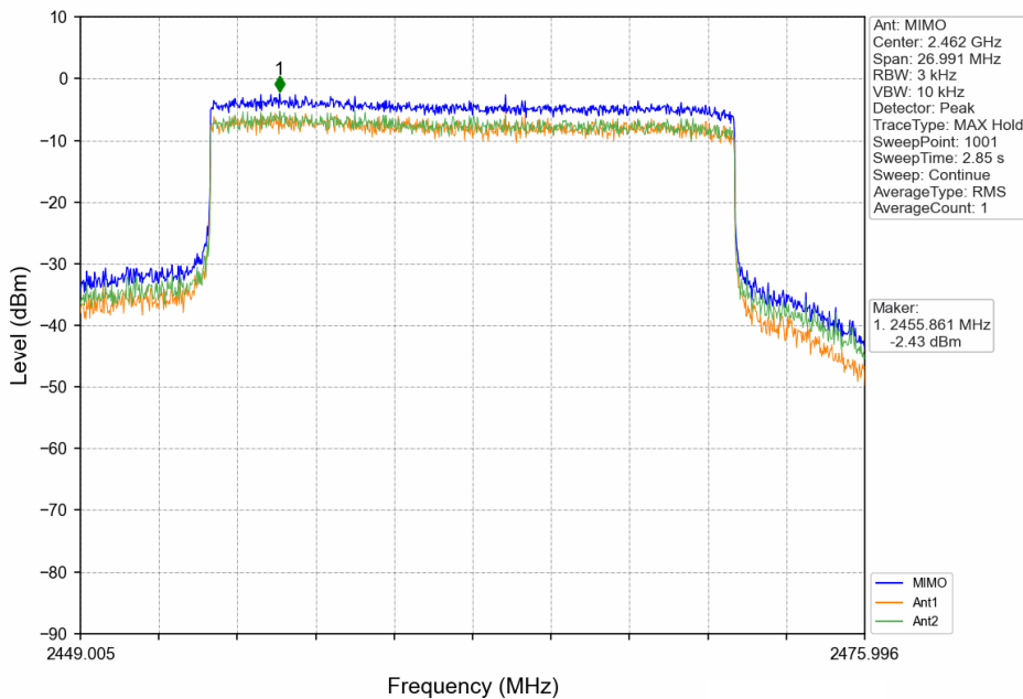
20MHz BW_HCH_2462.5MHz_MIMO_NTNV
