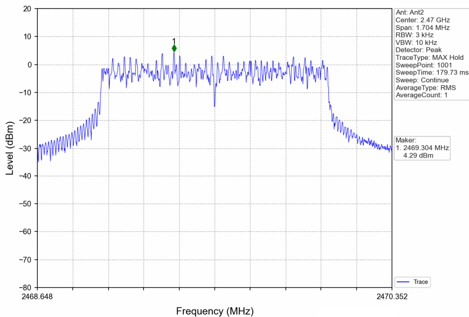
1.4MHz BW_HCH_2469.5MHz_Ant2_NTNV
