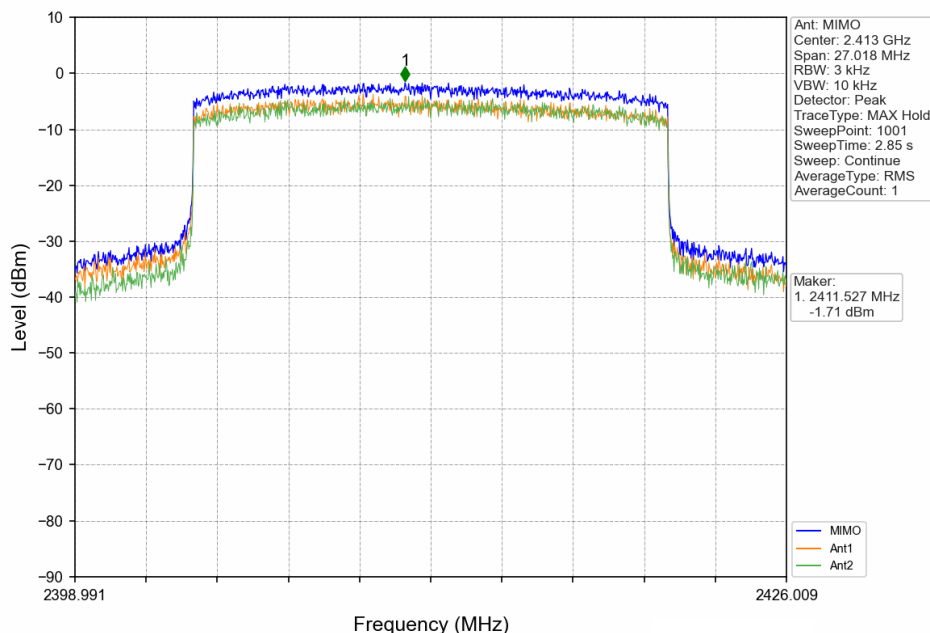
20MHz BW_LCH_2412.5MHz_MIMO_NTNV
