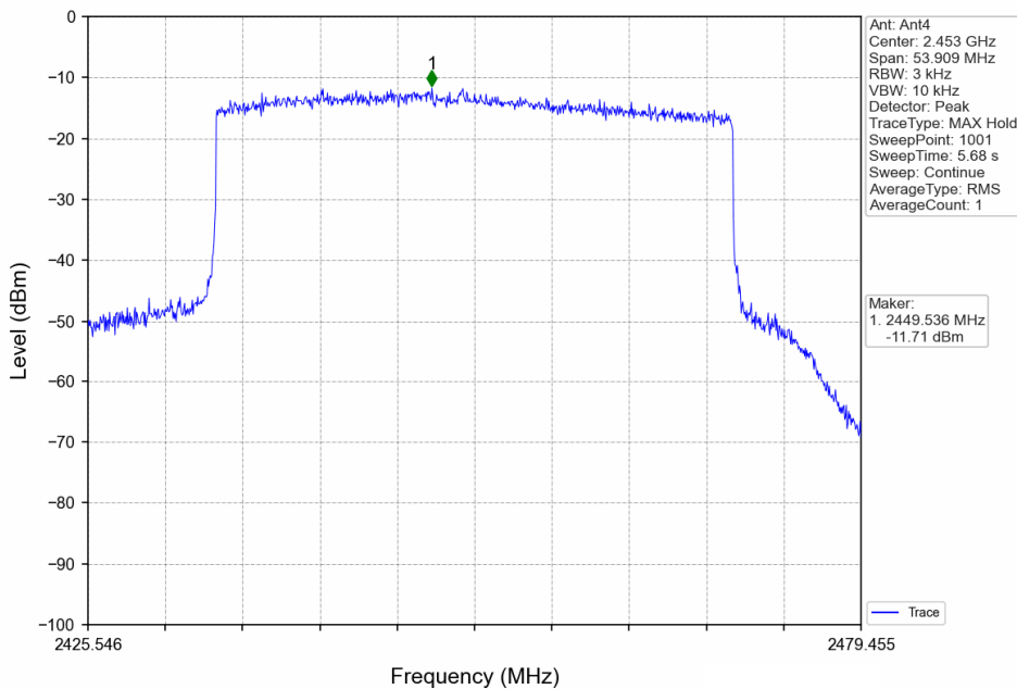
40MHz BW_HCH_2452.5MHz_Ant4_NTNV
