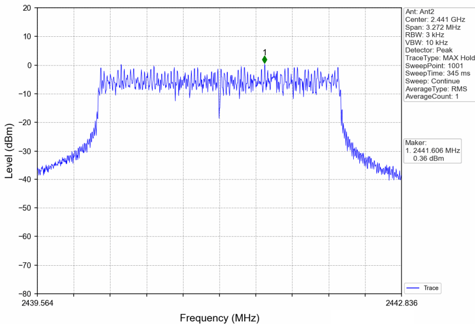
3MHz CA BW_MCH_2441.2MHz_Ant2_NTNV
