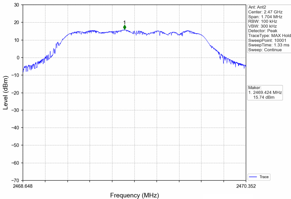
1.4MHz BW_HCH_2469.5MHz_Ant2_NTNV
