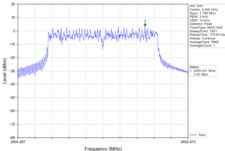
1.4MHz CA BW_LCH_2405.12MHz_Ant1_NTNV
