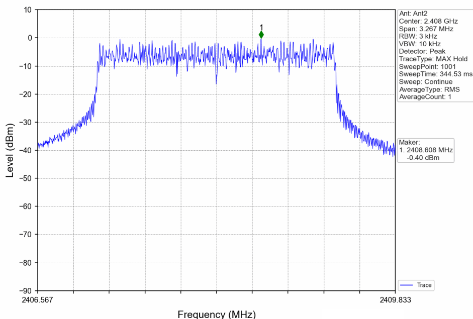
3MHz CA BW_LCH_2408.2MHz_MIMO_NTNV
