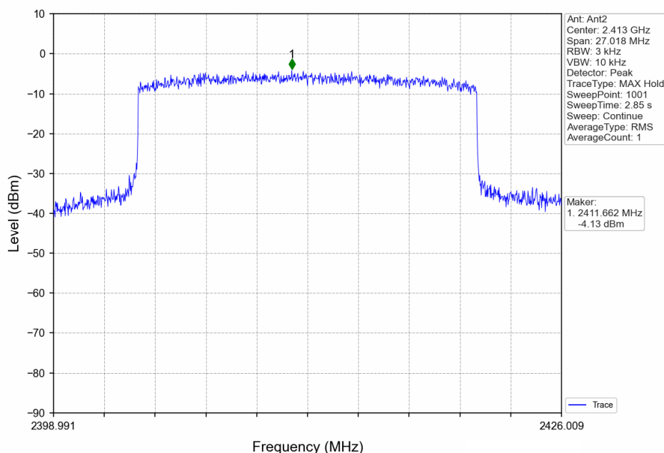
20MHz BW_LCH_2412.5MHz_MIMO_NTNV
