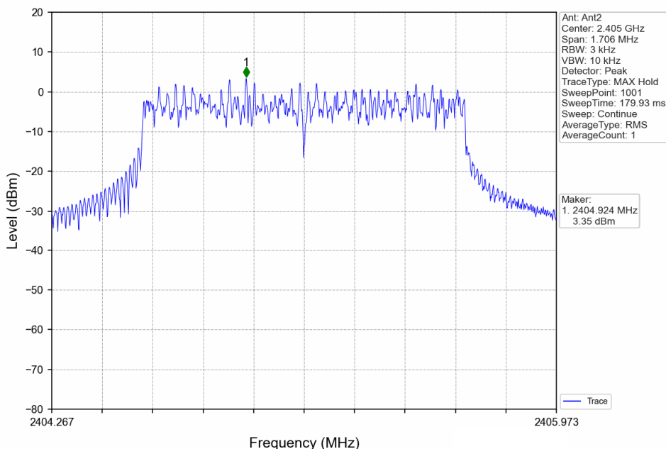
1.4MHz CA BW_LCH_2405.12MHz_MIMO_NTNV
