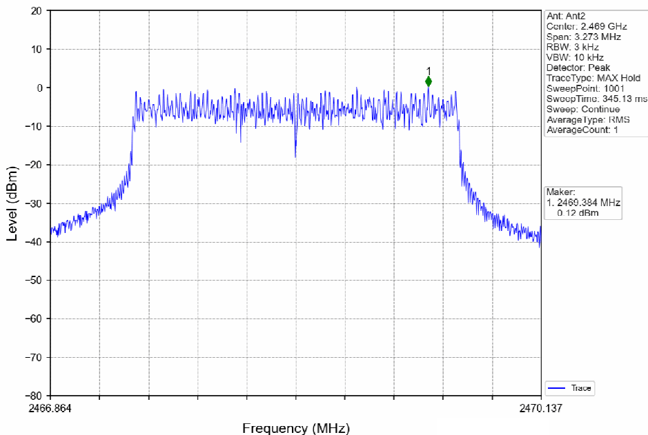
3MHz BW_HCH_2468.5MHz_Ant2_NTNV
