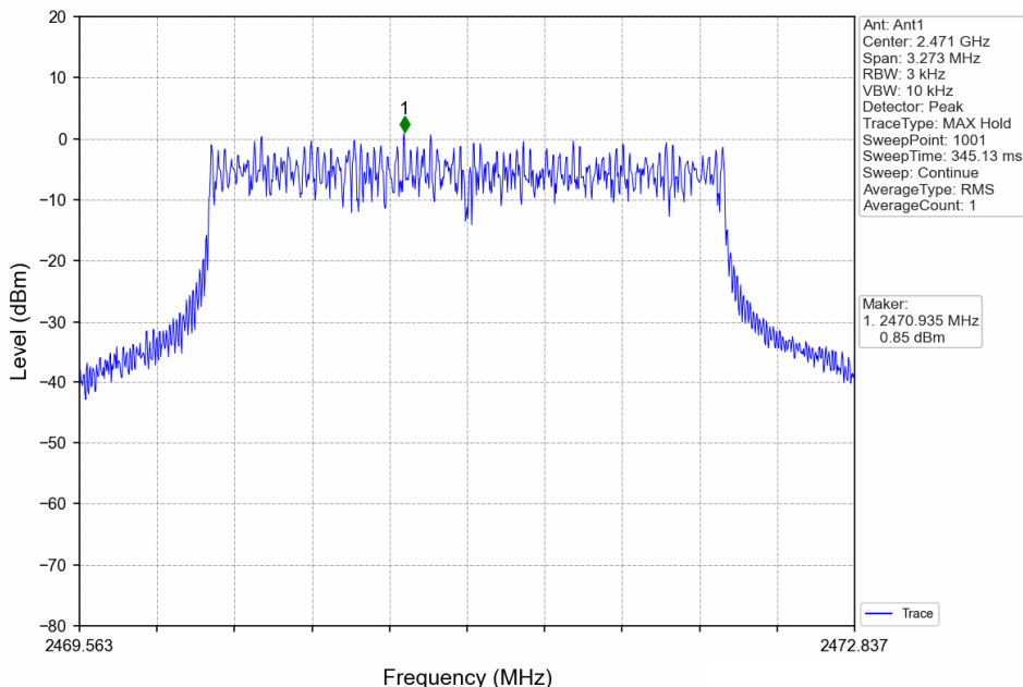
3MHz CA BW_HCH_2471.2MHz_Ant1_NTNV
