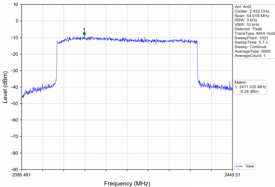
40MHz BW_LCH_2422.5MHz_Ant2_NTNV
