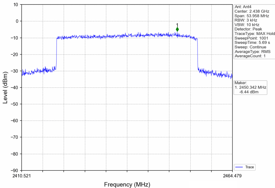
40MHz BW_MCH_2437.5MHz_Ant4_NTNV
