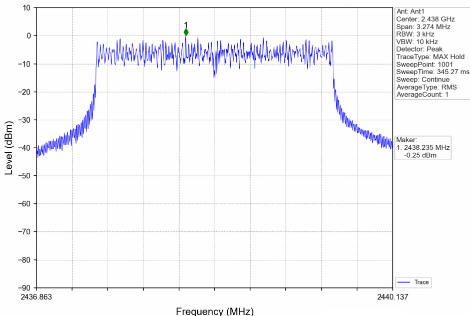
3MHz BW_MCH_2438.5MHz_Ant1_NTNV
