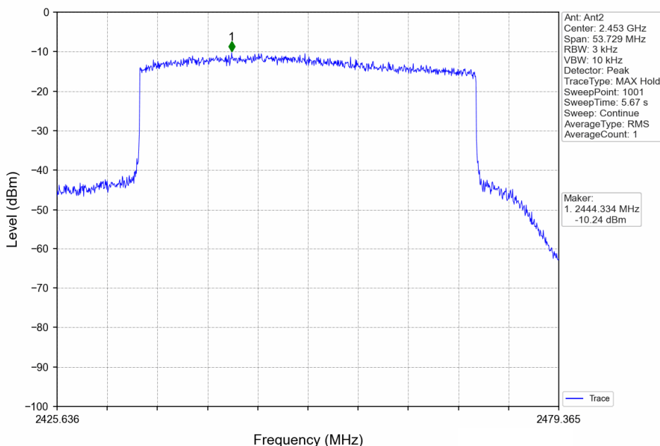
40MHz BW_HCH_2452.5MHz_Ant2_NTNV
