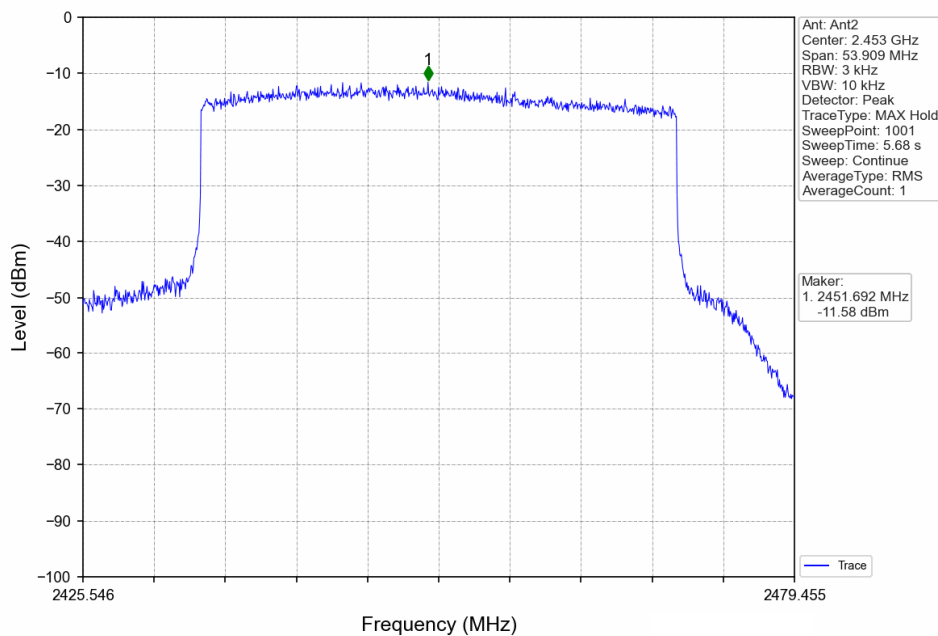
40MHz BW_HCH_2452.5MHz_Ant2_NTNV
