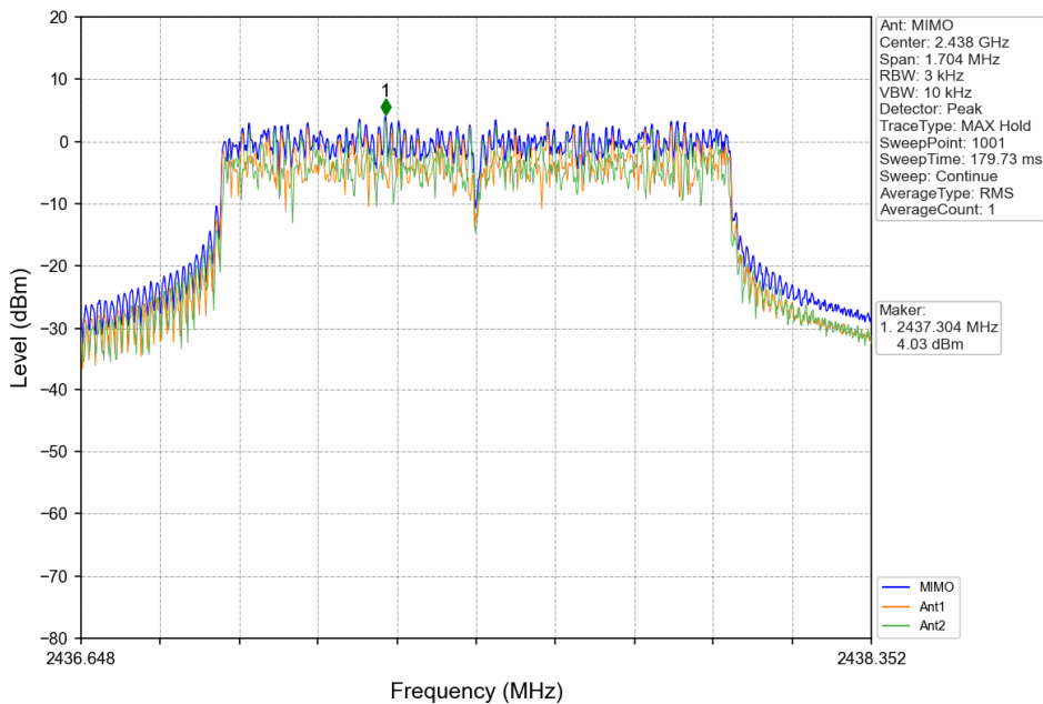
1.4MHz BW_MCH_2437.5MHz_MIMO_NTNV
