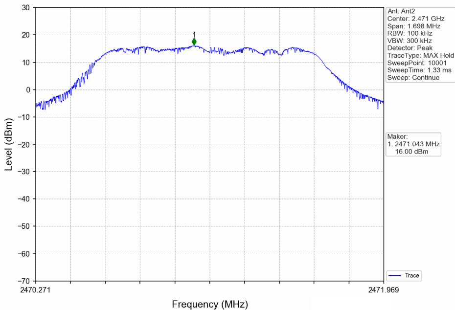
1.4MHz CA BW_HCH_2471.12MHz_Ant2_NTNV
