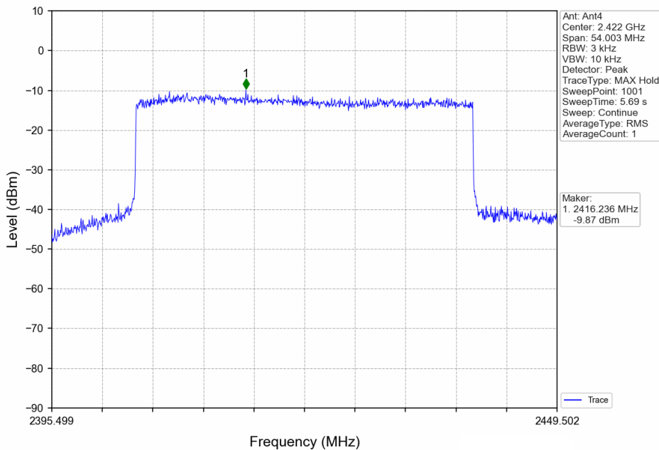
40MHz BW_LCH_2422.5MHz_Ant4_NTNV
