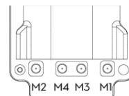
Antenna Ports on back of the flight controller
