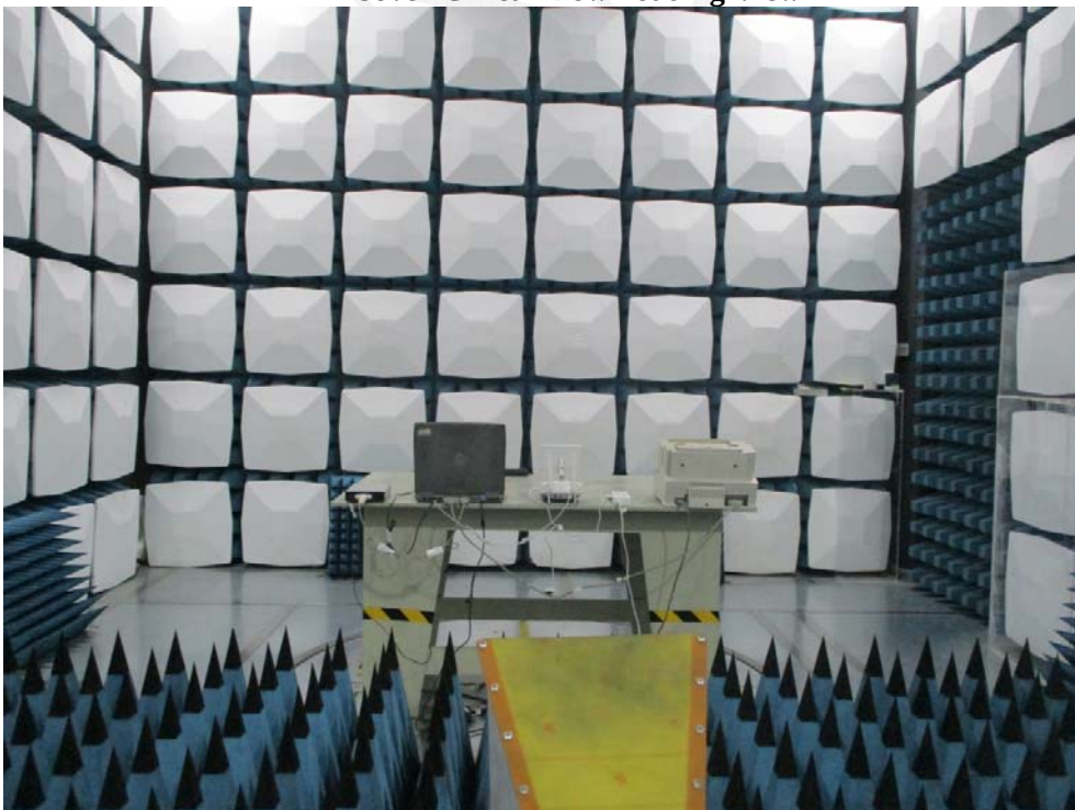
RE Above 1G Rear Downloading View
