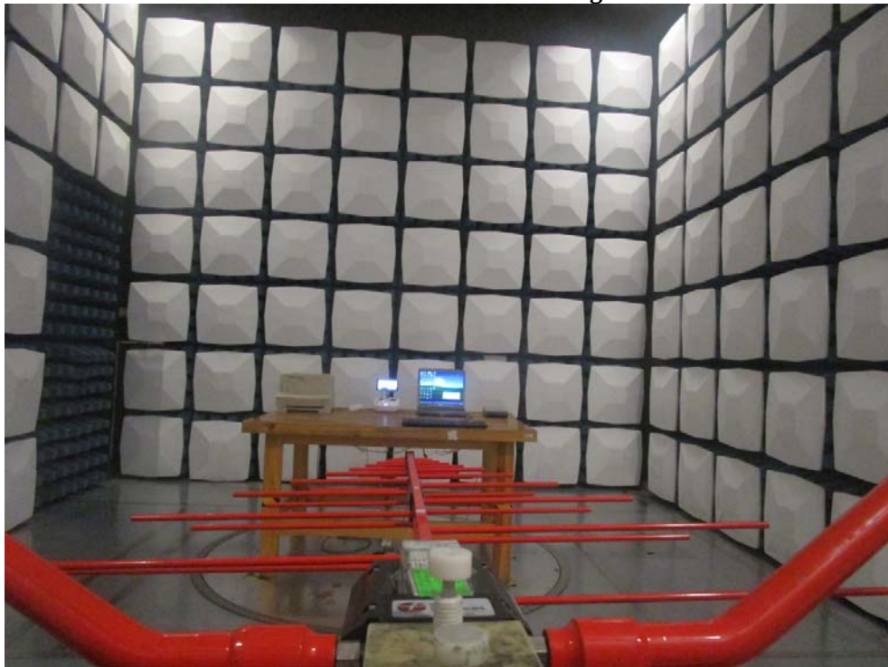
RE Below 1G Front Downloading View
