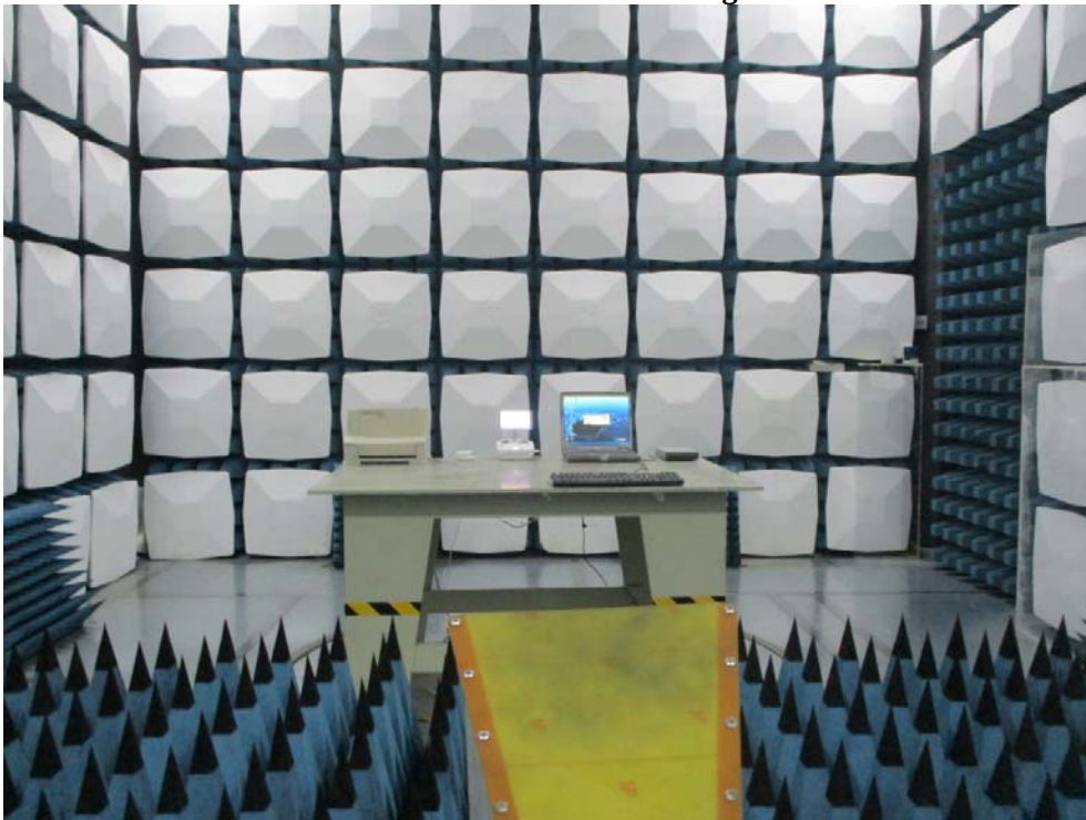
RE Above 1G Front Downloading View
