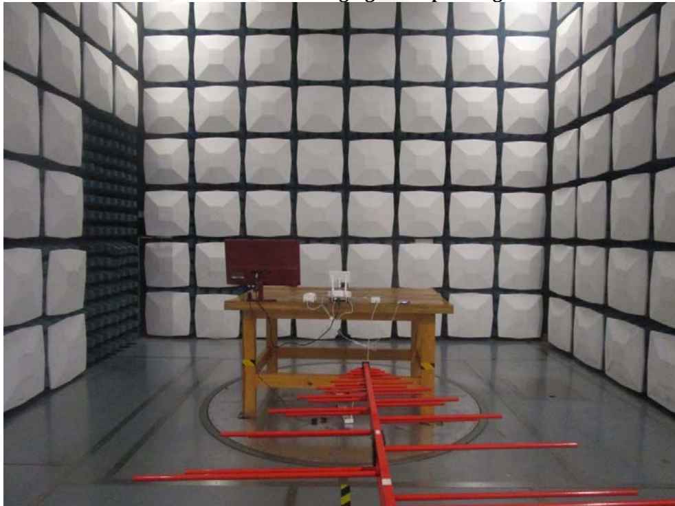
RE Below 1G Rear Charging and Operating View
