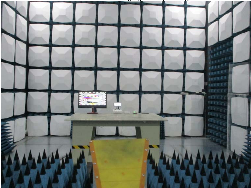
RE Above 1G Rear Charging and Operating View
