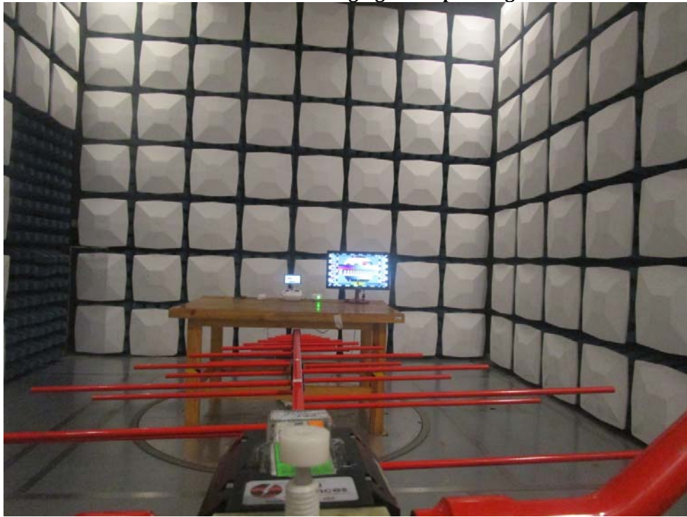
RE Below 1G Front Charging and Operating View
