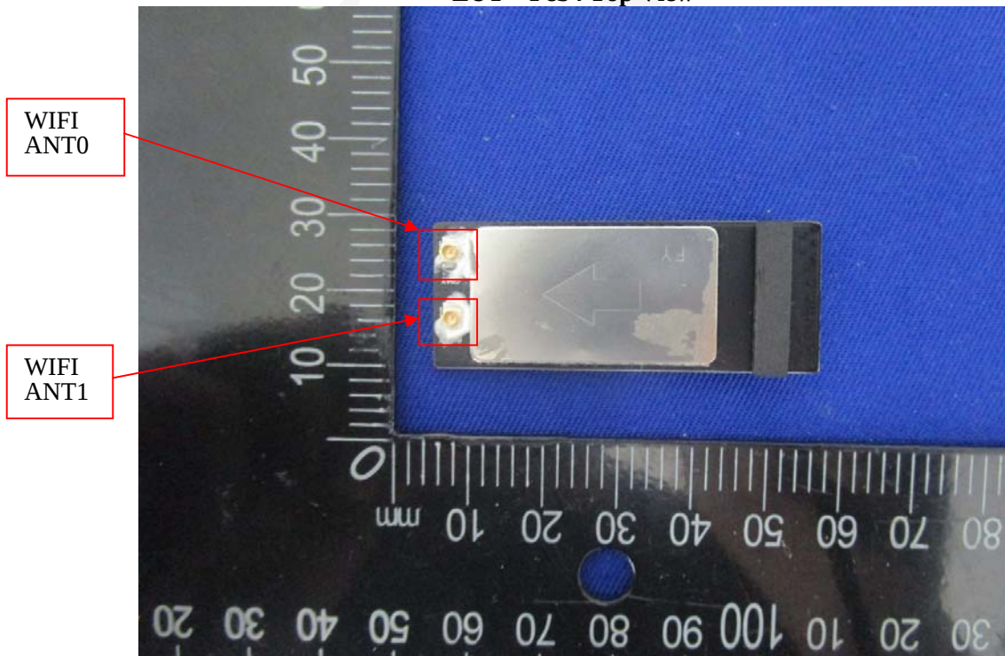
EUT – Pcb4 Top View
