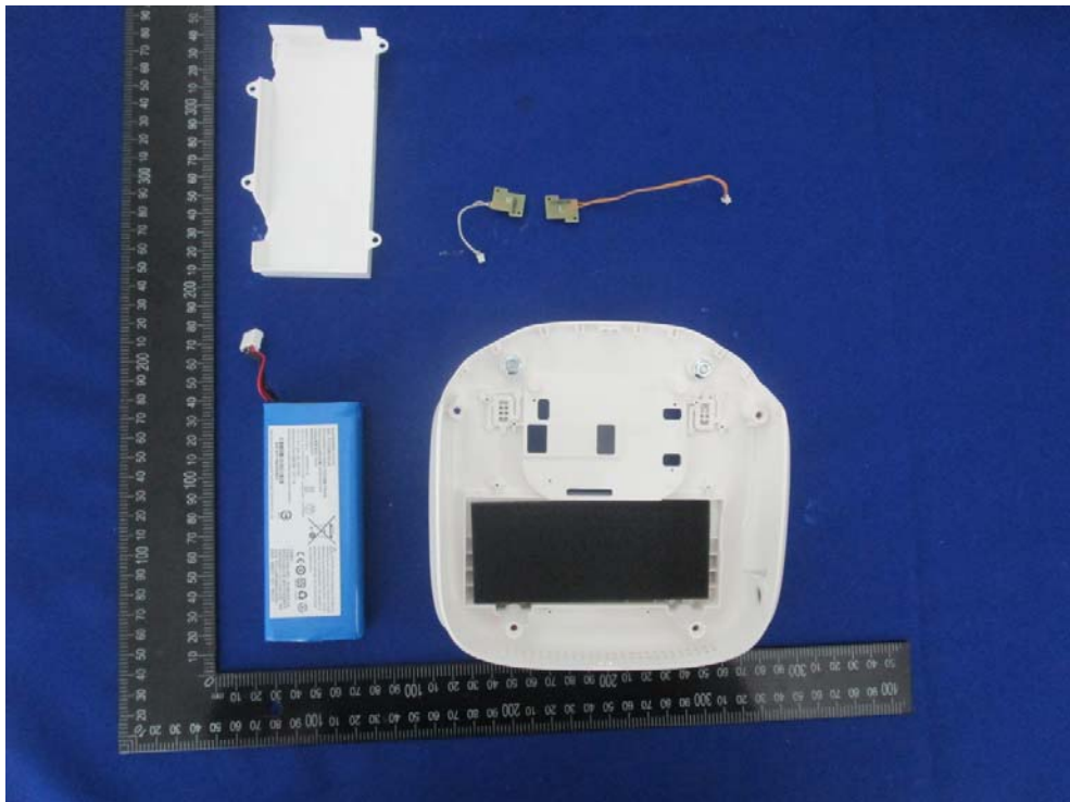
EUT – Uncover5 View
