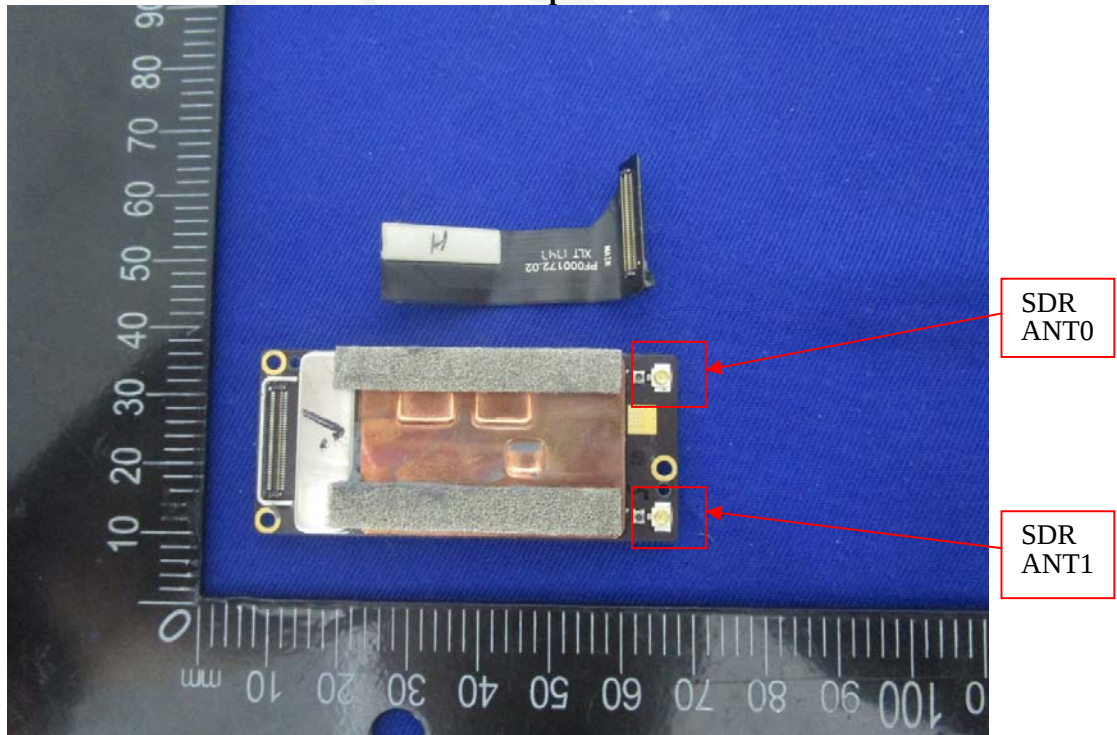
EUT – Pcb7 Top View
