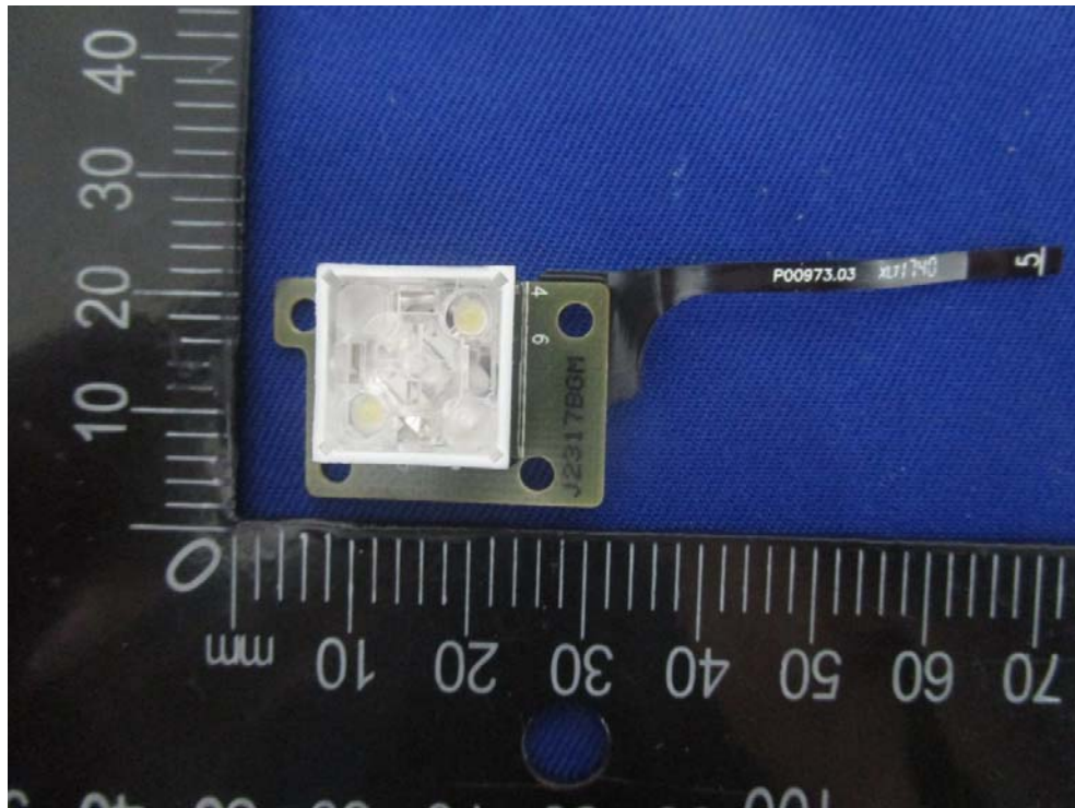
EUT – Button1 Pcb View
