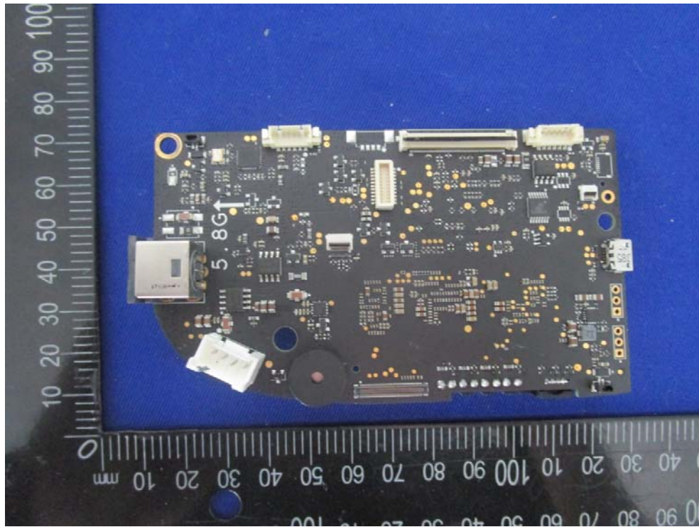
EUT – Pcb3 Uncover3 View
