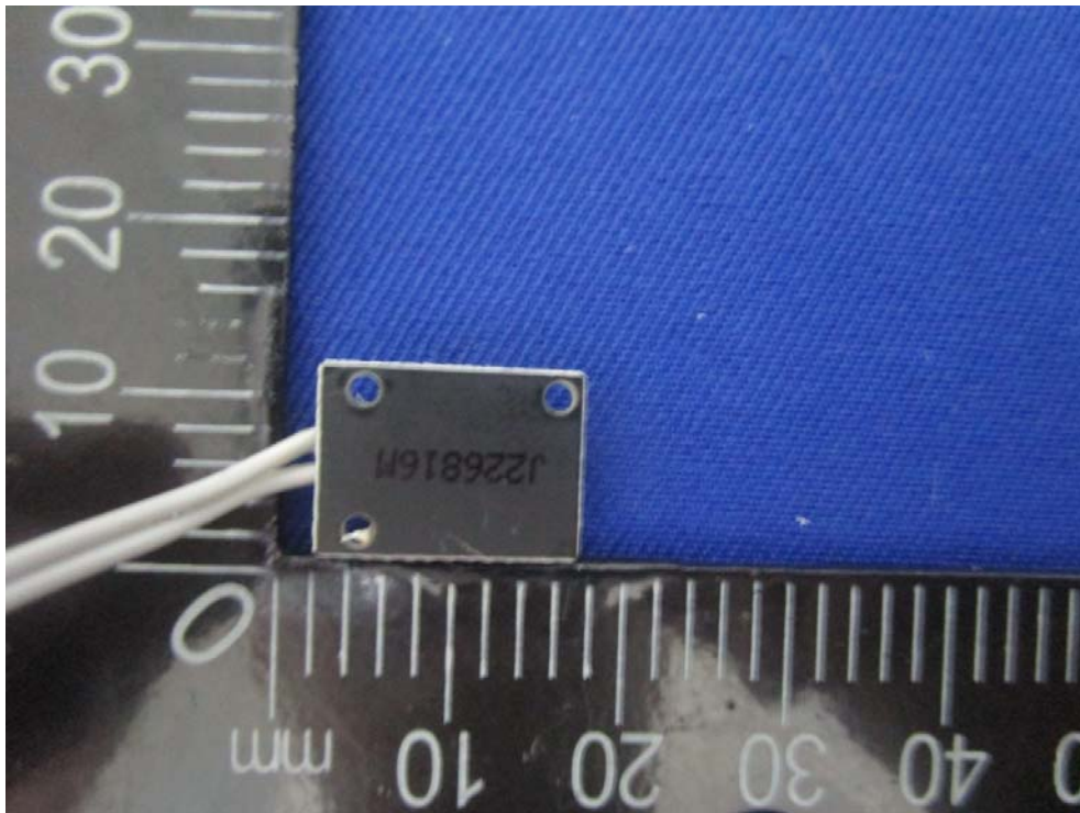
EUT – Pcb9 Bottom View
