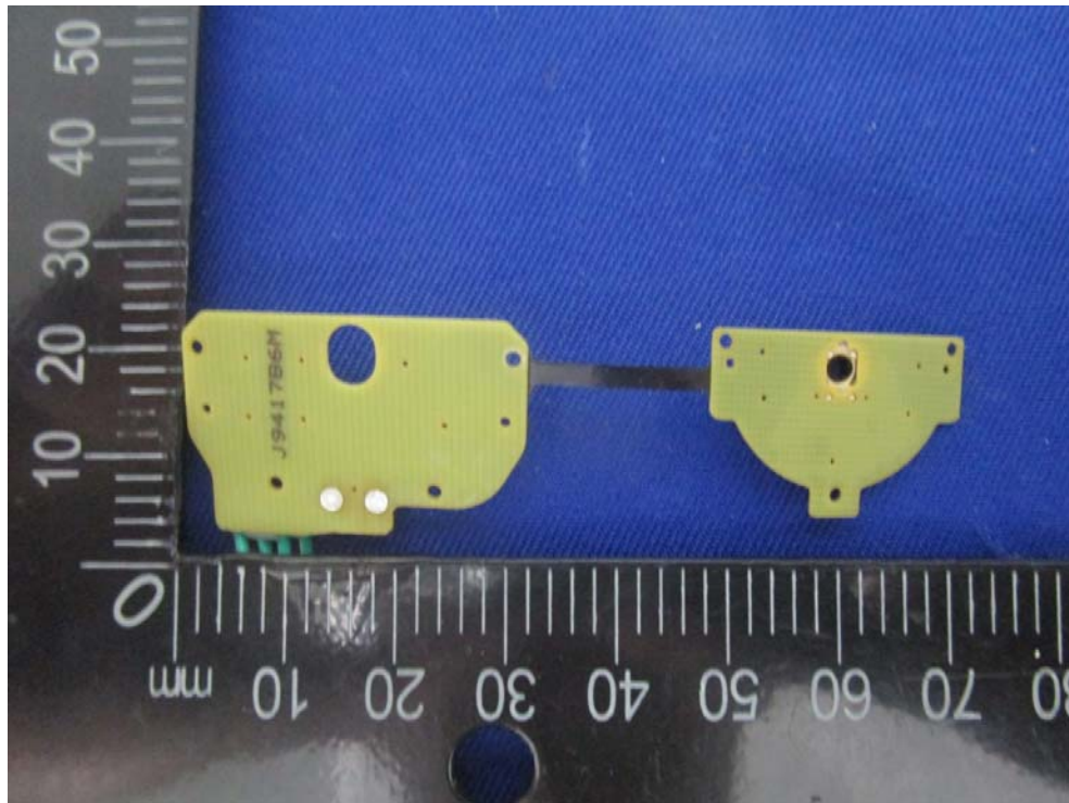
EUT – Pcb6 Bottom View
