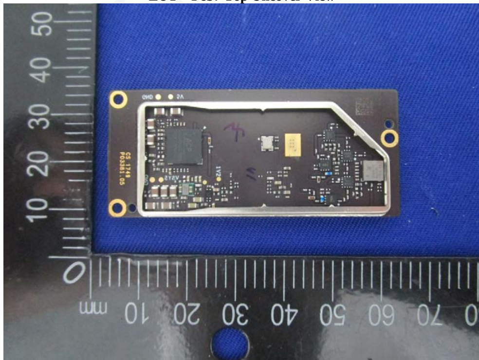
EUT – Pcb7 Top Uncover View
