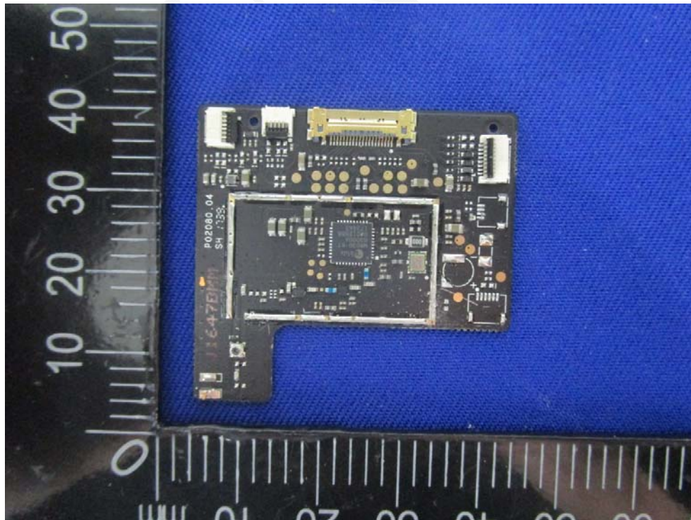
EUT – GPS Uncover View
