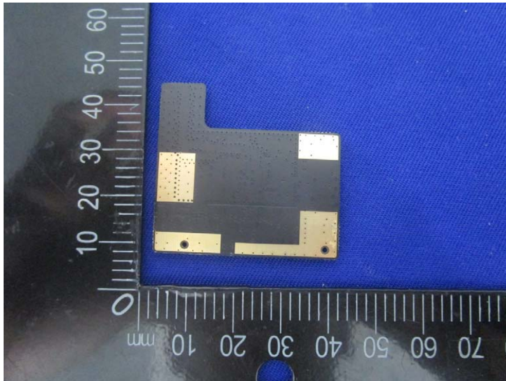
EUT – GPS Bottom View
