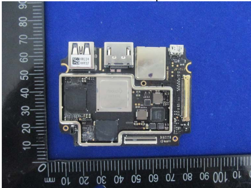
EUT – Pcb1 Uncover1 Top View
