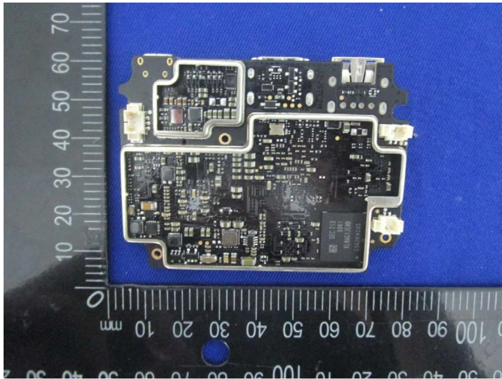
EUT – Pcb1 Uncover Bottom View
