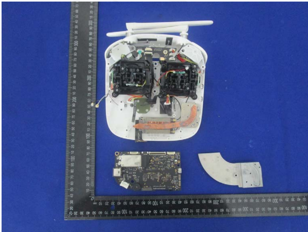
EUT – Uncover6 View
