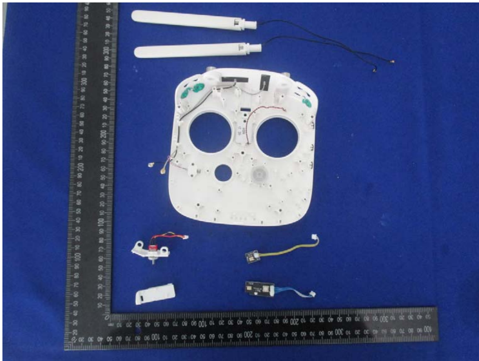
EUT – Uncover8 View
