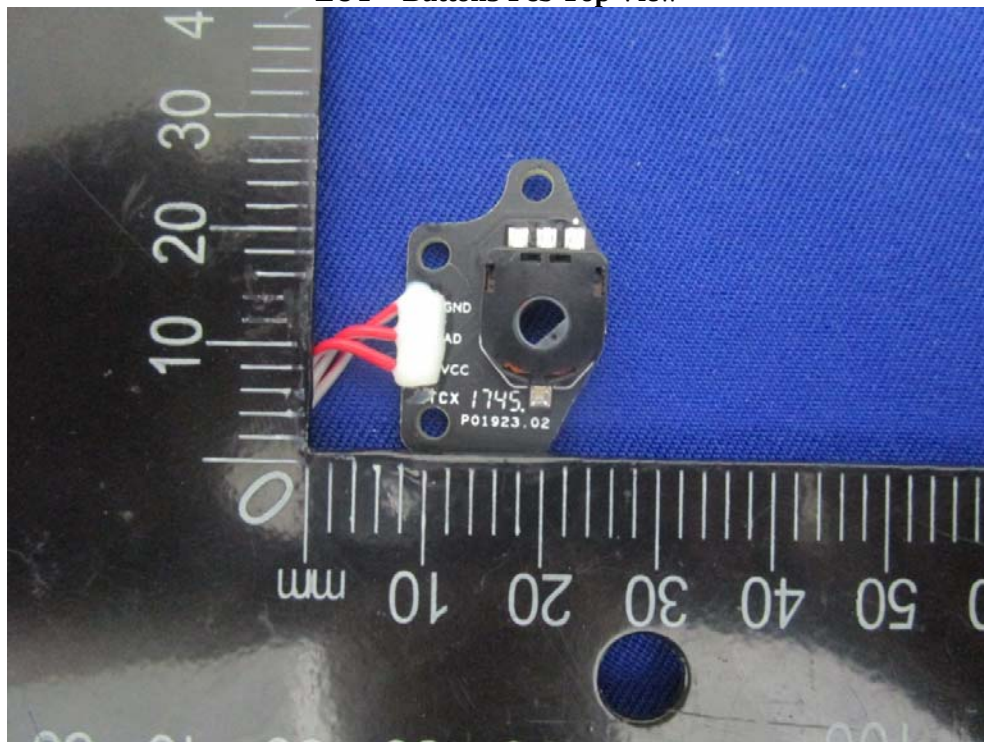
EUT – Button3 Pcb Top View
