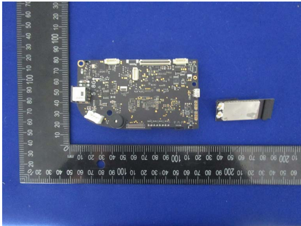
EUT – Pcb3 Uncover1 View
