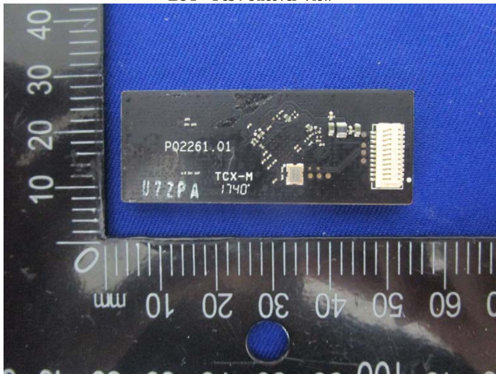
EUT – Pcb4 Uncover View
