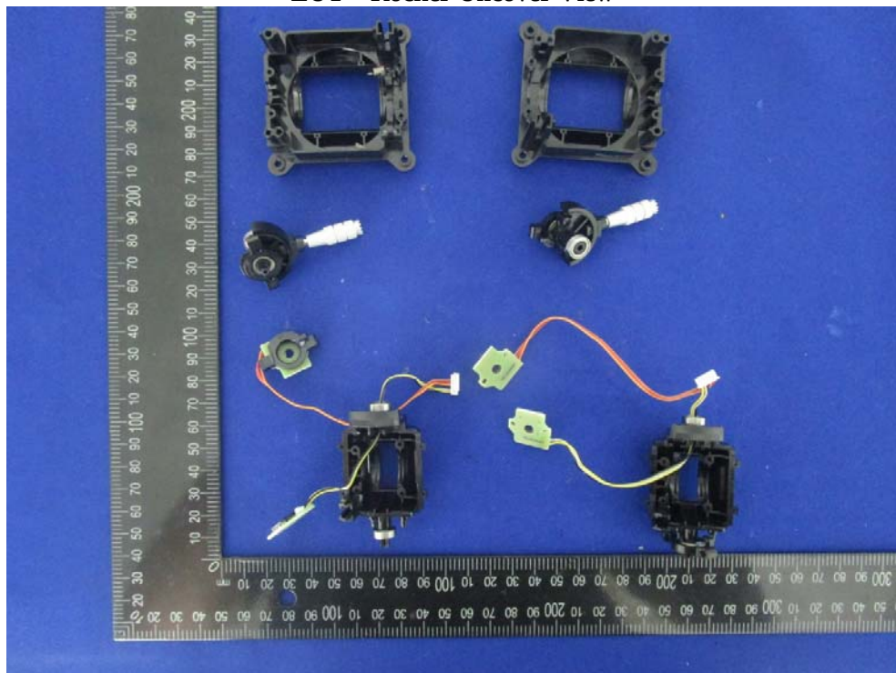
EUT – Rocker Uncover View
