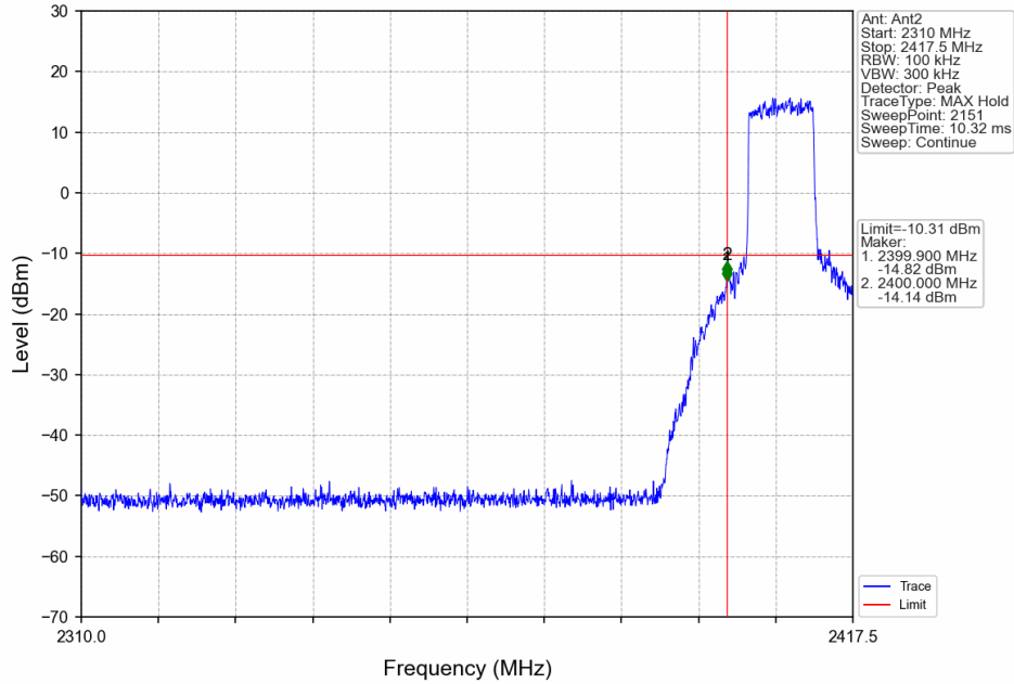
10M_LCH_2407.5MHz_Ant2_NTNV
