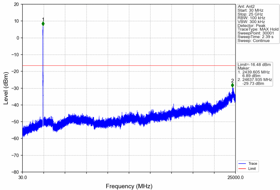
40M_LCH_2422.5MHz_Ant2_NTNV
