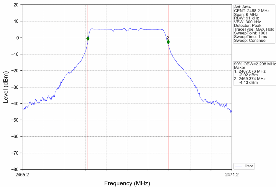
3M_HCH_2468.2MHz_Ant4_NTNV
