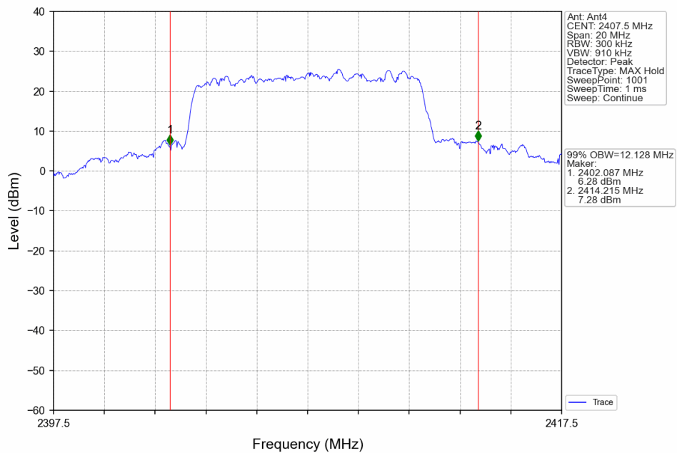
10M_LCH_2407.5MHz_Ant4_NTNV
