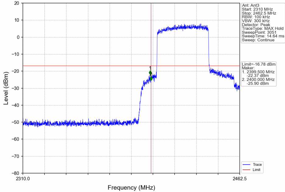
40M_LCH_2422.5MHz_Ant3_NTNV
