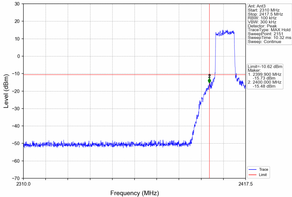
10M_LCH_2407.5MHz_Ant3_NTNV
