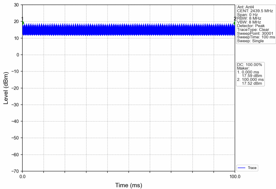
5M_MCH_2439.5MHz_Ant4_NTNV
