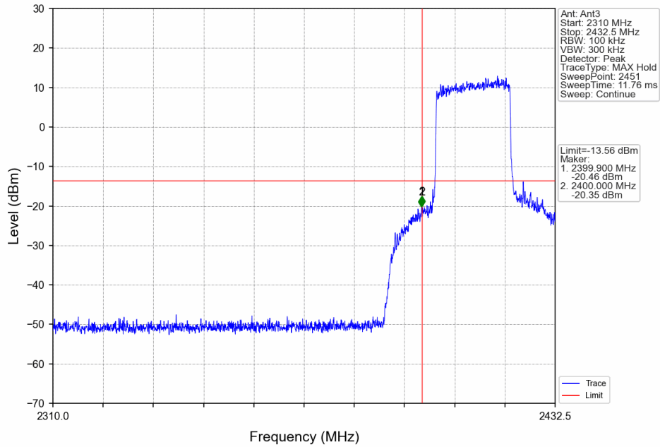
20M_LCH_2412.5MHz_Ant3_NTNV
