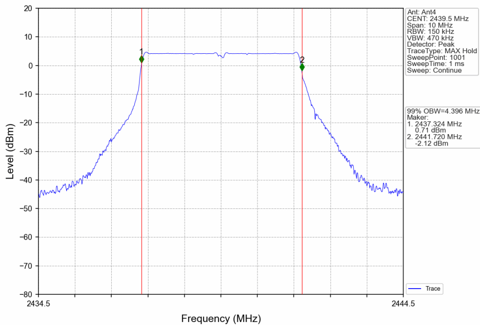
5M_MCH_2439.5MHz_Ant4_NTNV
