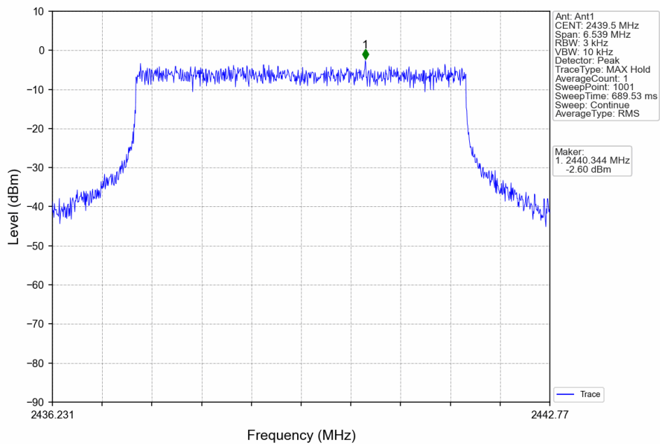
5M_MCH_2439.5MHz_Ant1_NTNV
