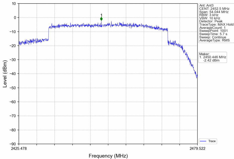
40M_HCH_2452.5MHz_Ant3_NTNV
