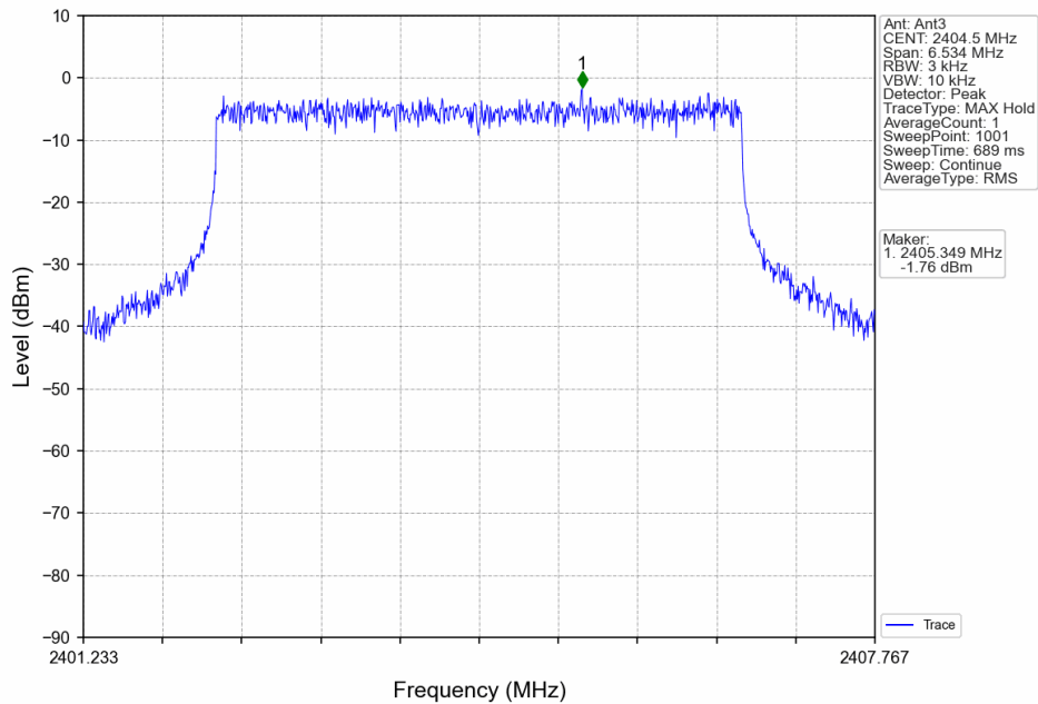
5M_LCH_2404.5MHz_Ant3_NTNV
