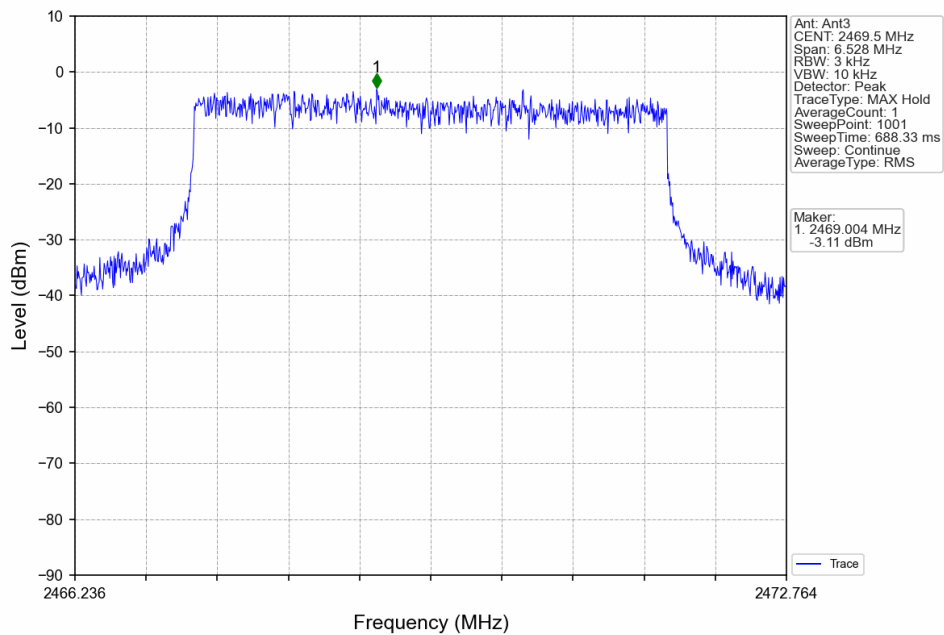
5M_HCH_2469.5MHz_Ant3_NTNV
