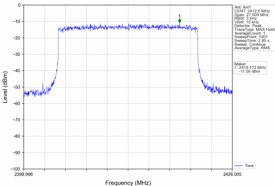
20M_LCH_2412.5MHz_Ant1_NTNV
