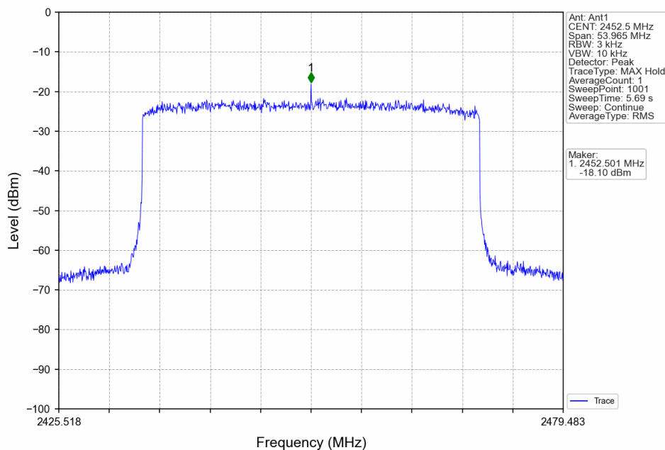
40M_HCH_2452.5MHz_Ant1_NTNV
