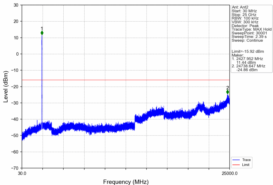
60M_LCH_2432.5MHz_Ant2_NTNV
