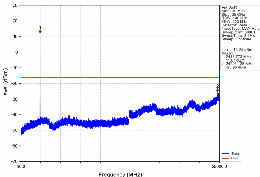
60M_HCH_2442.5MHz_Ant3_NTNV
