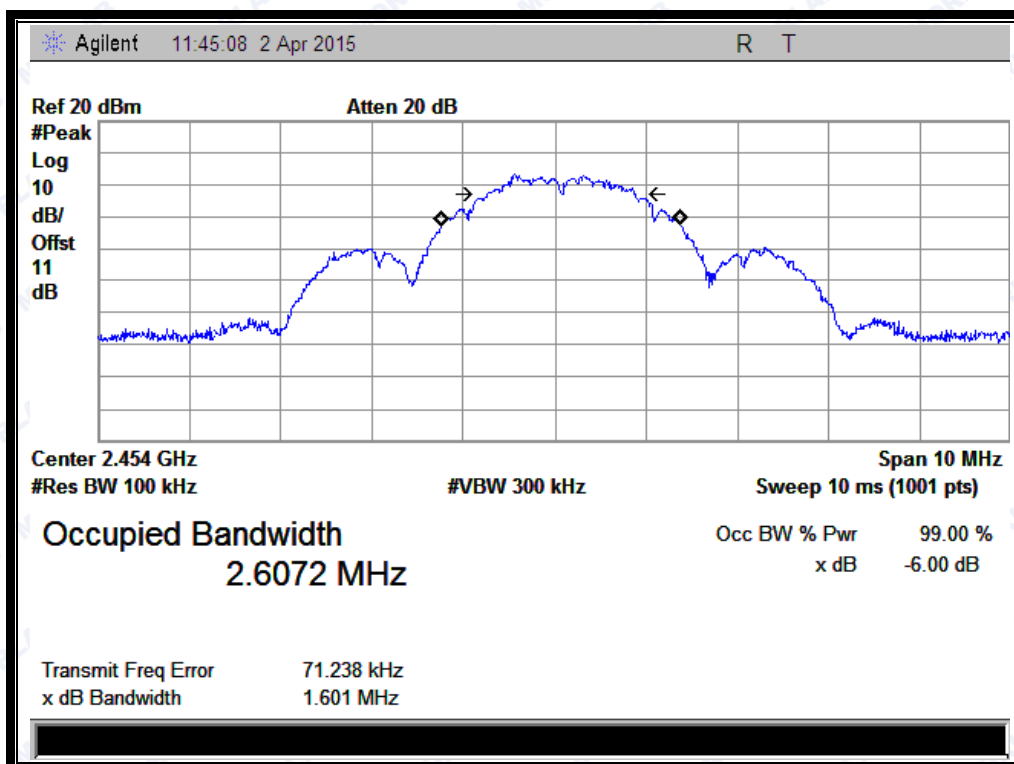
(Plot C: Channel 39: 2454MHz)
