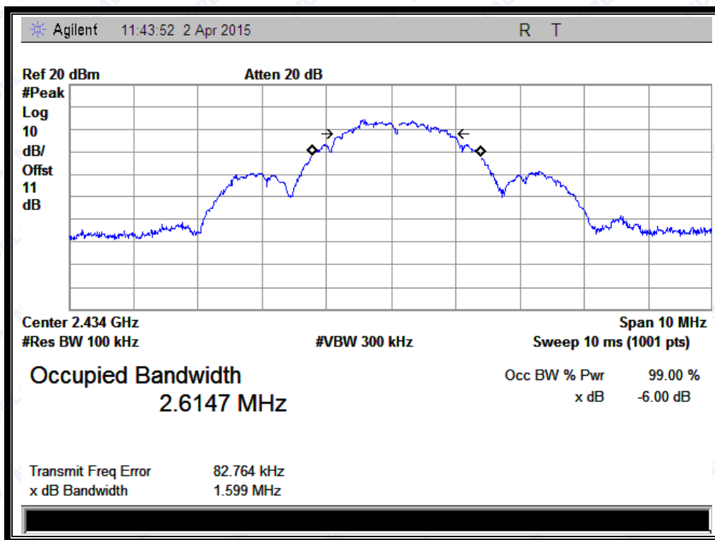
(Plot B: Channel 19: 2434 MHz)
