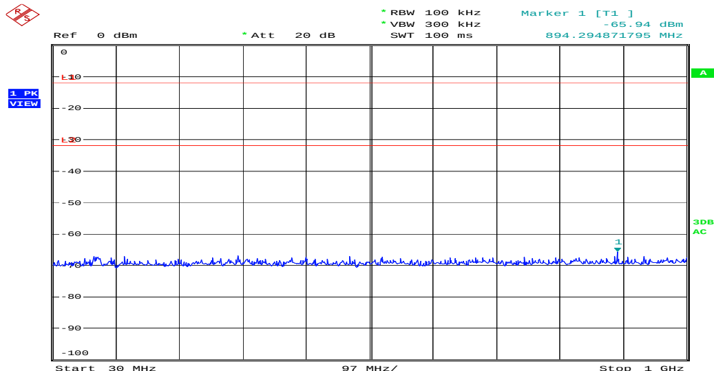
Figure 23: Spurious Emission from 30MHz to 1GHz, Mode A (2412MHz)
