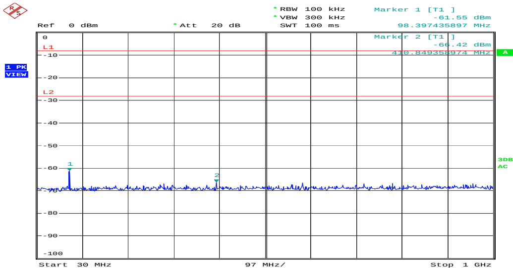
Figure 8: Spurious Emission from 30MHz to 1GHz, Mode A (2412MHz)
