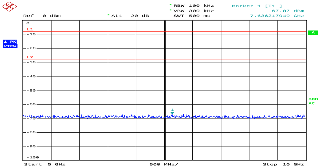
Figure 10: Spurious Emission from 5 to 10GHz, Mode A (2412MHz)
