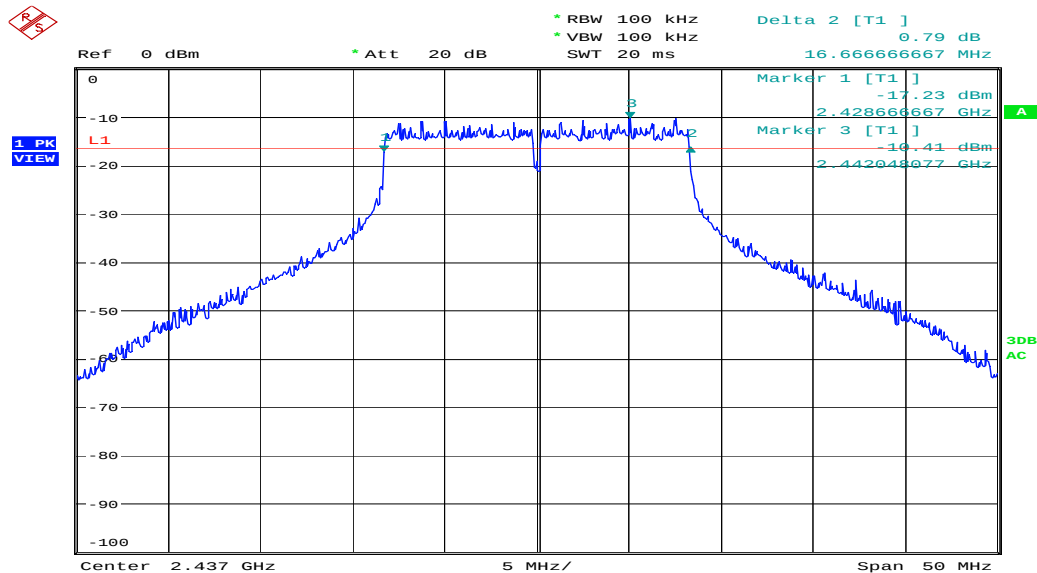
Figure 6: 6dB Bandwidth, Mode B (2437MHz)
