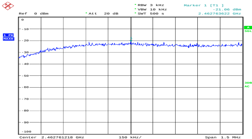
Figure 40: Power Spectral Density, Mode C (2462MHz), 802.11.b
