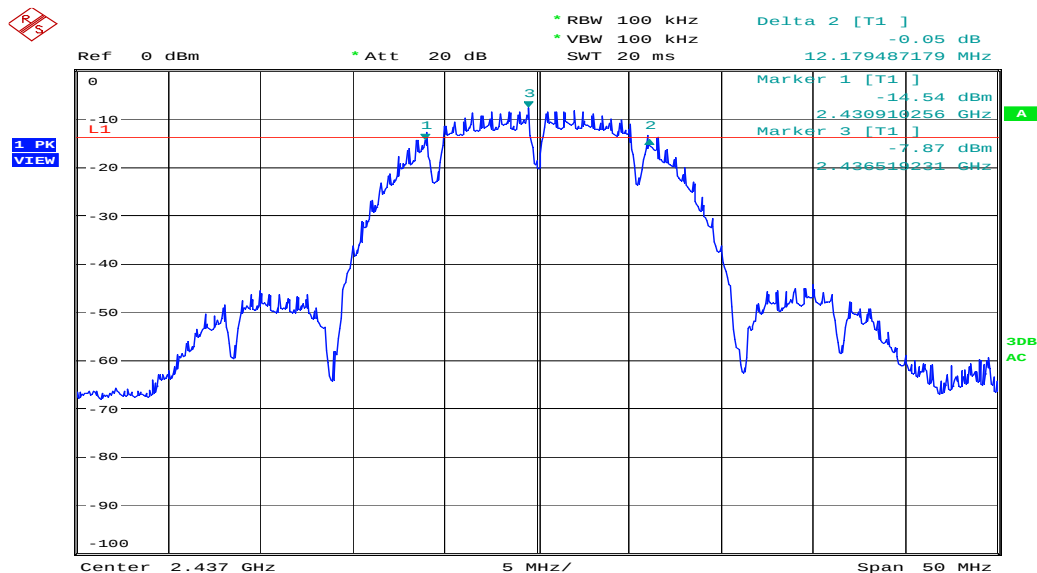
Figure 3: 6dB Bandwidth, Mode B (2437MHz)
