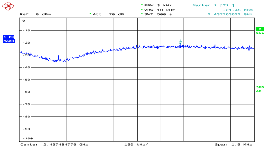
Figure 39: Power Spectral Density, Mode B (2437MHz), 802.11.b
