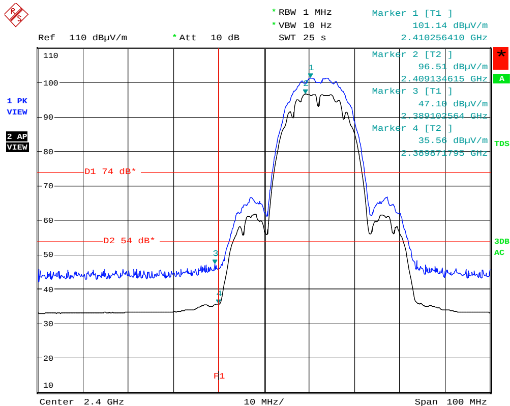
Figure 44: Band Edge Radiated Emission, Mode A (2412MHz), Peak and Average
