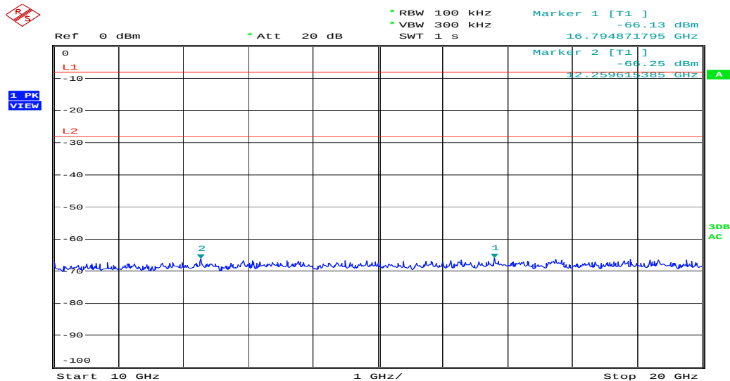
Figure 16: Spurious Emission from 10 to 20GHz, Mode B (2437MHz)
