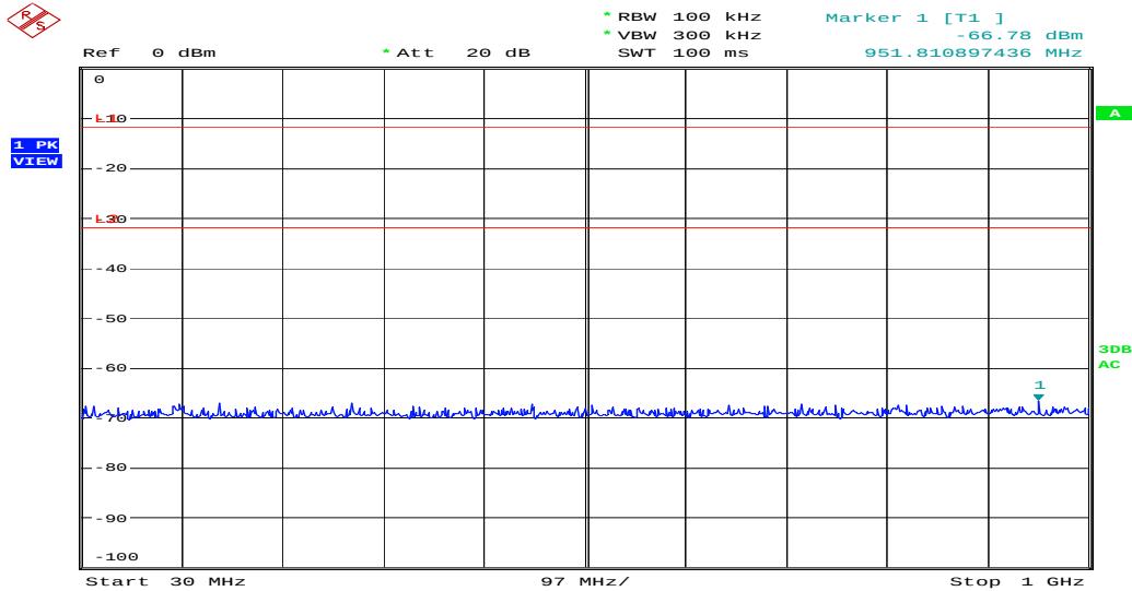
Figure 28: Spurious Emission from 30MHz to 1GHz, Mode B (2437MHz)
