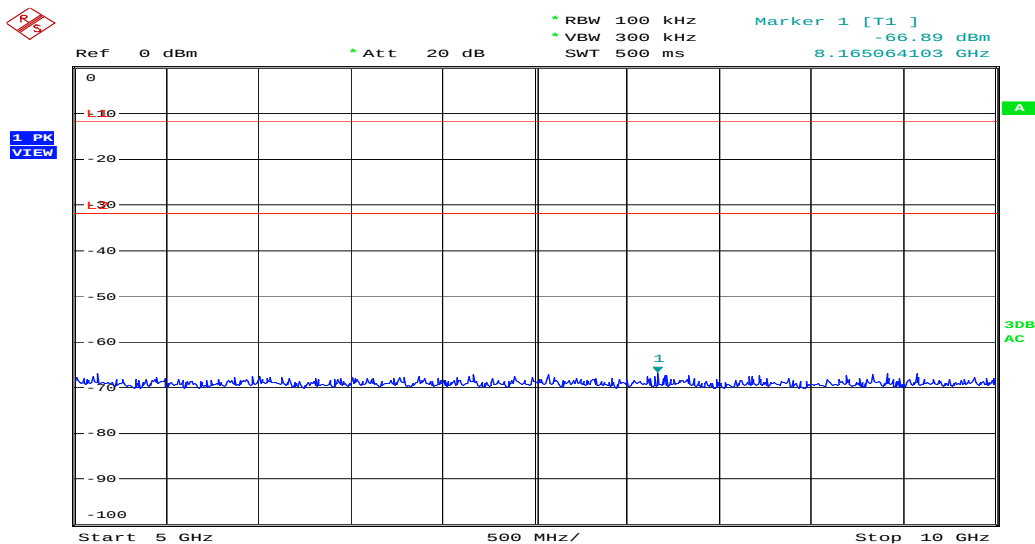
Figure 30: Spurious Emission from 5 to 10GHz, Mode B (2437MHz)
