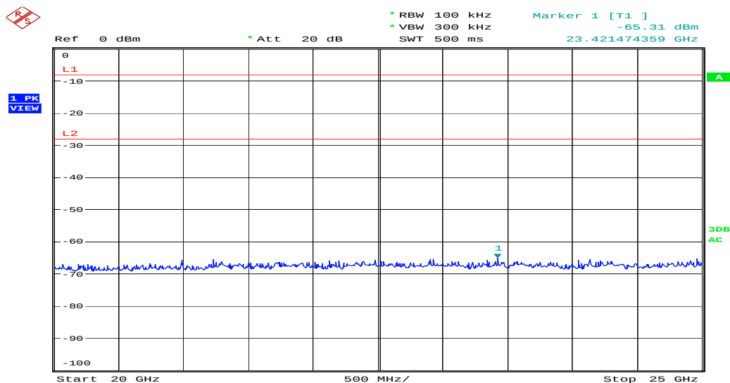
Figure 17: Spurious Emission from 20 to 25GHz, Mode B (2437MHz)
