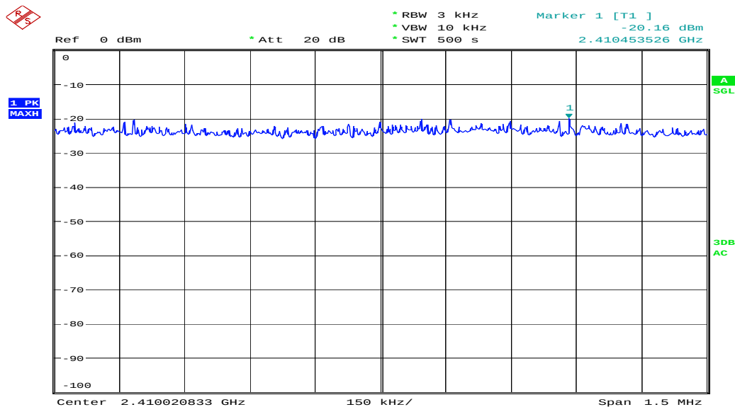
Figure 38: Power Spectral Density, Mode A (2412MHz), 802.11.b
