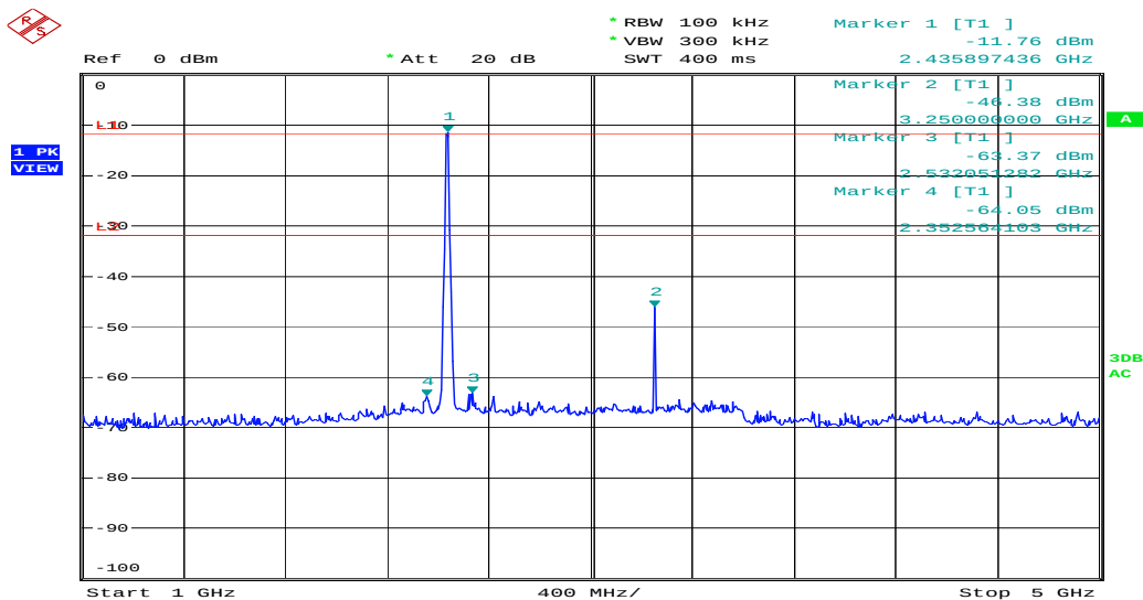
Figure 29: Spurious Emission from 1 to 5GHz, Mode B (2437MHz)
