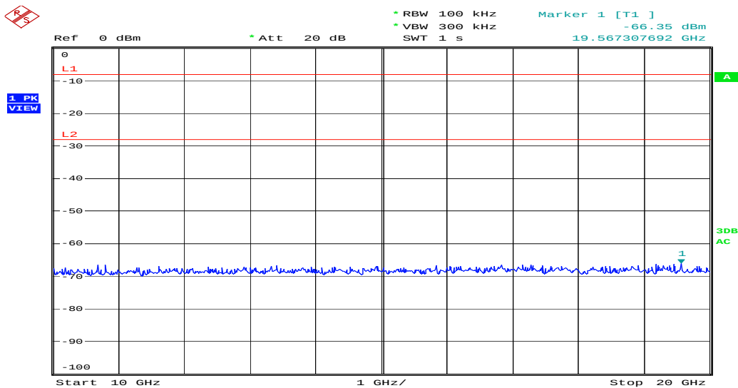
Figure 11: Spurious Emission from 10 to 20GHz, Mode A (2412MHz)
