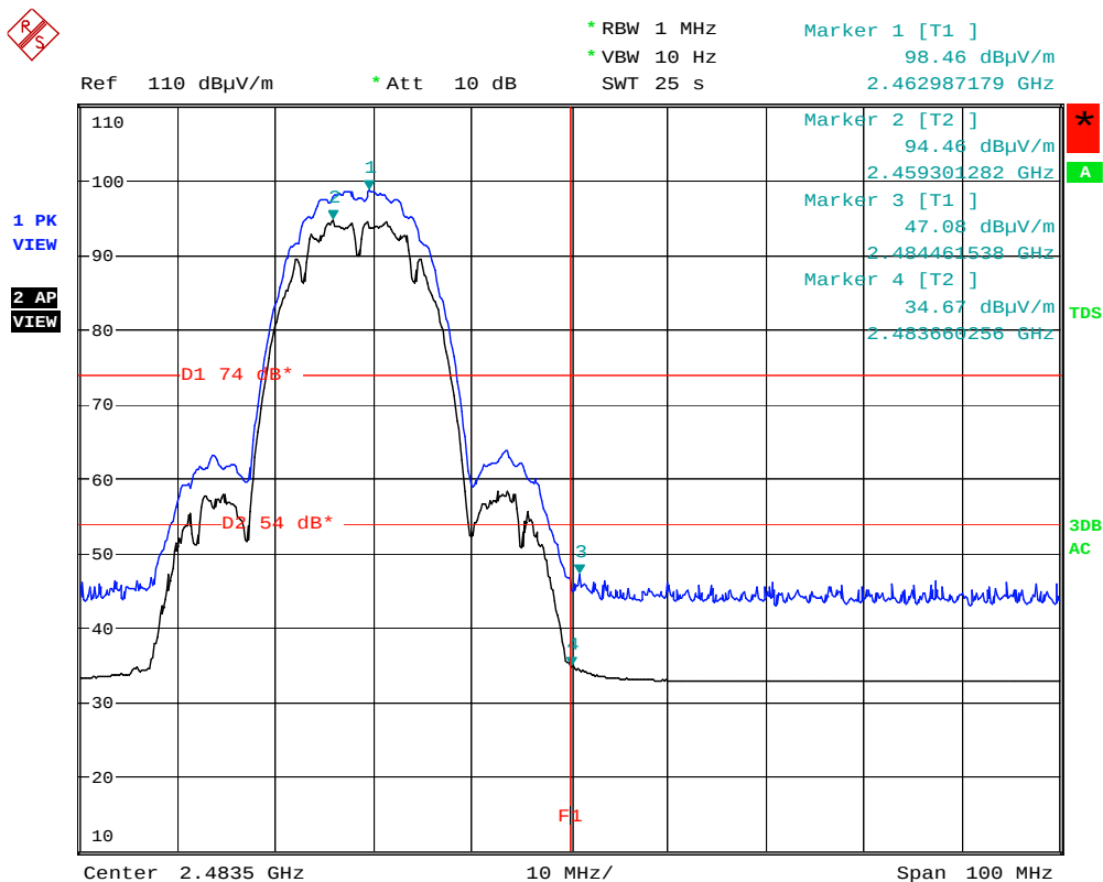
Figure 45: Band Edge Radiated Emission, Mode C (2462MHz), Peak and Average
