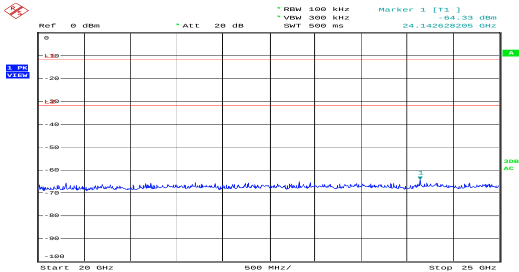
Figure 32: Spurious Emission from 20 to 25GHz, Mode B (2437MHz)
