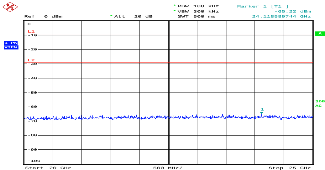
Figure 22: Spurious Emission from 20 to 25GHz, Mode C (2462MHz)
