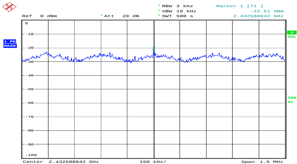
Figure 42: Power Spectral Density, Mode B (2437MHz), 802.11.g
