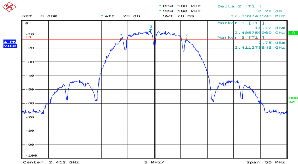
Figure 2: 6dB Bandwidth, Mode A (2412MHz)
