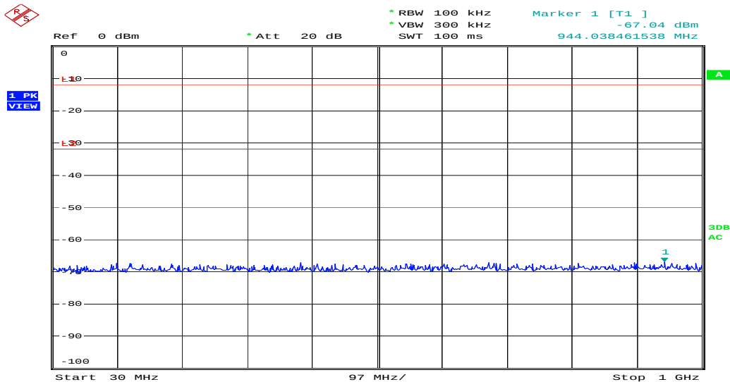
Figure 33: Spurious Emission from 30MHz to 1GHz, Mode C (2462MHz)
