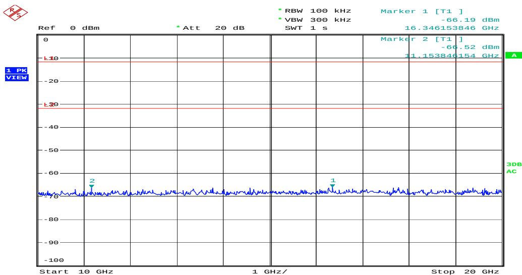
Figure 31: Spurious Emission from 10 to 20GHz, Mode B (2437MHz)
