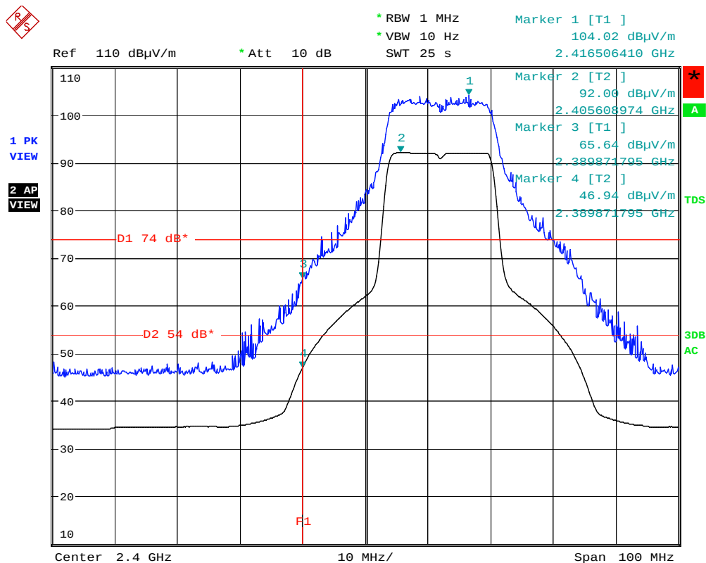
Figure 46: Band Edge Radiated Emission, Mode A (2412MHz), Peak and Average
