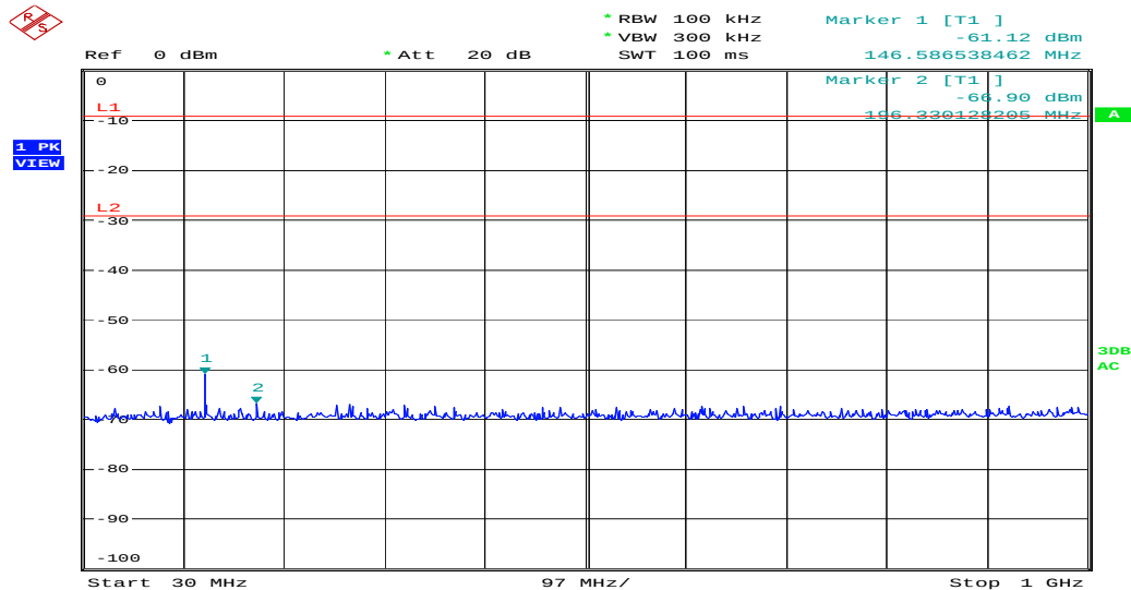
Figure 18: Spurious Emission from 30MHz to 1GHz, Mode C (2462MHz)
