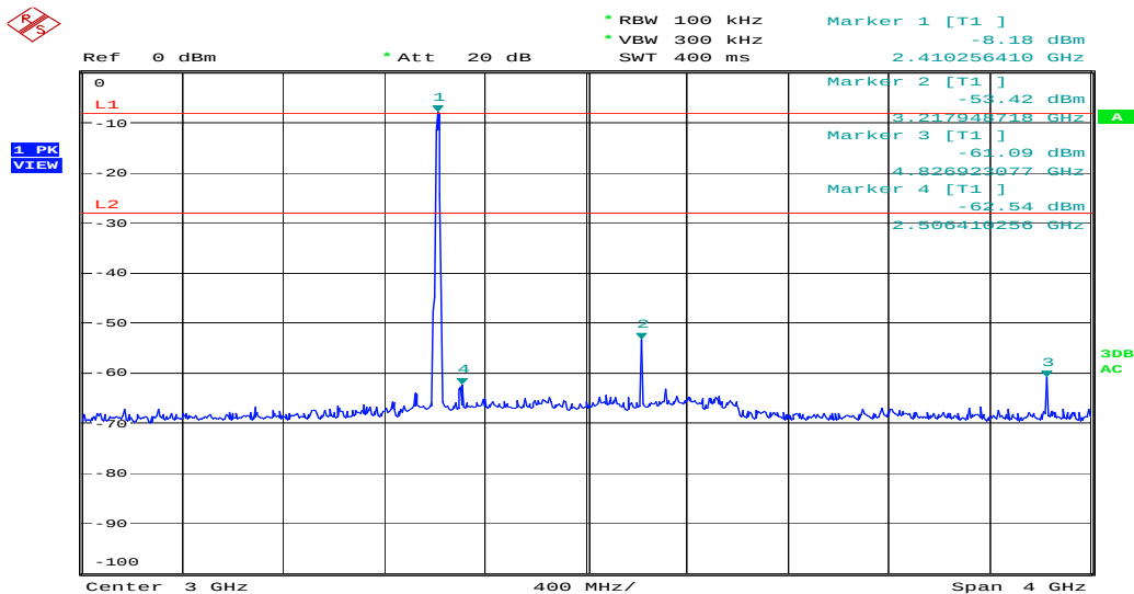
Figure 9: Spurious Emission from 1 to 5GHz, Mode A (2412MHz)
