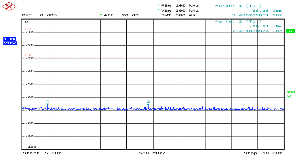
Figure 20: Spurious Emission from 5 to 10GHz, Mode C (2462MHz)
