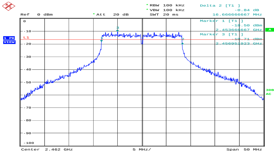
Figure 7: 6dB Bandwidth, Mode C (2462MHz)
