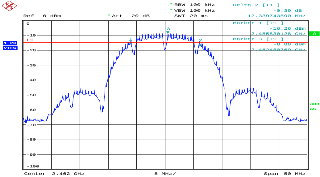
Figure 4: 6dB Bandwidth, Mode C (2462MHz)
