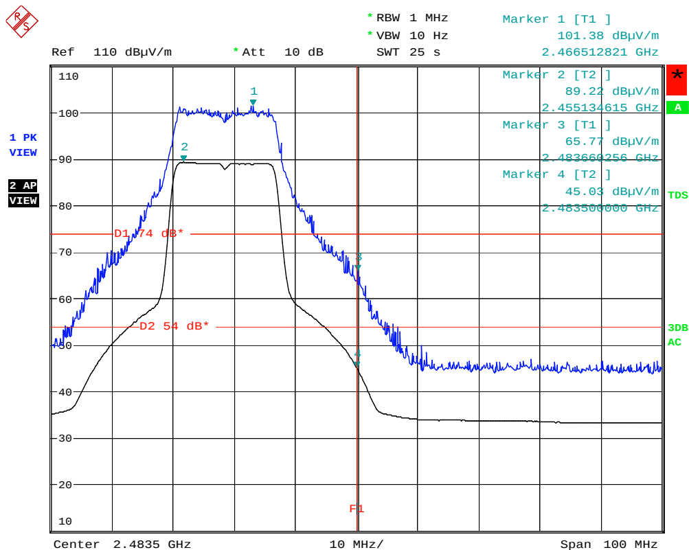
Figure 47: Band Edge Radiated Emission, Mode C (2462MHz), Peak and Average
