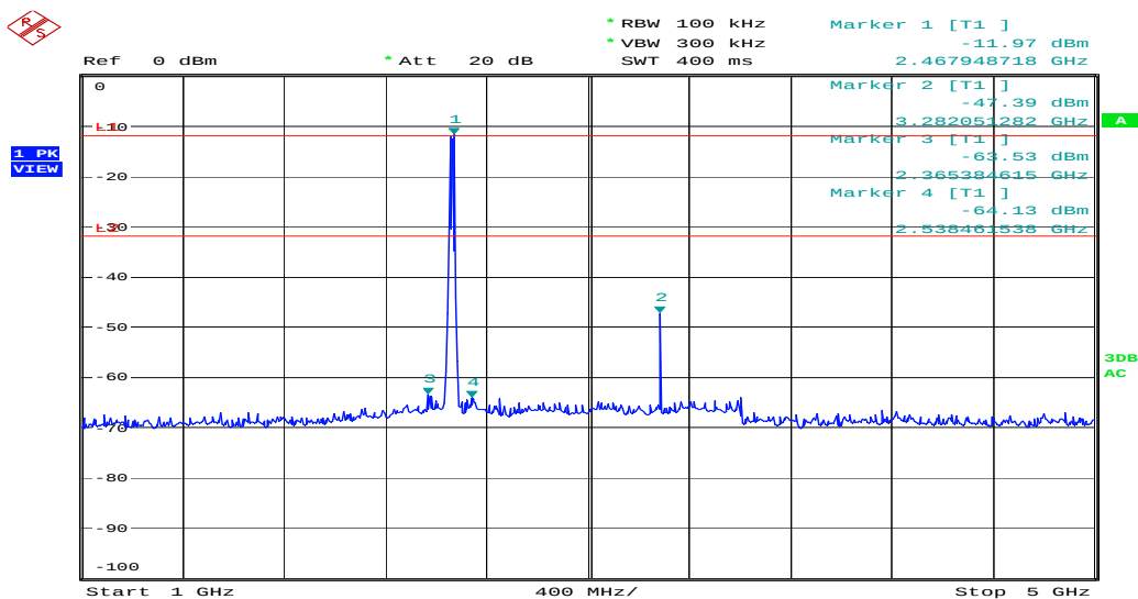
Figure 34: Spurious Emission from 1 to 5GHz, Mode C (2462MHz)
