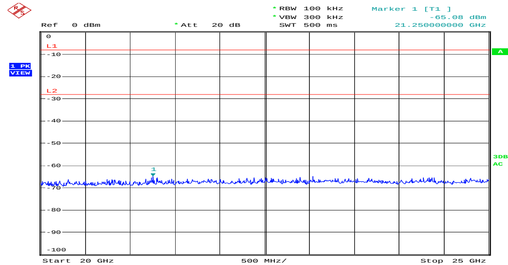
Figure 12: Spurious Emission from 20 to 25GHz, Mode A (2412MHz)
