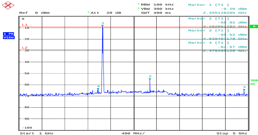
Figure 19: Spurious Emission from 1 to 5GHz, Mode C (2462MHz)
