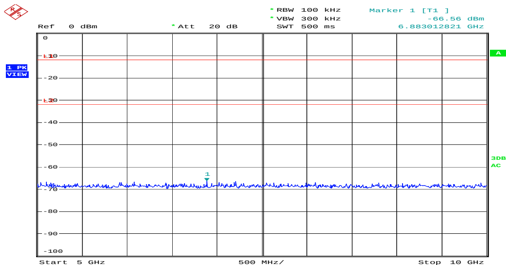
Figure 25: Spurious Emission from 5 to 10GHz, Mode A (2412MHz)
