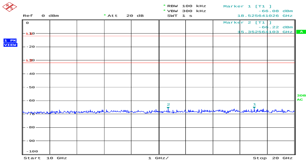
Figure 26: Spurious Emission from 10 to 20GHz, Mode A (2412MHz)
