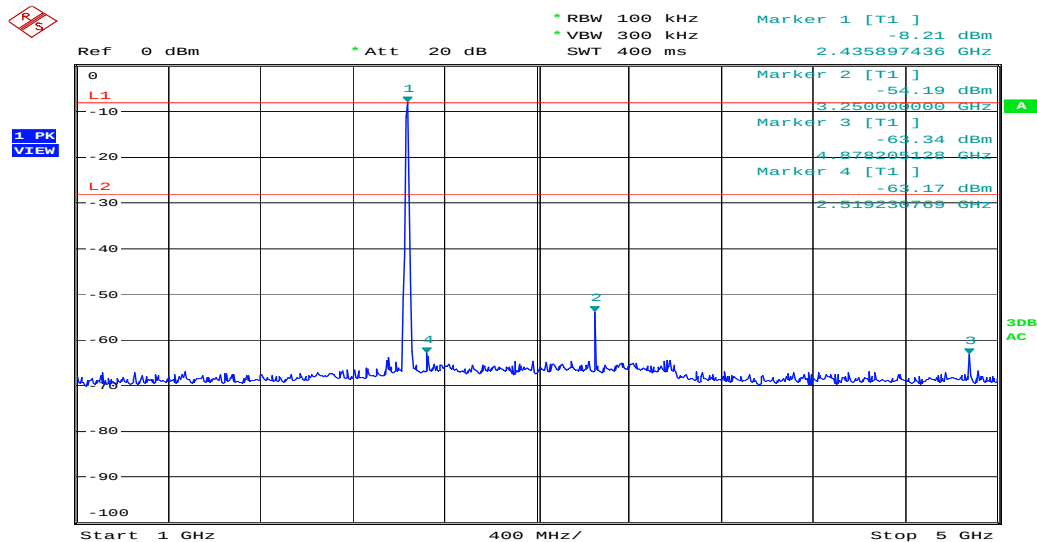
Figure 14: Spurious Emission from 1 to 5GHz, Mode B (2437MHz)
