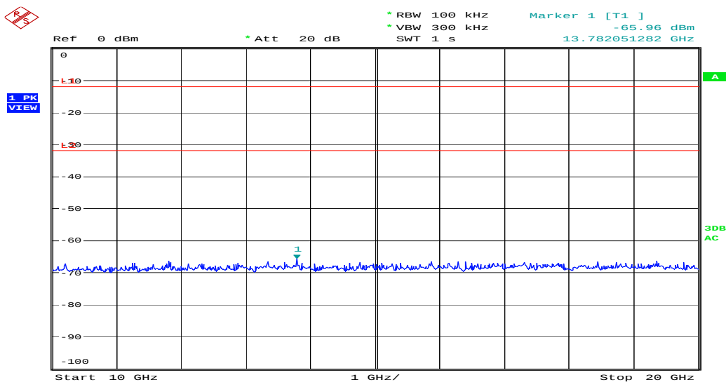
Figure 36: Spurious Emission from 10 to 20GHz, Mode C (2462MHz)
