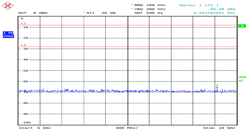
Figure 15: Spurious Emission from 5 to 10GHz, Mode B (2437MHz)
