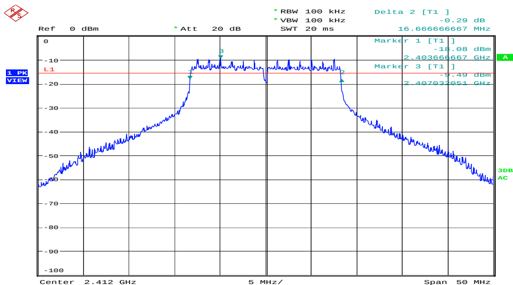
Figure 5: 6dB Bandwidth, Mode A (2412MHz)
