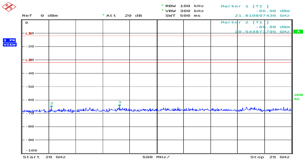
Figure 37: Spurious Emission from 20 to 25GHz, Mode C (2462MHz)
