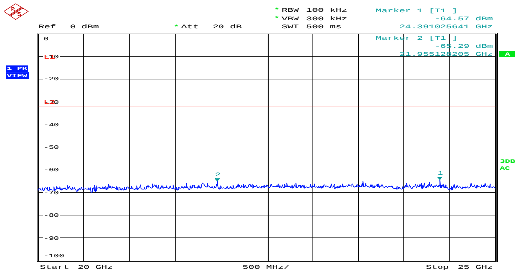
Figure 27: Spurious Emission from 20 to 25GHz, Mode A (2412MHz)
