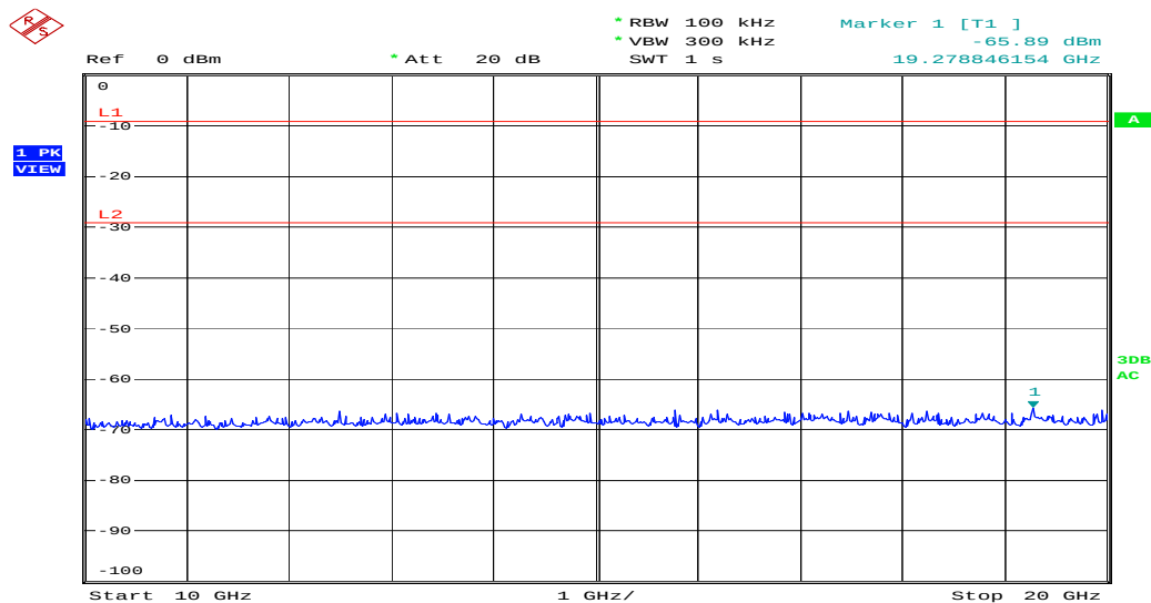
Figure 21: Spurious Emission from 10 to 20GHz, Mode C (2462MHz)
