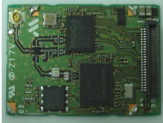
Module without shielding (Top view)
