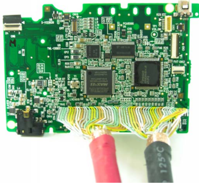
Bottom View control PCB
