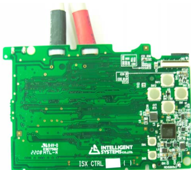
Bottom View CPU board
