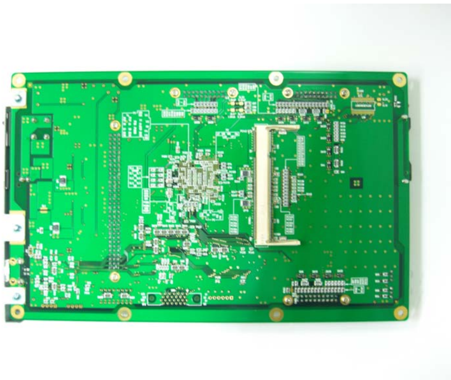
Bottom View Power Board
