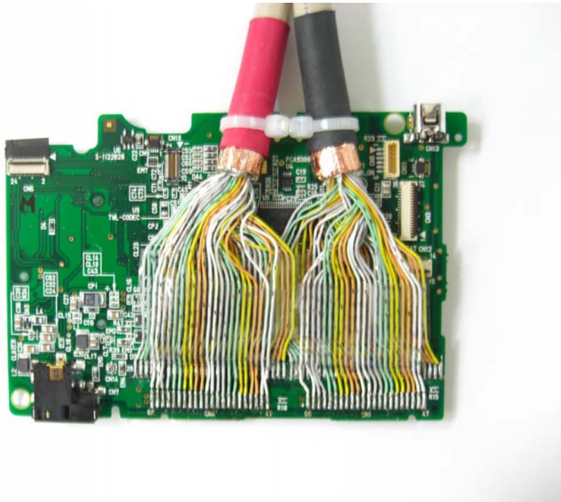
Bottom View control PCB 2 nd picture
