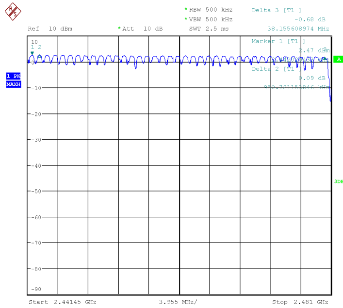
Fig.93 Number of hopping frequency: 8DPSK, Ch40~78
