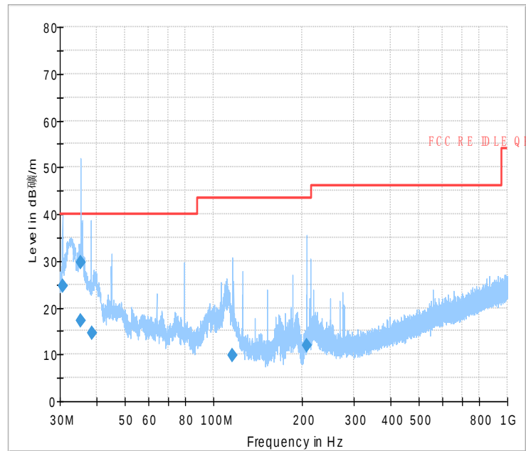
Fig.52 Radiated emission: 8DPSK, Ch0, 30MHz~1GHz
