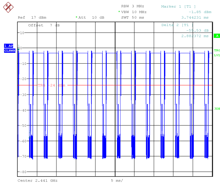
Fig.68 Time of occupancy (Dwell Time): Ch39,Packet 2-DH5
