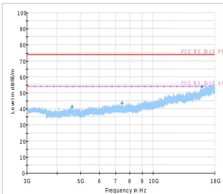
Fig.48 Radiated emission: \pi/4 DQPSK, Ch0, 3GHz~18GHz
