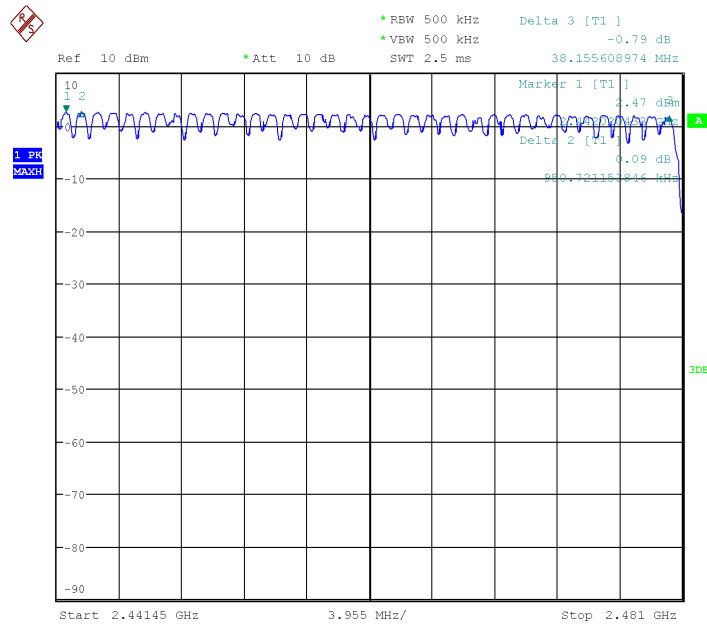
Fig.91 Number of hopping frequency: \pi/4 DQPSK, Ch40~78
