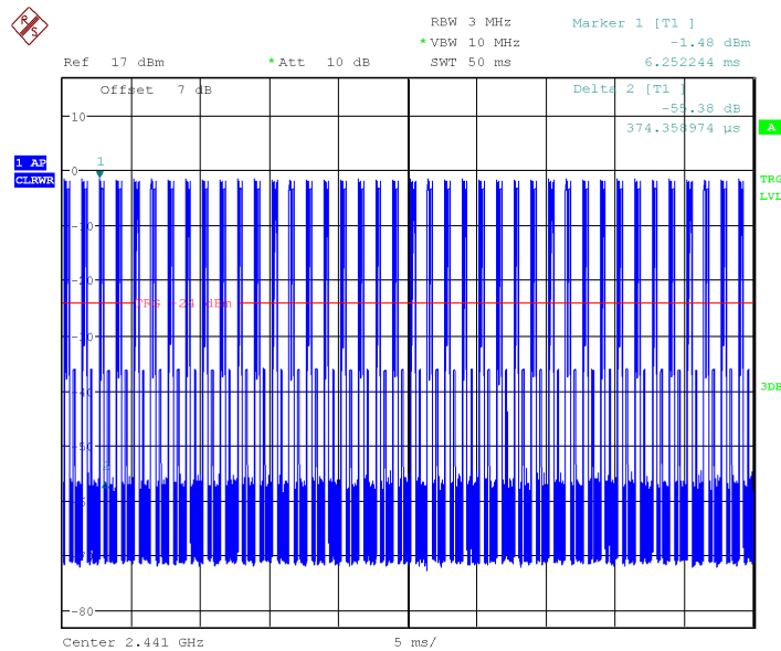
Fig.64 Time of occupancy (Dwell Time): Ch39,Packet 2-DH1
