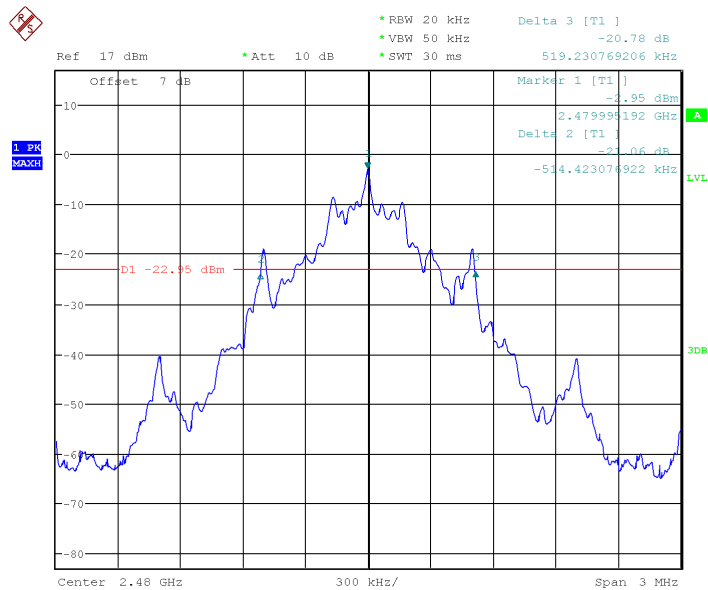
Fig.77 20dB Bandwidth: GFSK, Ch39
