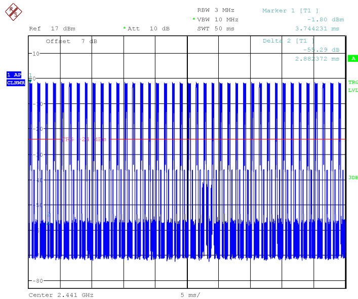
Fig.70 Time of occupancy (Dwell Time): Ch39,Packet 3-DH1
