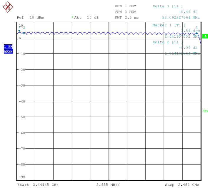
Fig.89 Number of hopping frequency: GFSK, Ch40~78
