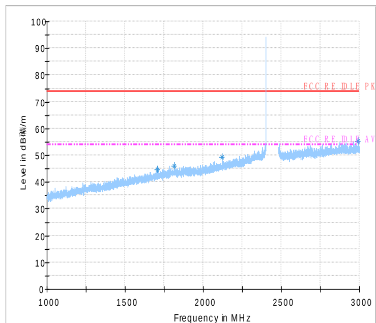
Fig.53 Radiated emission: 8DPSK, Ch0, 1GHz~3GHz
