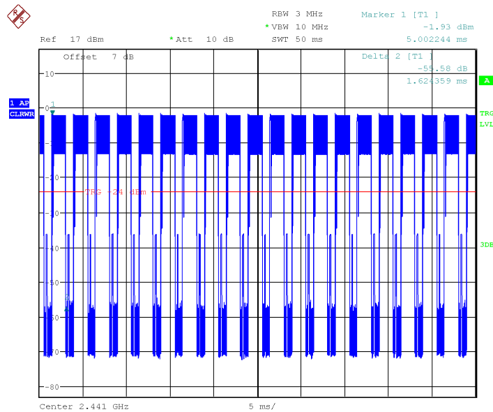
Fig.72 Time of occupancy (Dwell Time): Ch39,Packet 3-DH3
