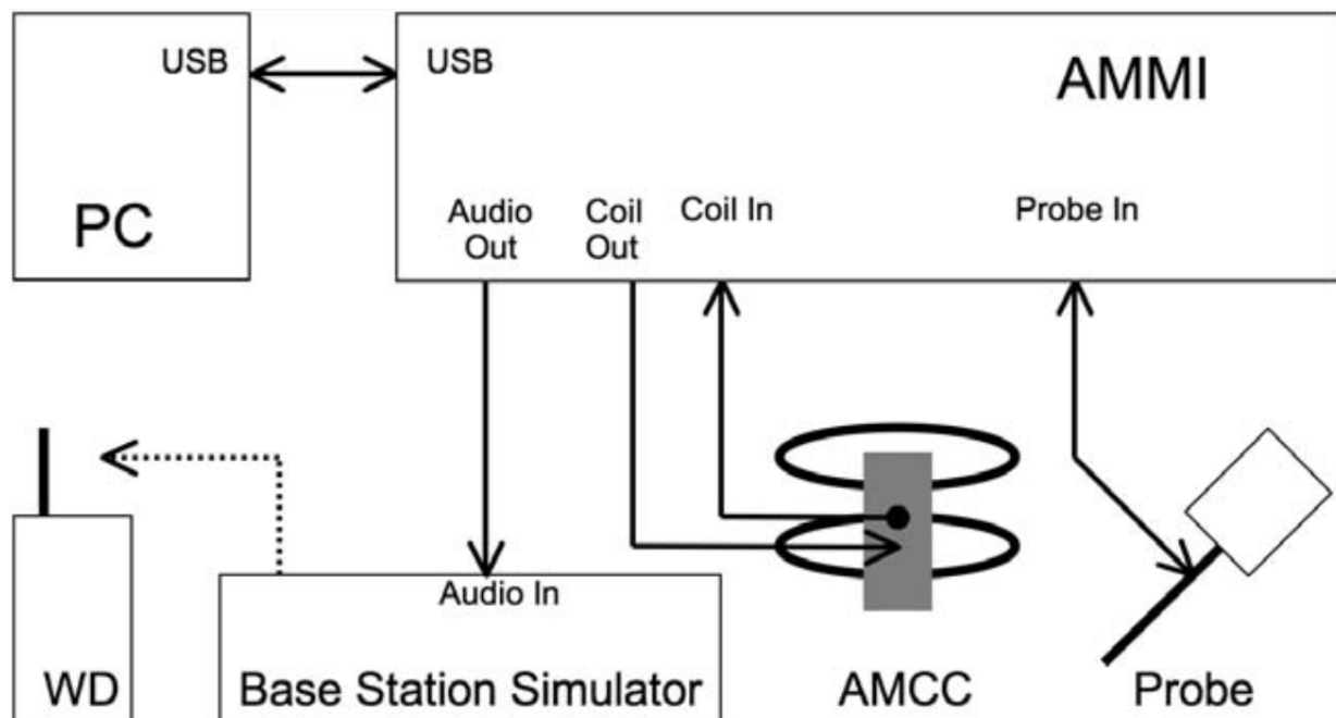
Fig. 5.5 T-Coil setup cabling
