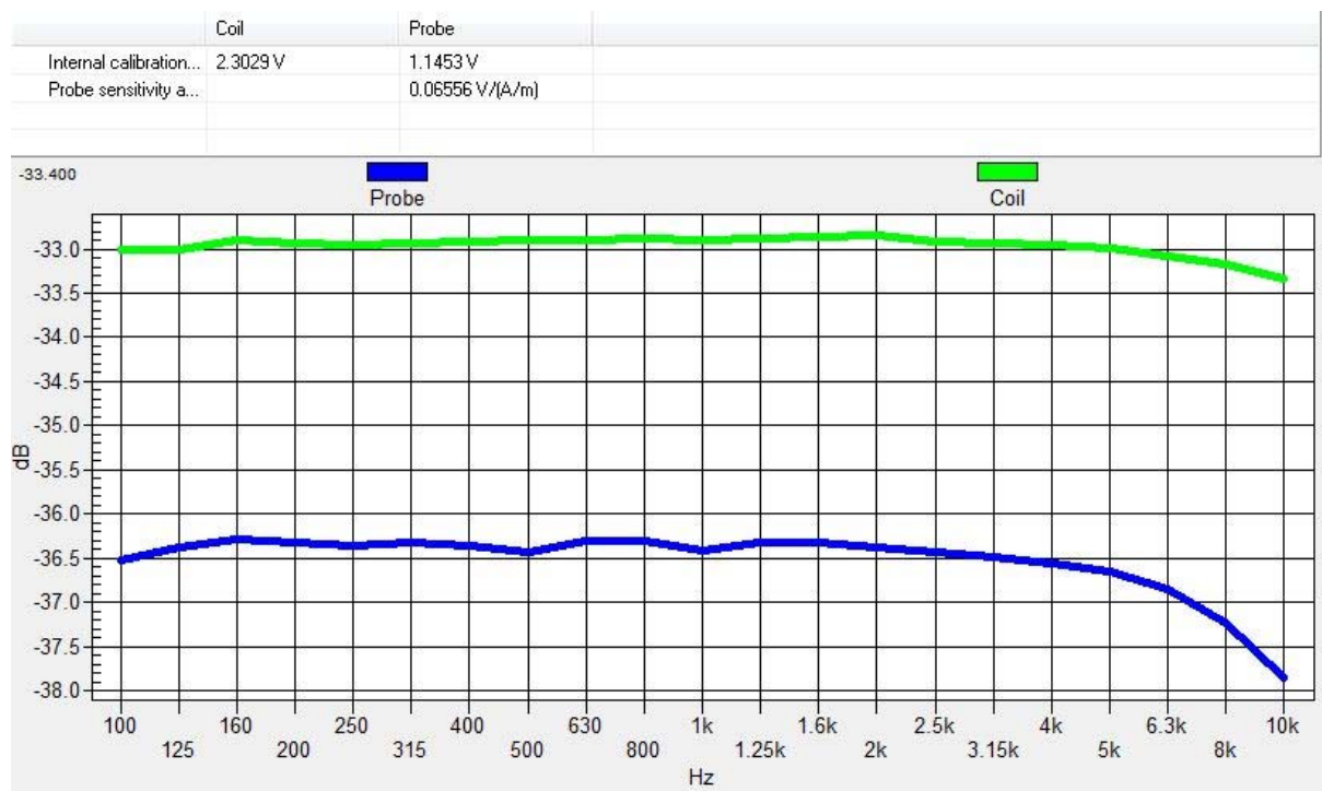
Fig. 5.3 The frequency response and sensitivity of AM1D probe
