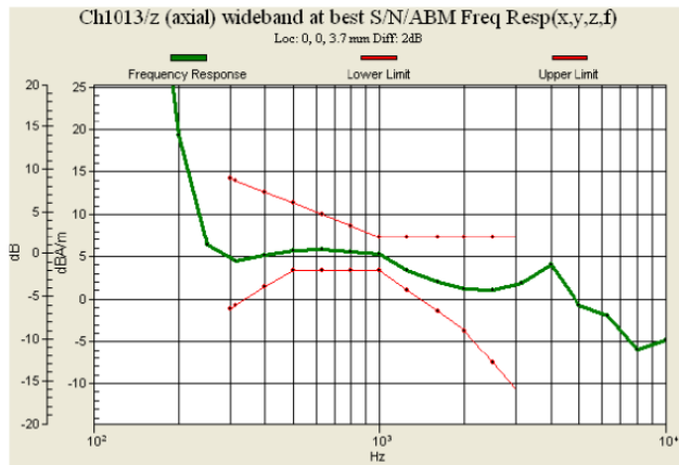
Fig 7.1 CDMA2000 BC0 Ch1013
