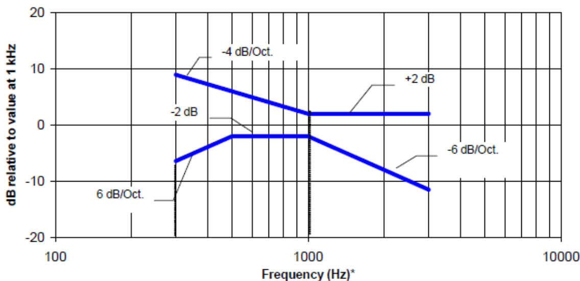
Fig. 4.1 Magnetic field frequency response for WDs with field strength \leq -15 dB at 1 KHz
