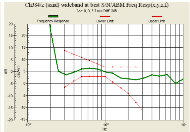
Fig 7.2 CDMA2000 BC0 Ch384
