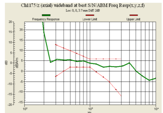
Fig 7.6 CDMA2000 BC1 Ch1175
