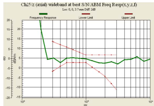
Fig 7.4 CDMA2000 BC1 Ch25
