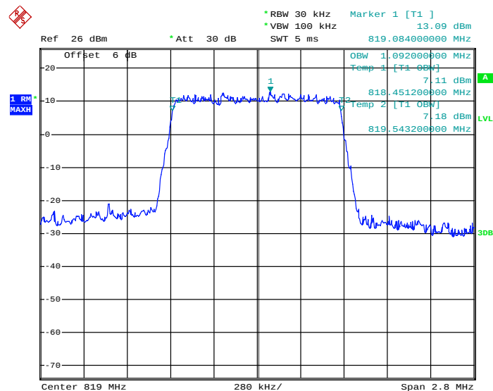
99% Occupied Bandwidth Plot on Channel 26740
