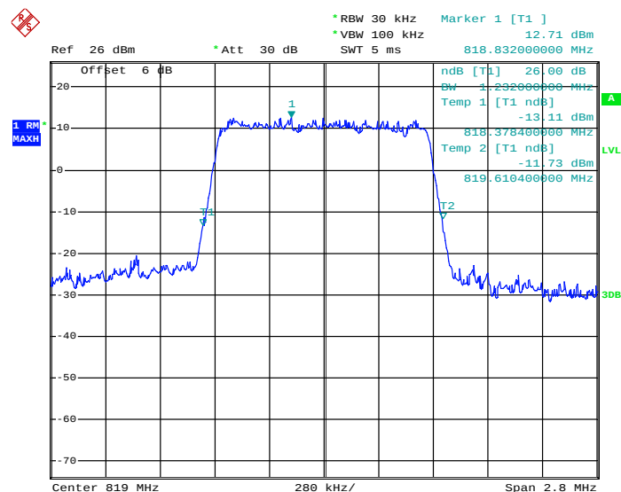
26dB Bandwidth Plot on Channel 26740
