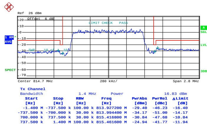
Lower Band Edge Plot for QPSK-RB Size 6, RB Offset 0
