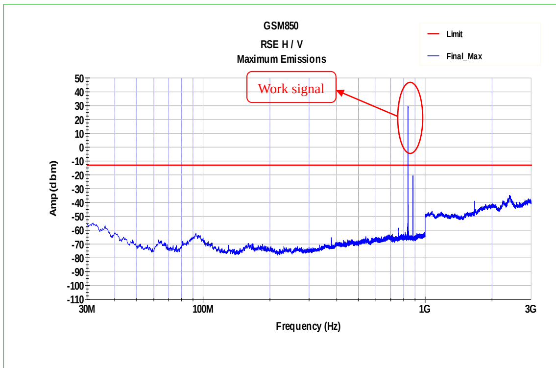
Fig.1 GSM850 on Channel 189 30MHz~3GHz
