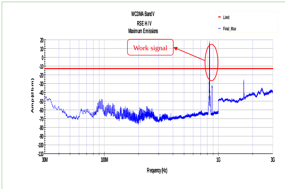
Fig.5 WCDMA Band V on Channel 4175 30MHz~3GHz
