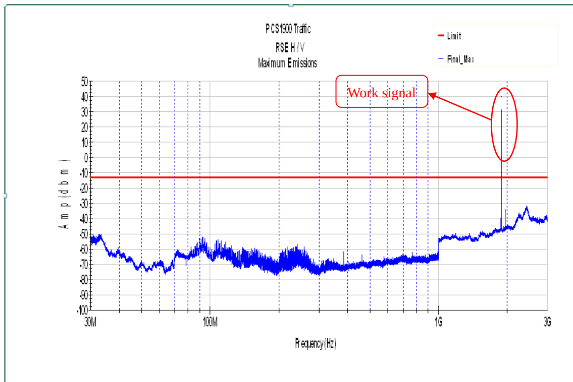
Fig.3 GSM1900 on Channel 661 30MHz~3GHz
