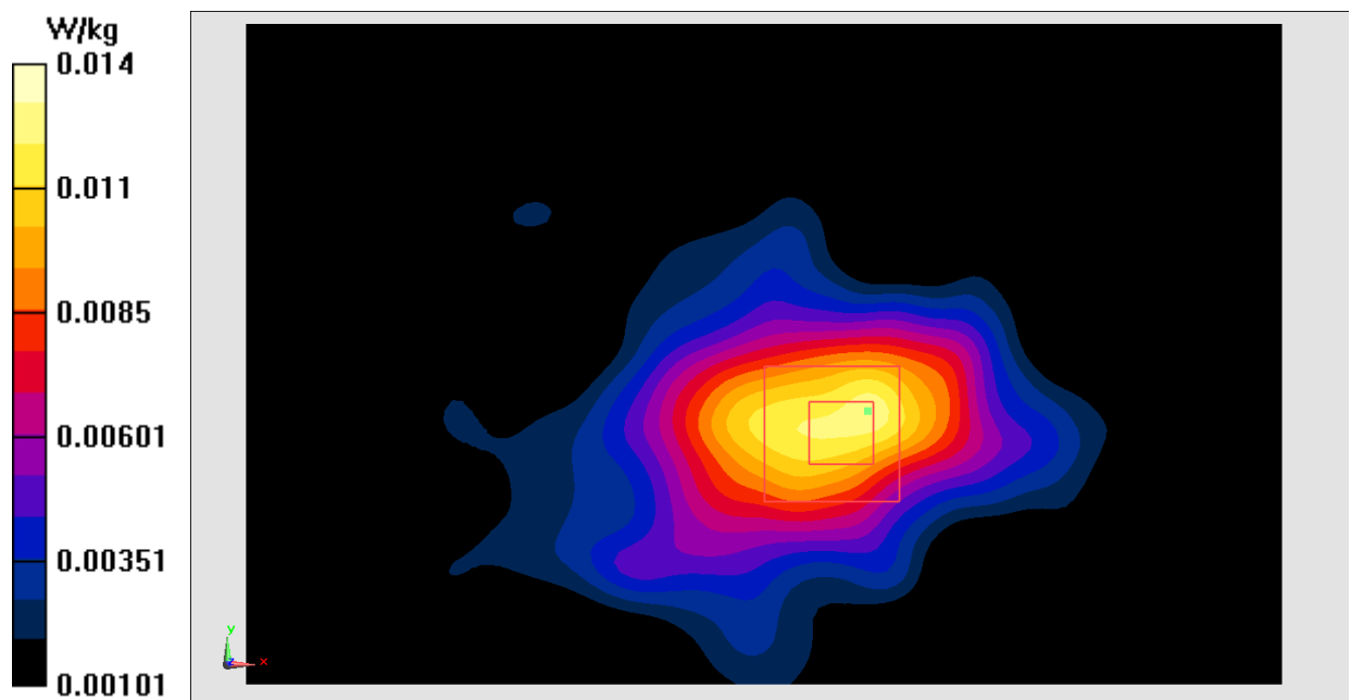
Fig.10 2450 MHz
