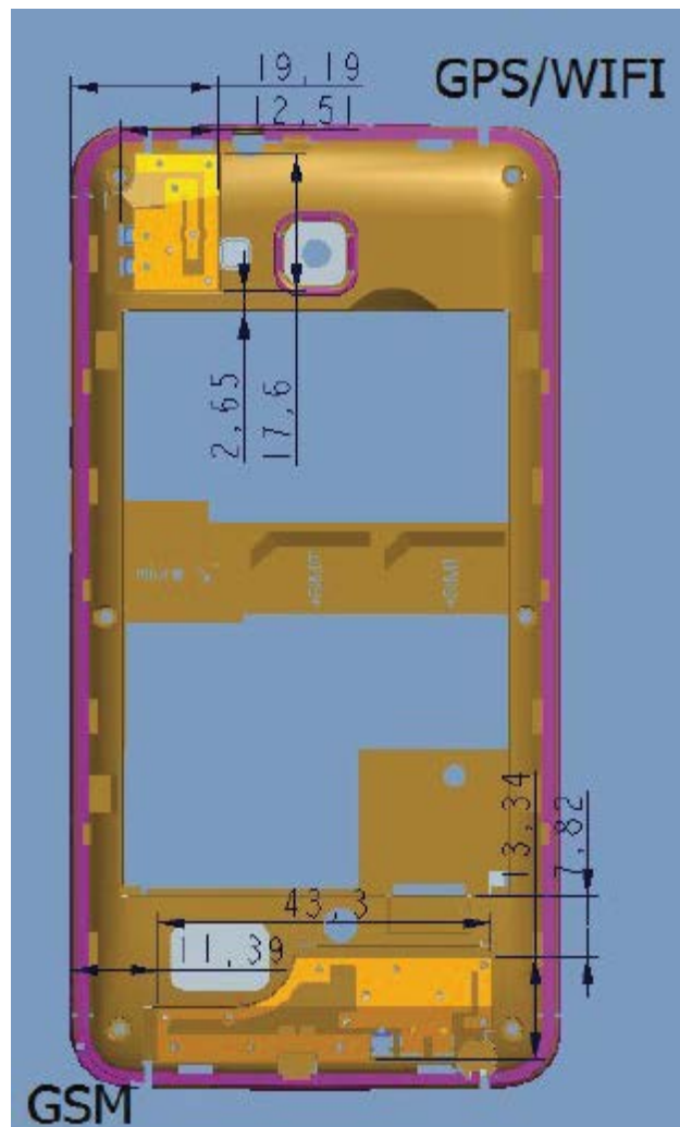
Picture 12.1 Antenna Locations
