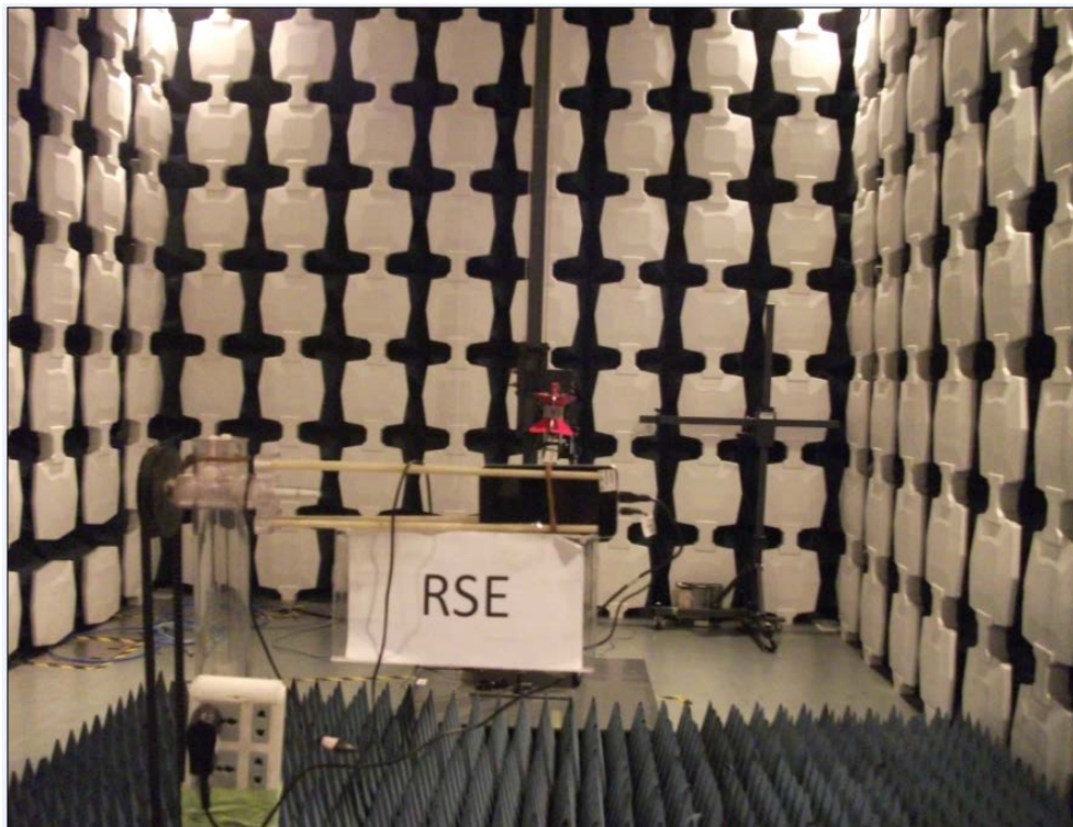
RSE Above 3GHz
