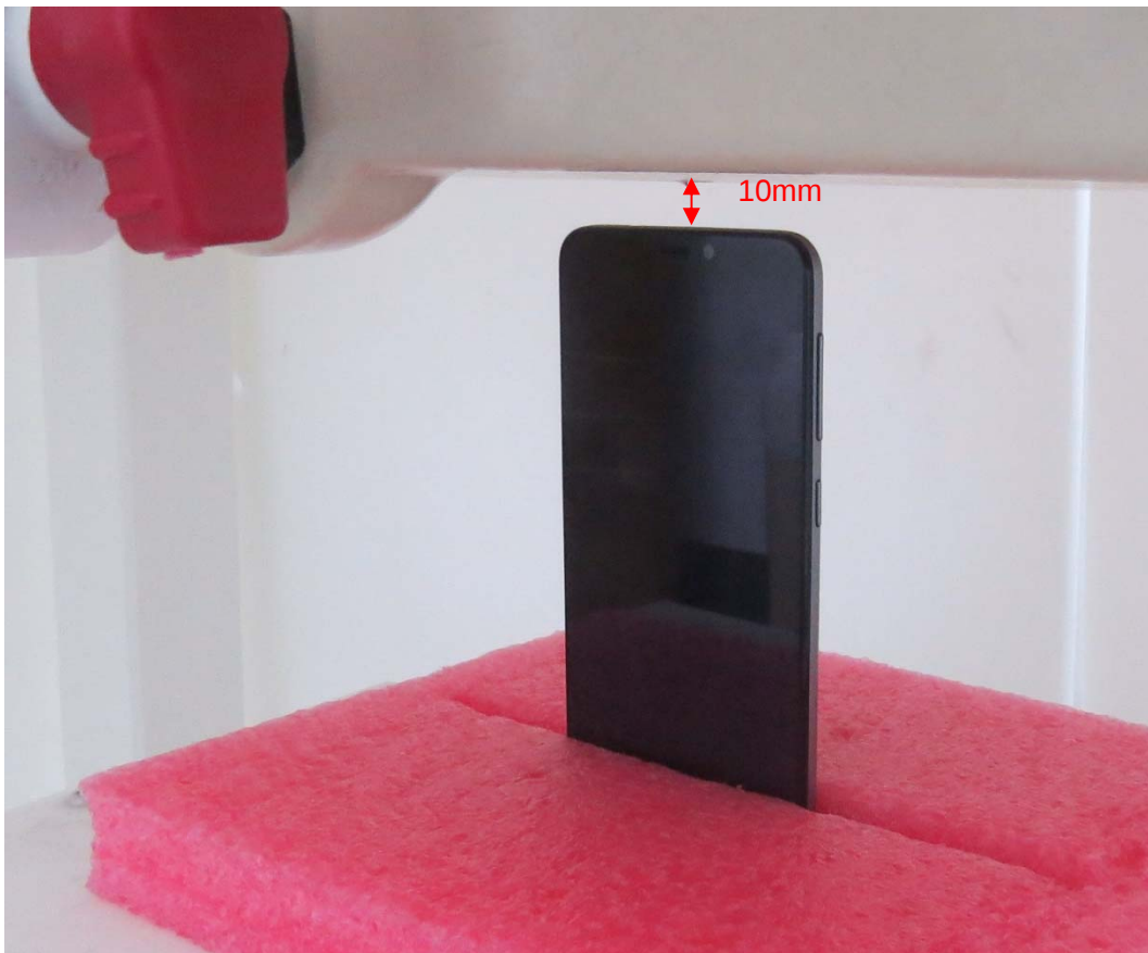
Picture 12: Top Side, the distance from handset to the bottom of the Phantom is 10mm
