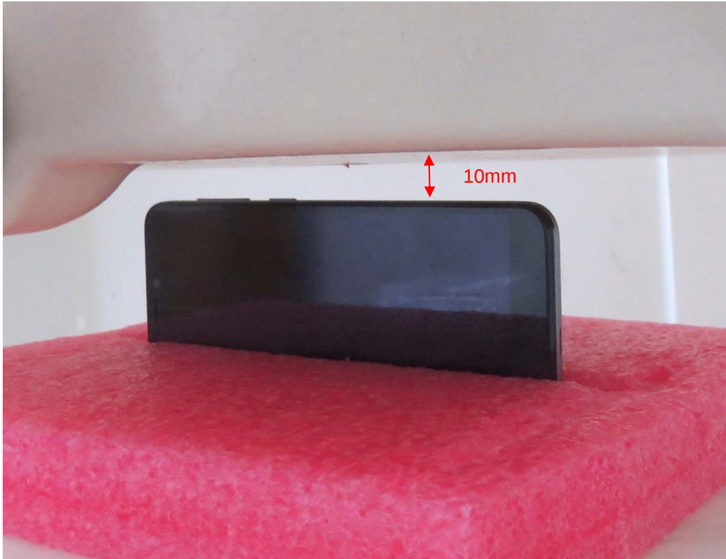
Picture 11: Right Side, the distance from handset to the bottom of the Phantom is 10mm
