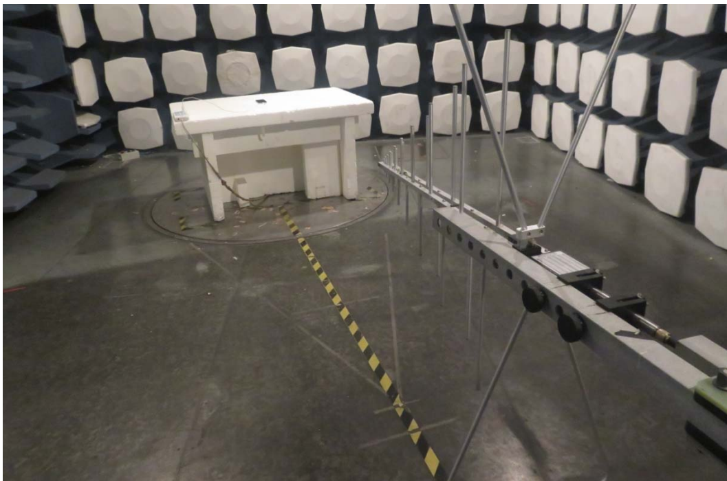
30MHz-1GHz
