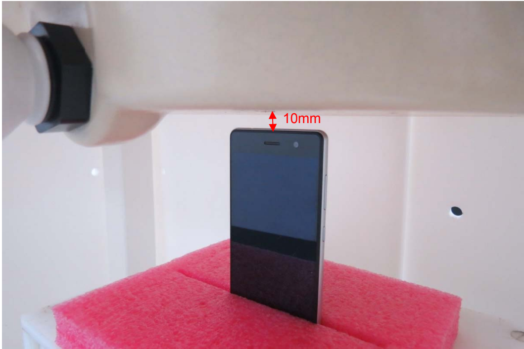
Picture 24: Top Side, the distance from handset to the bottom of the Phantom is 10mm
