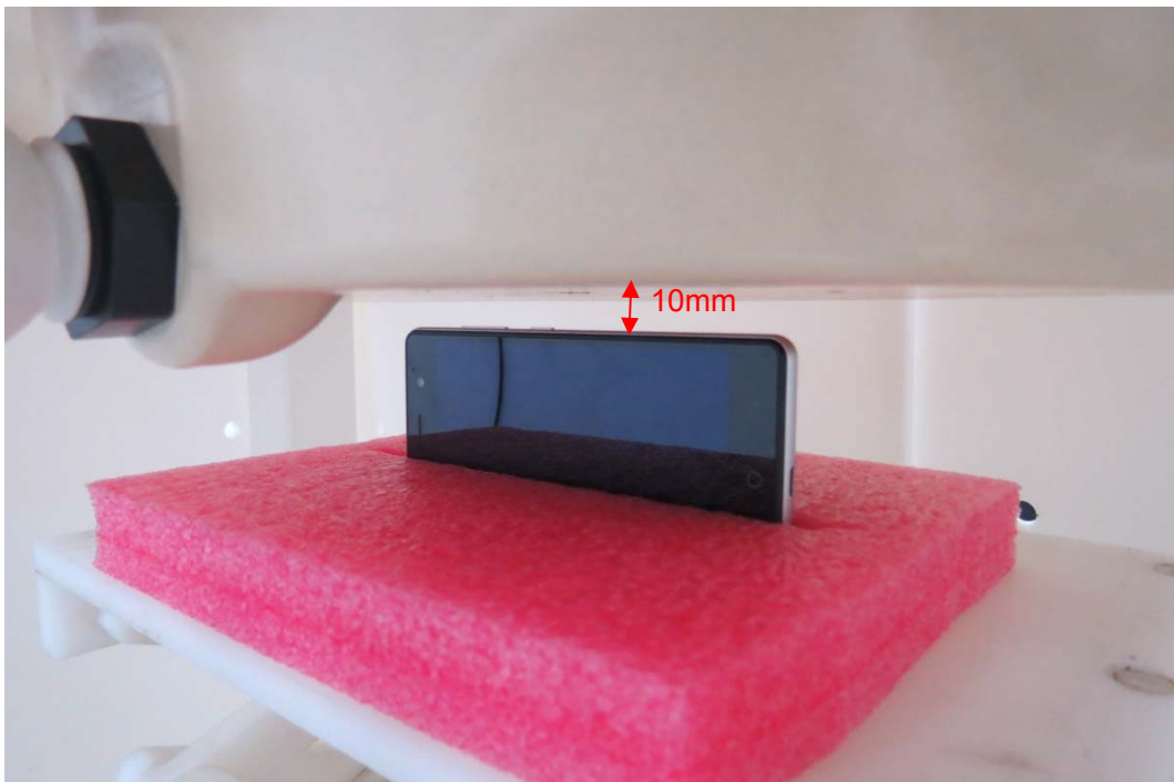
Picture 23: Right Side, the distance from handset to the bottom of the Phantom is 10mm
