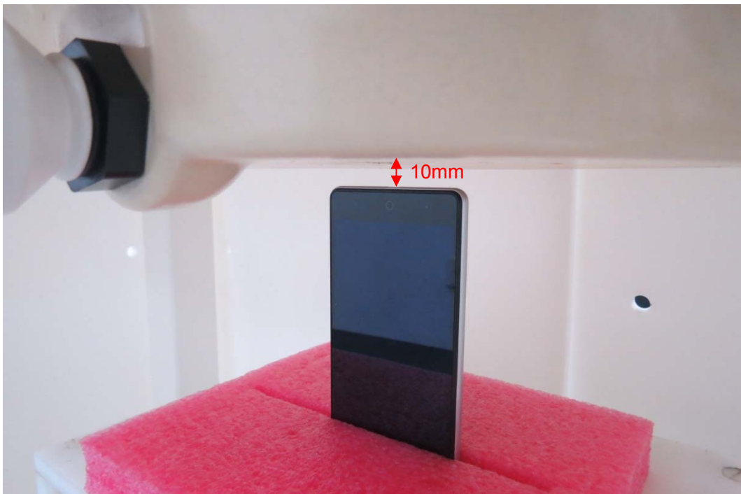
Picture 25: Bottom Side, the distance from handset to the bottom of the Phantom is 10mm
