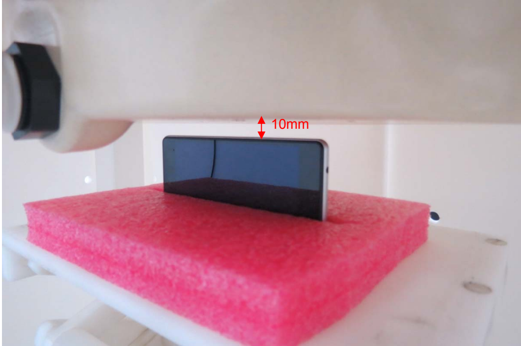
Picture 22: Left Side, the distance from handset to the bottom of the Phantom is 10mm
