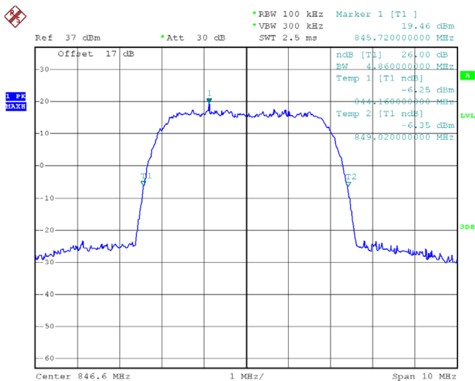
(Plot E5: WCDMA 850MHz Channel = 4233 26dB bandwidth)
