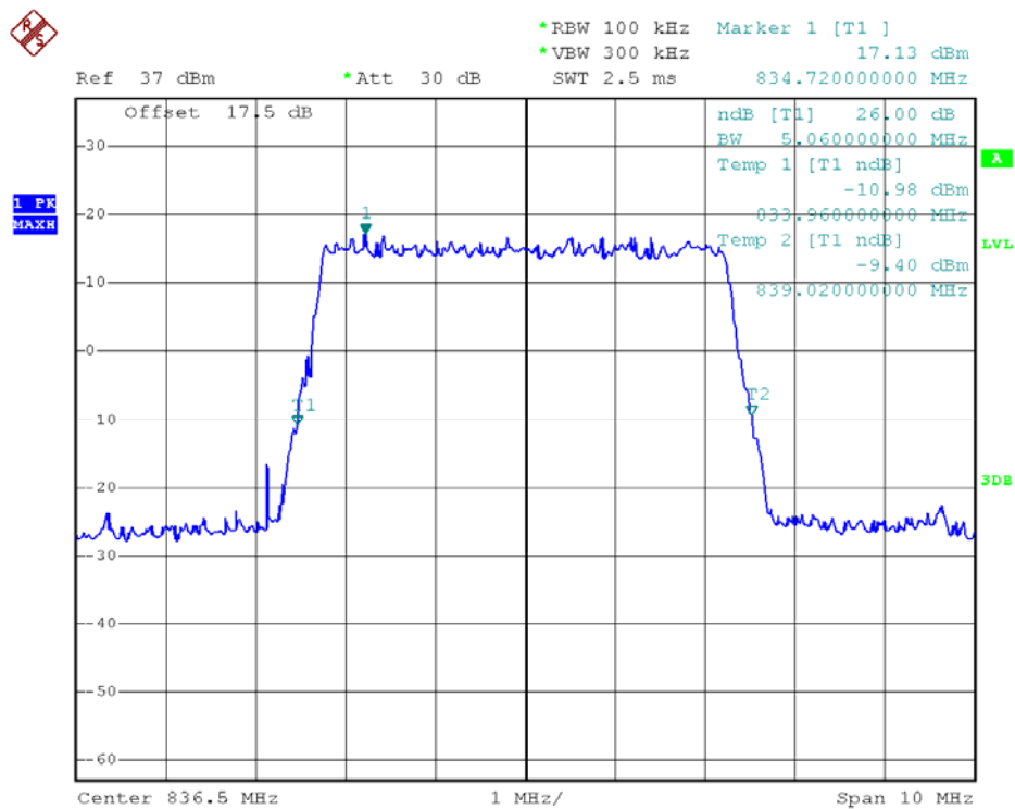
26dB Bandwidth LTE Band 5/5MHz/QPSK
