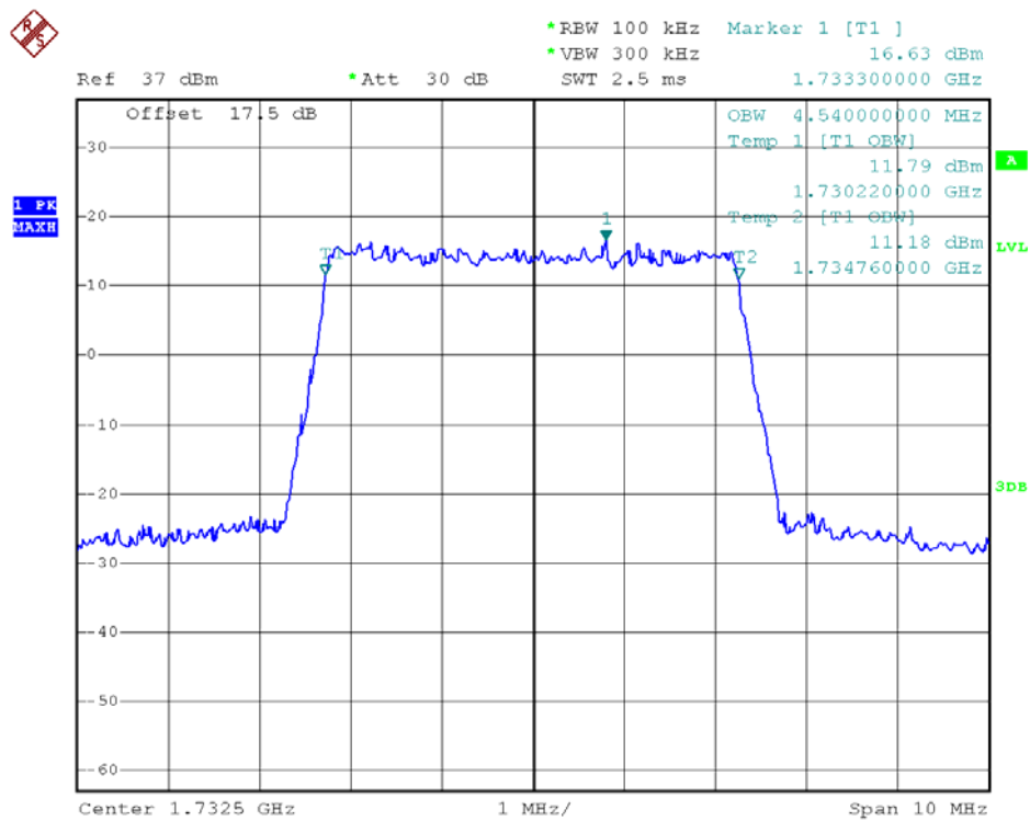
99% Occupied Bandwidth LTE Band 4/5MHz/QPSK
