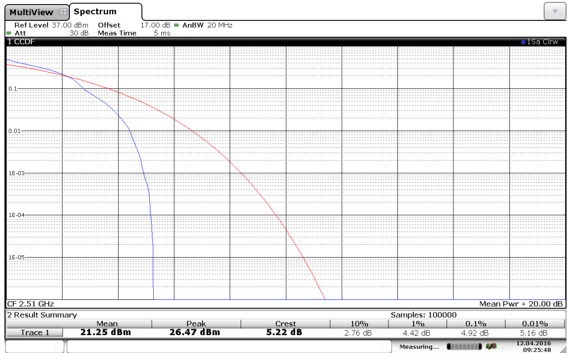
(Plot D1: Band 7/20MHz/16QAM in L Ch 1RB Size )
