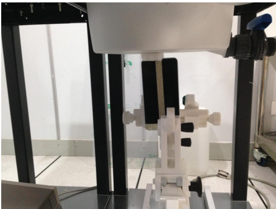
Fig.10 Body Edge C(UP,10mm separation)
