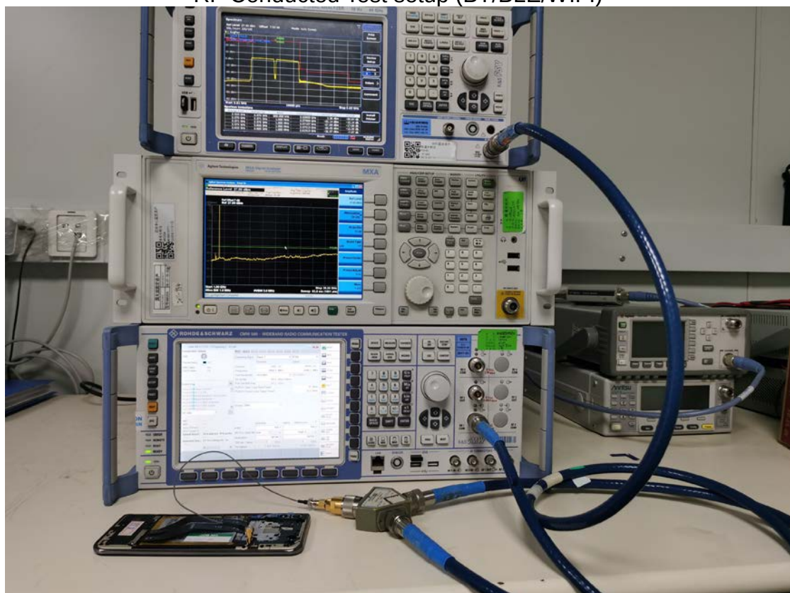
RF Conducted Test setup (GSM/WCDMA/LTE)
