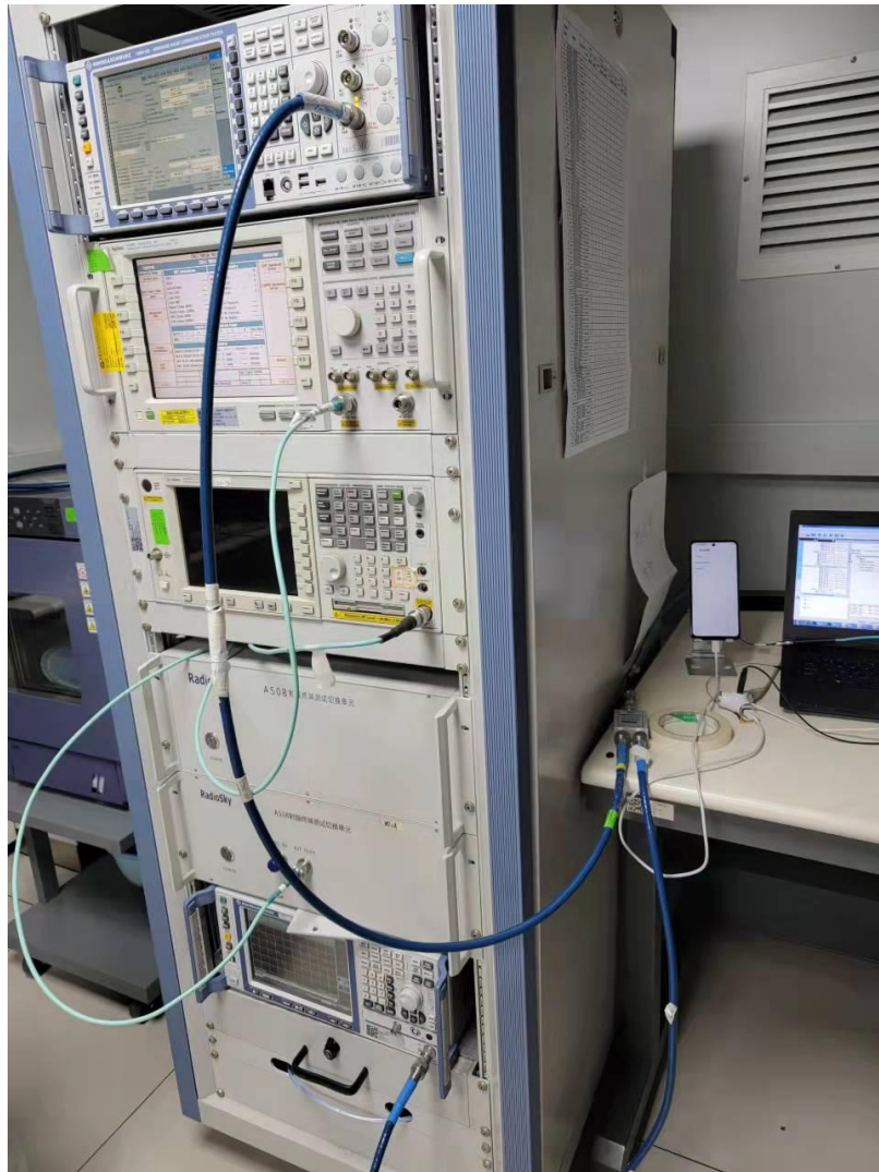
'RF Conducted Test setup (GSM/WCDMA/LTE)
