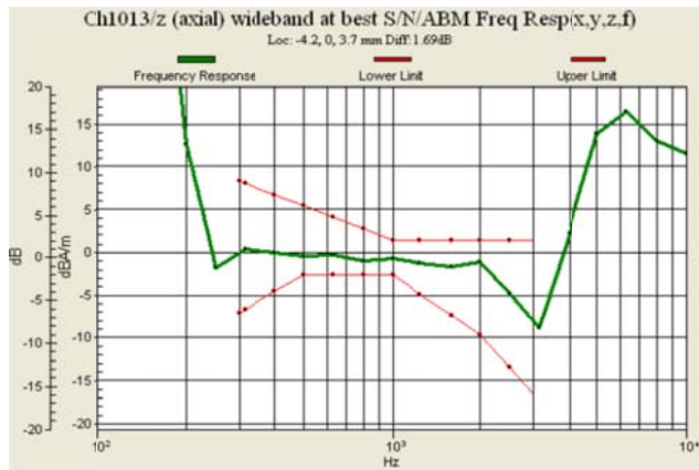
Fig 7.1 CDMA2000 BC0 Ch1013
