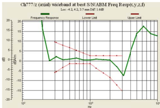
Fig 7.3 CDMA2000 BC0 Ch777
