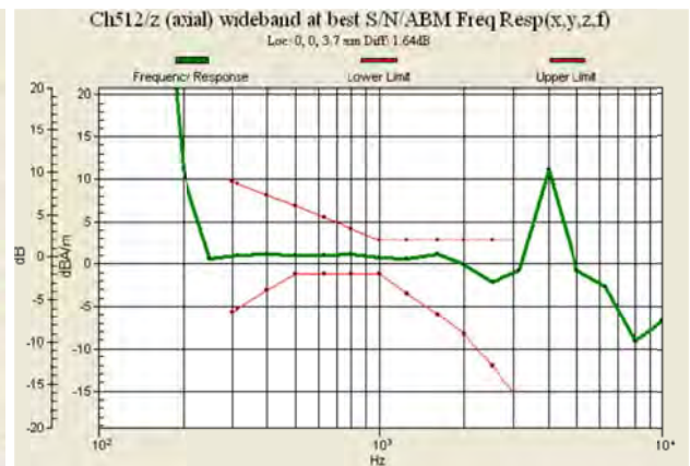
Fig 7.4 GSM1900 Ch512
