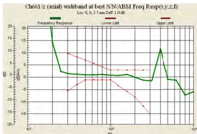
Fig 7.5 GSM1900 Ch661
