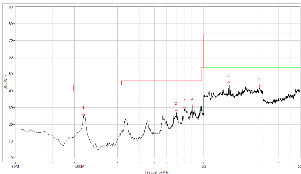
(Plot B: 30MHz – 6GHz, Test Antenna Horizontal)
