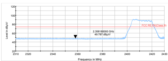
802.11g-Channel 1 Peak
