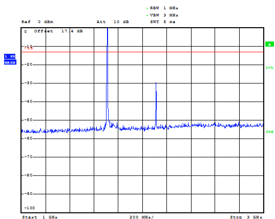
LTE Band 66 3MHz CH-Low 1GHz~3GHz
