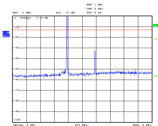
LTE Band 66 1.4MHz CH-High 1GHz~3GHz
