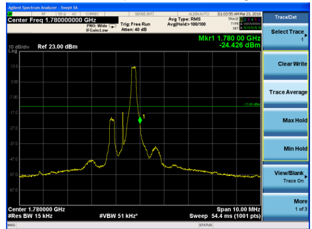
LTE Band 66 16QAM 1.4MHz CH-High, 1 RB
