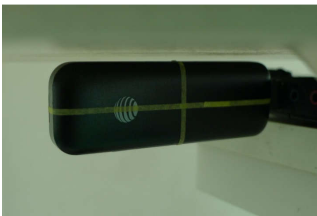
Vertical Back, Test Separation 5 mm
