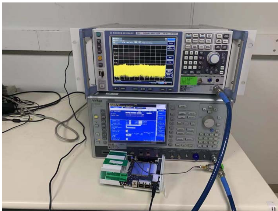
RF Conducted Test setup (WCDMA/LTE)
