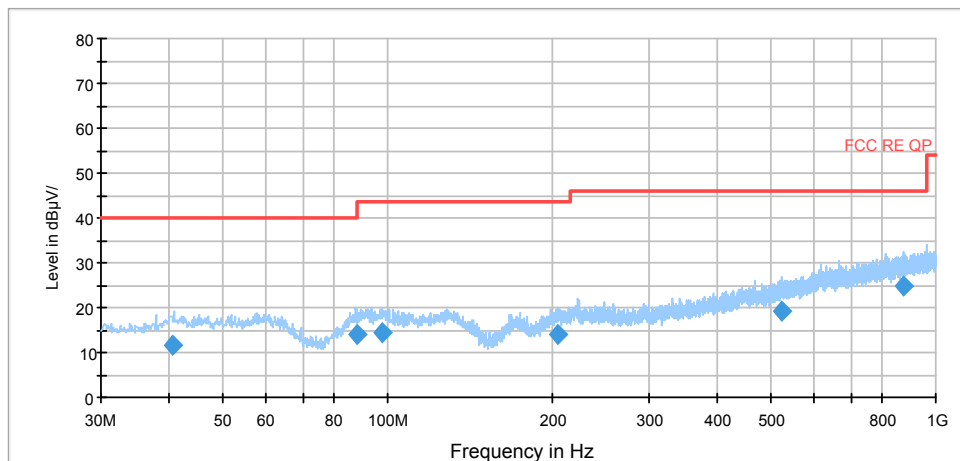
Radiates Emission from 30MHz to 1GHz (Vertical)
