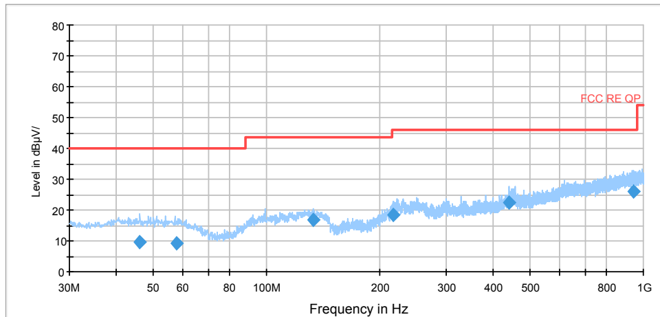
Radiates Emission from 30MHz to 1GHz (Horizontal)
