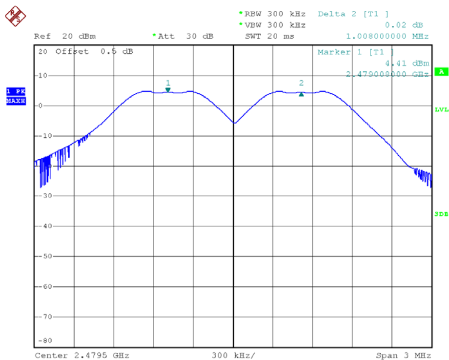
GFSK High Channel Mode
