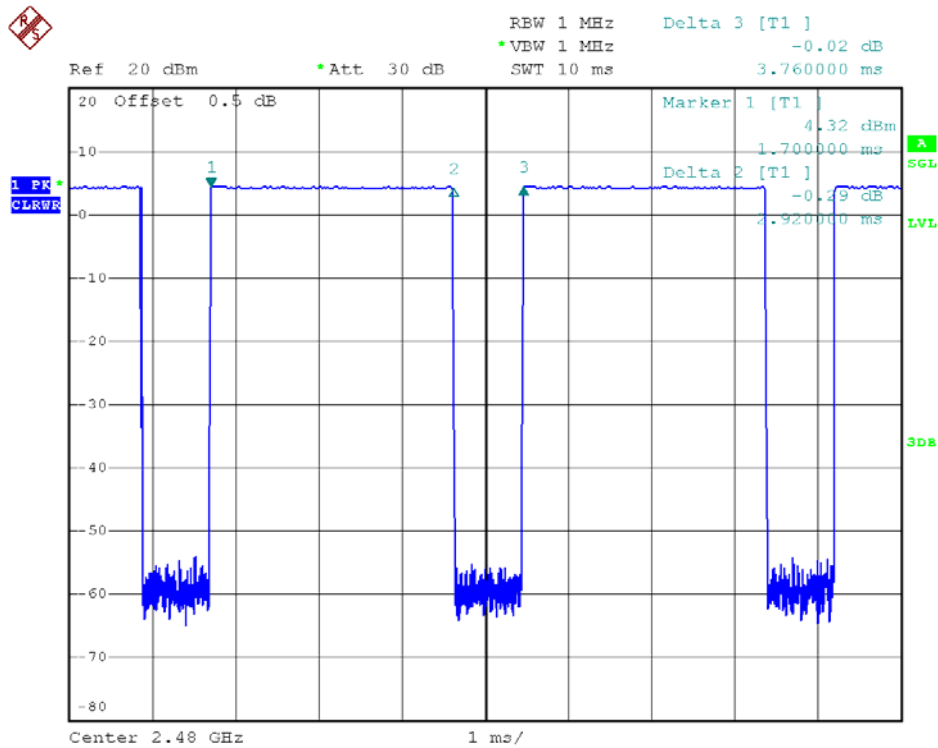
78 Channel @ DH5
