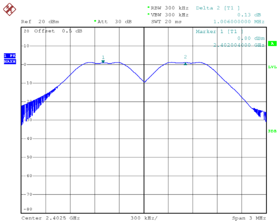
GFSK Low Channel Mode
