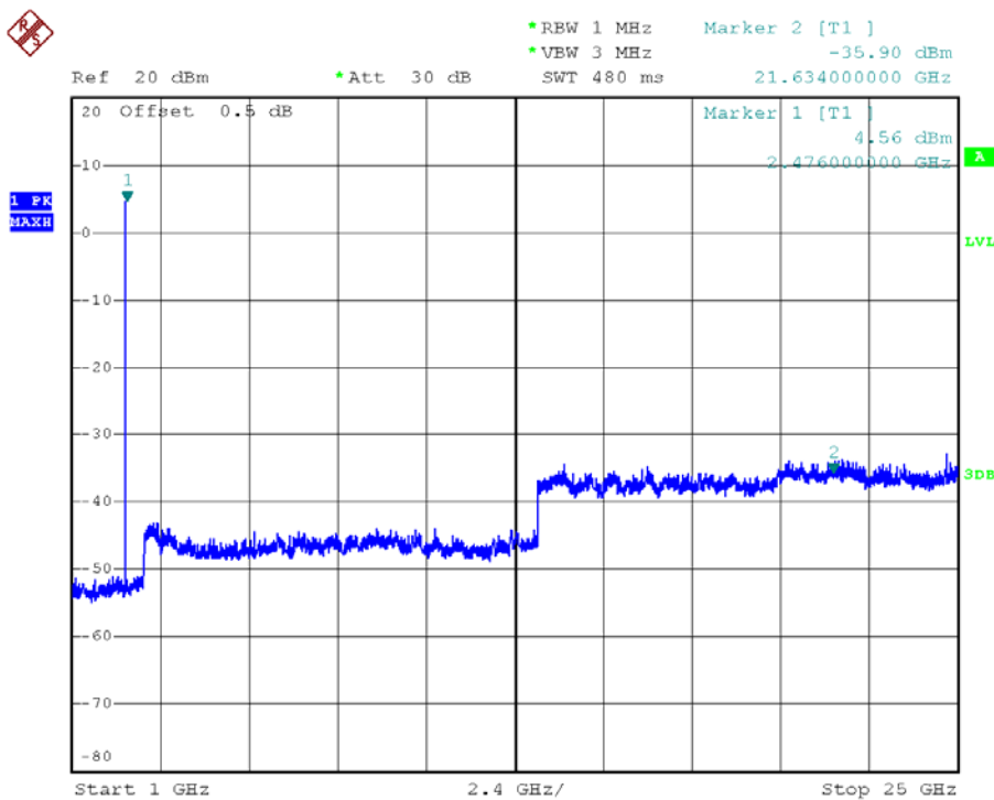
High Channel 1GHz to 25GHz @ GFSK Mode
