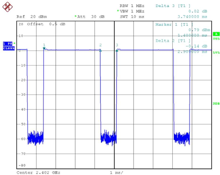
0 Channel @ DH5
