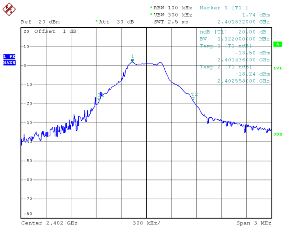
(Plot A: 0 Channel @ GFSK)
