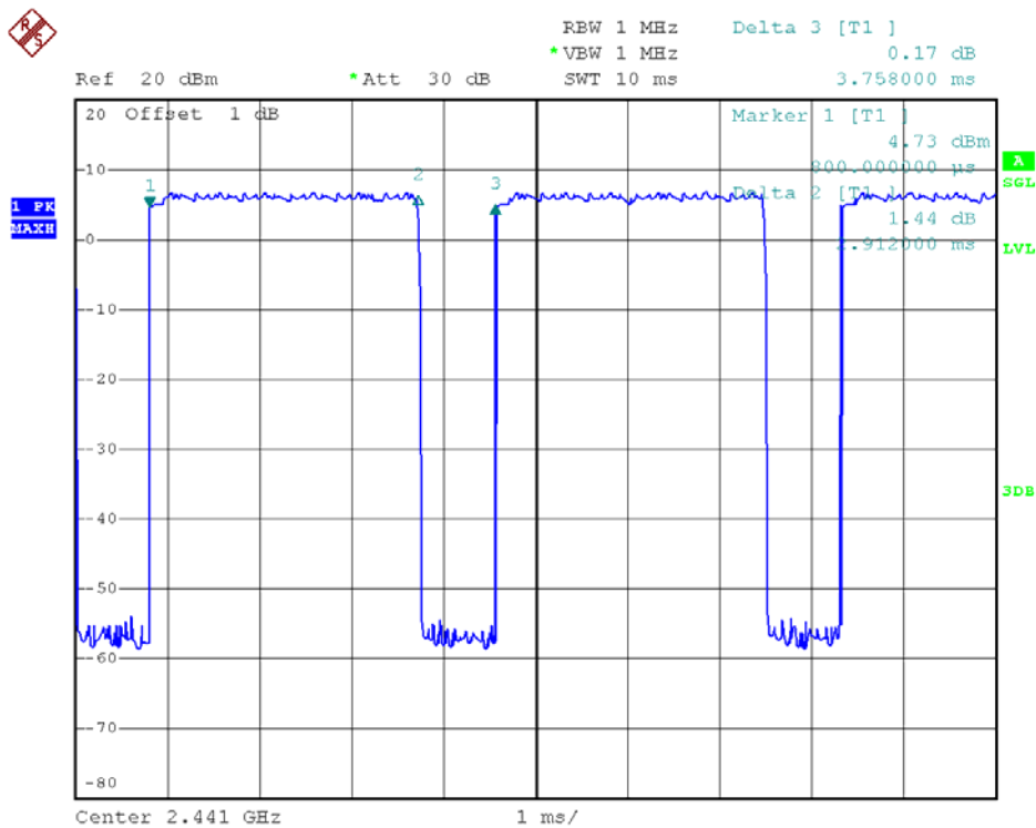
39 Channel @ 3DH5
