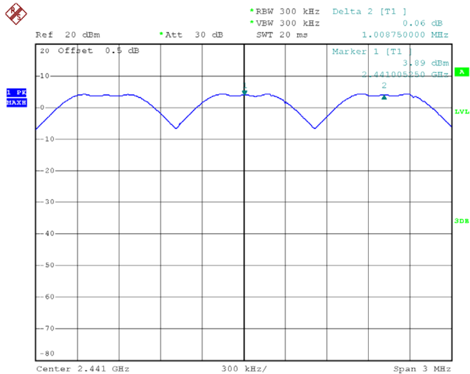
GFSK Middle Channel Mode
