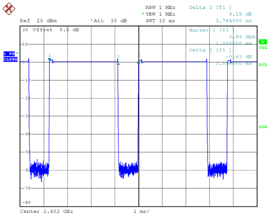
0 Channel @ 2DH5
