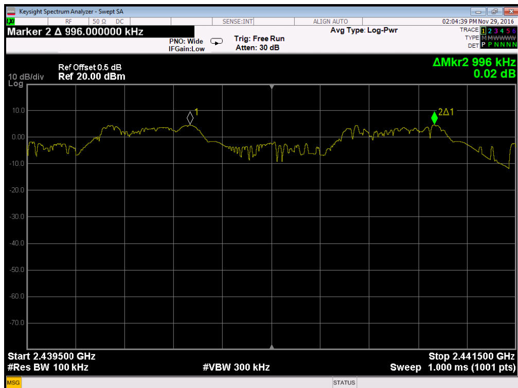
8-DPSK Mode
