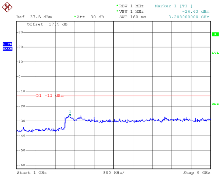
WCDMA850MHz Channel = 4132, 1GHz to 9GHz
