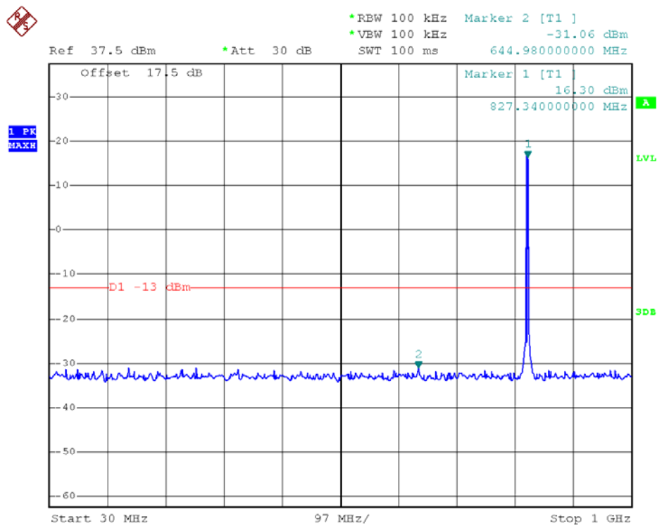
WCDMA850MHz Channel = 4132, 30MHz to 1GHz
