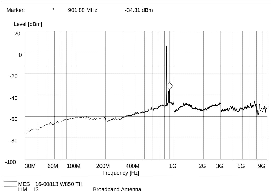
WCDMA 850MHz, Test Antenna Horizontal
