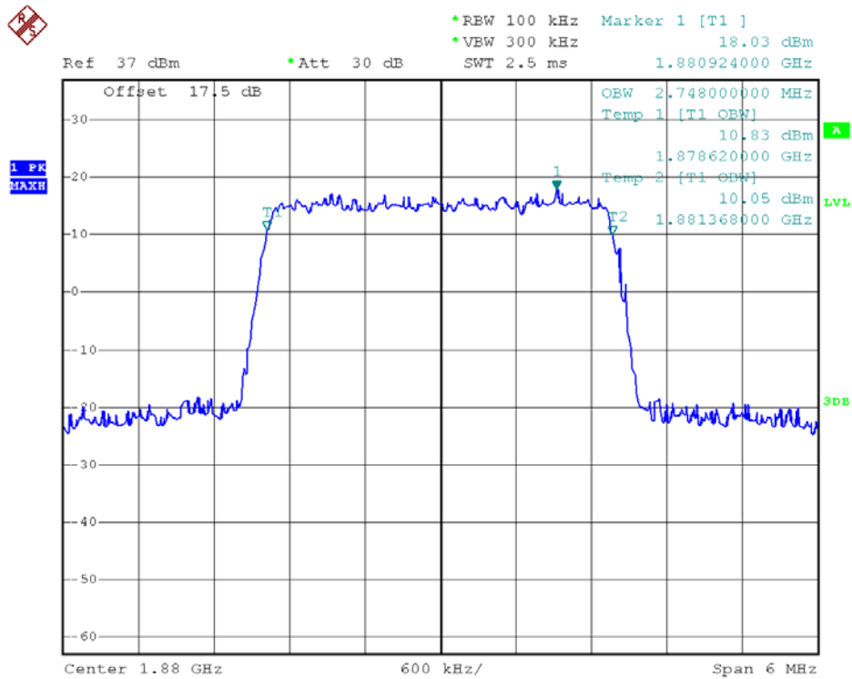
99% Occupied Bandwidth LTE Band 2/3MHz/16QAM
