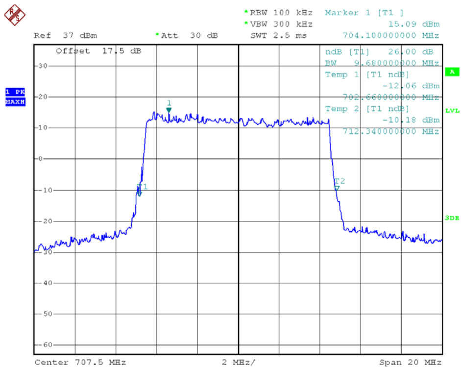
26dB Bandwidth LTE Band 12/10MHz/QPSK
