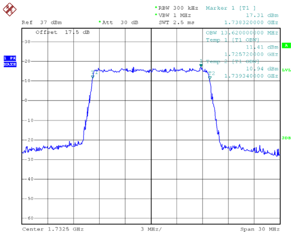
99% Occupied Bandwidth LTE Band 4/15MHz/QPSK
