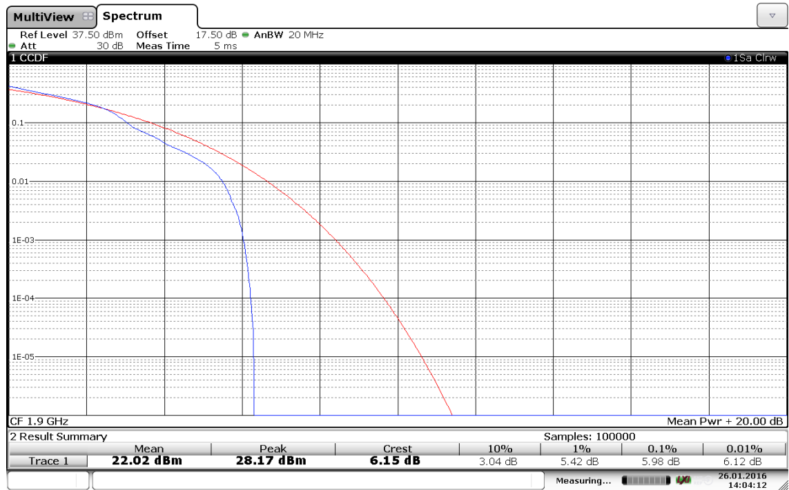
(Plot A5: Band 2/20MHz/16QAM in H Ch 1RB Size)
