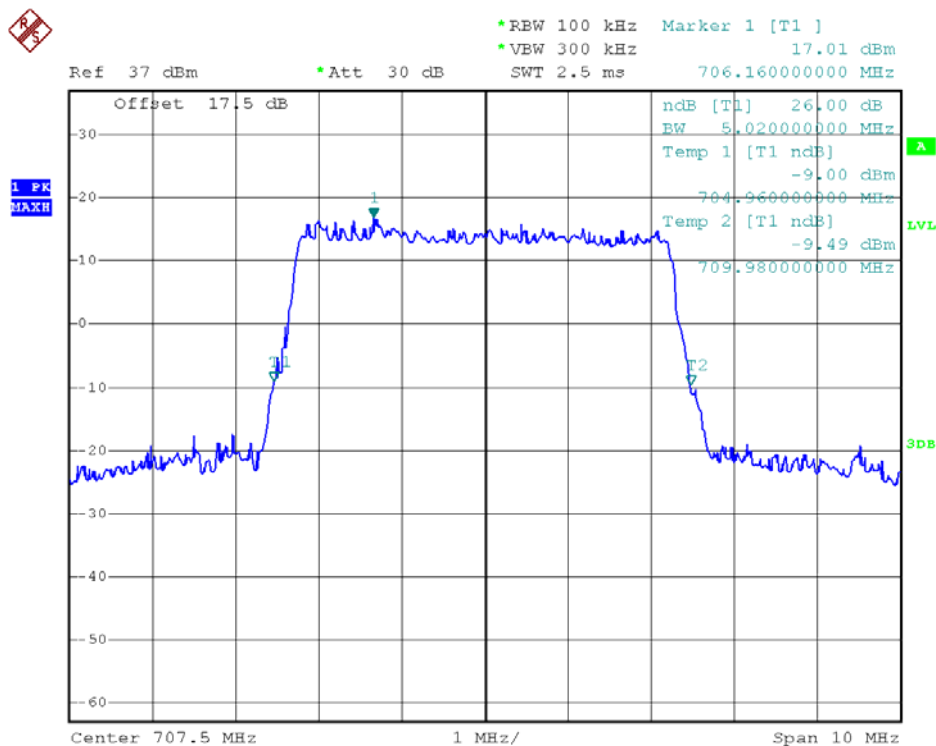
26dB Bandwidth LTE Band 12/5MHz/16QAM
