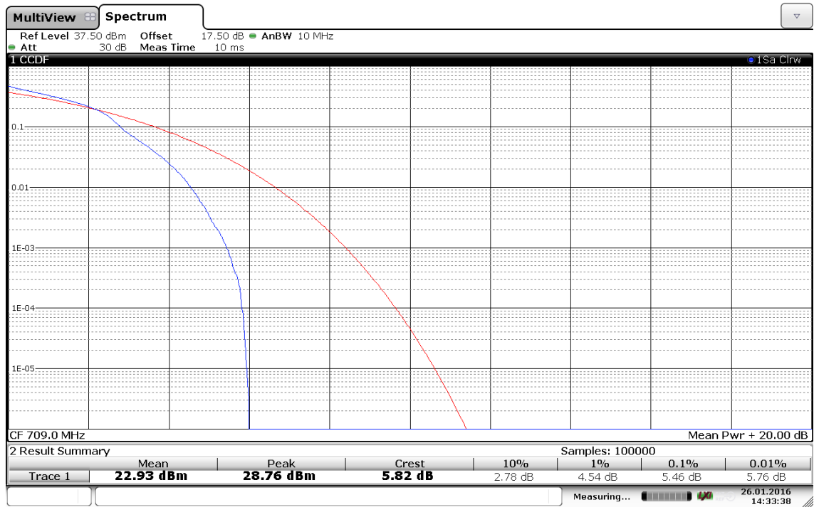
(Plot F1: Band 17/10MHz/16QAM in L Ch 1RB Size )
