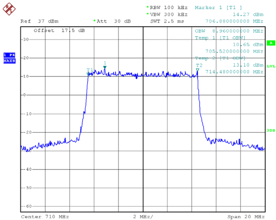
99% Occupied Bandwidth LTE Band 17/10MHz/16QAM
