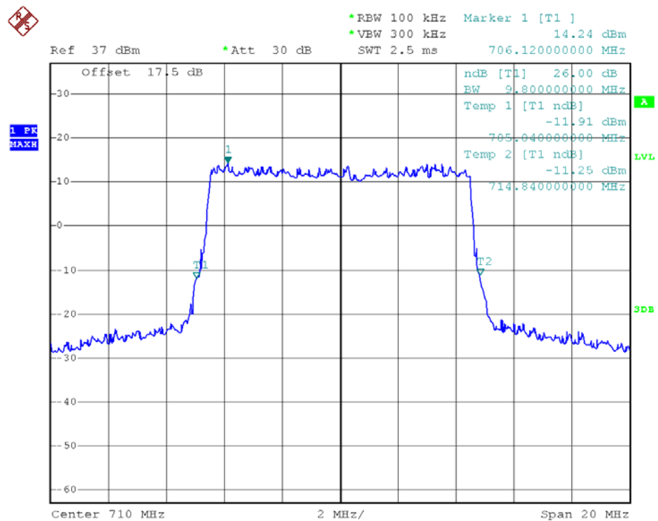
26dB Bandwidth LTE Band 17/10MHz/QPSK
