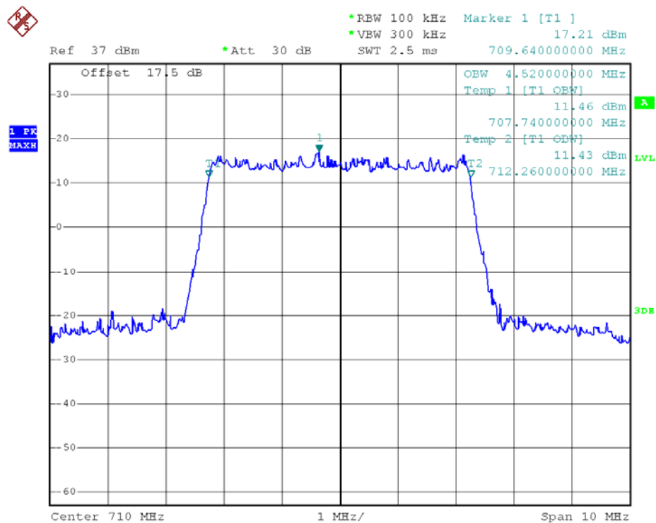
99% Occupied Bandwidth LTE Band 17/5MHz/16QAM
