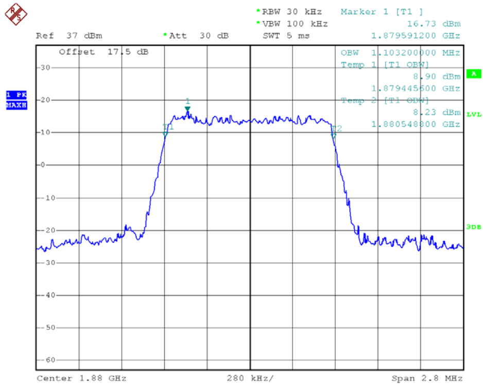
99% Occupied Bandwidth LTE Band 2 1.4MHz/16QAM
