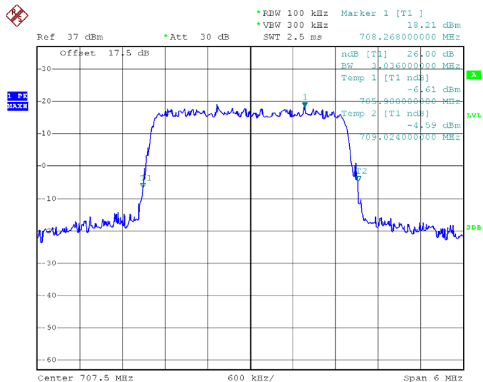
26dB Bandwidth LTE Band 12/3MHz/16QAM
