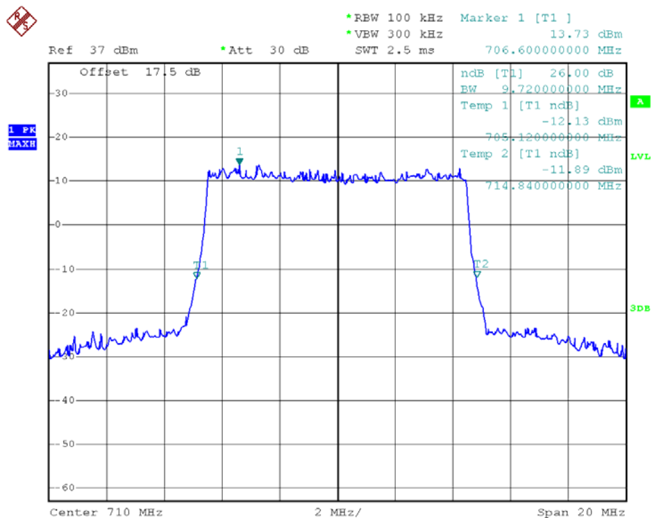
26dB Bandwidth LTE Band 17/10MHz/16QAM
