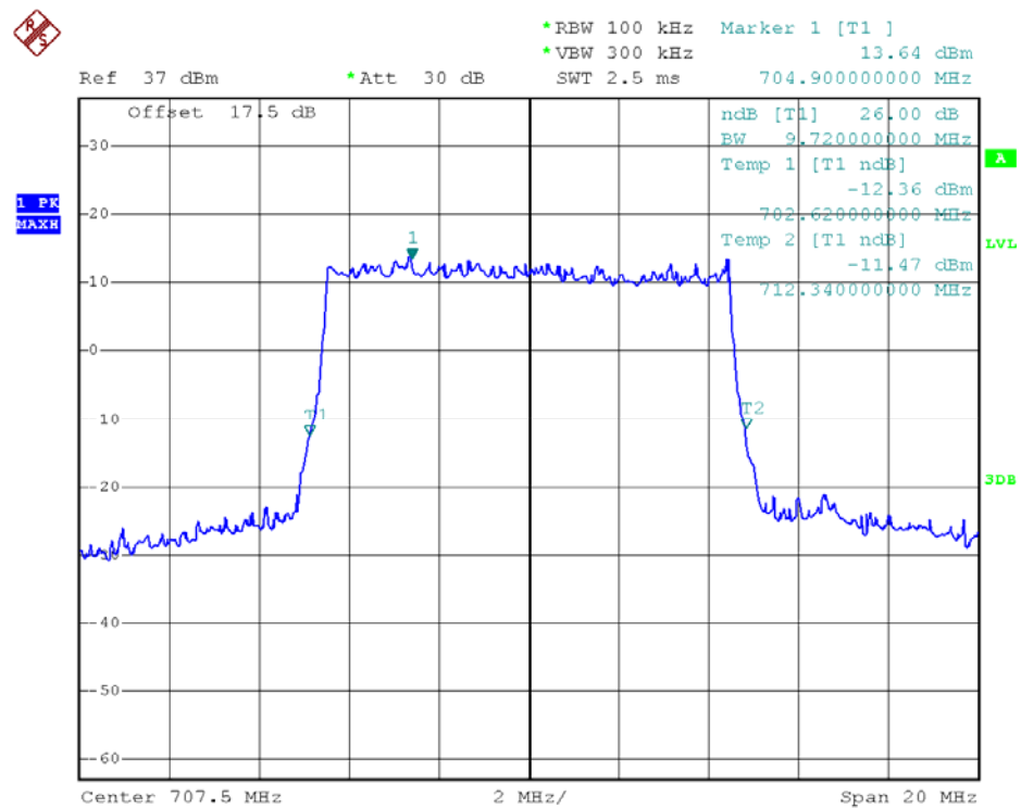
26dB Bandwidth LTE Band 12/10MHz/16QAM
