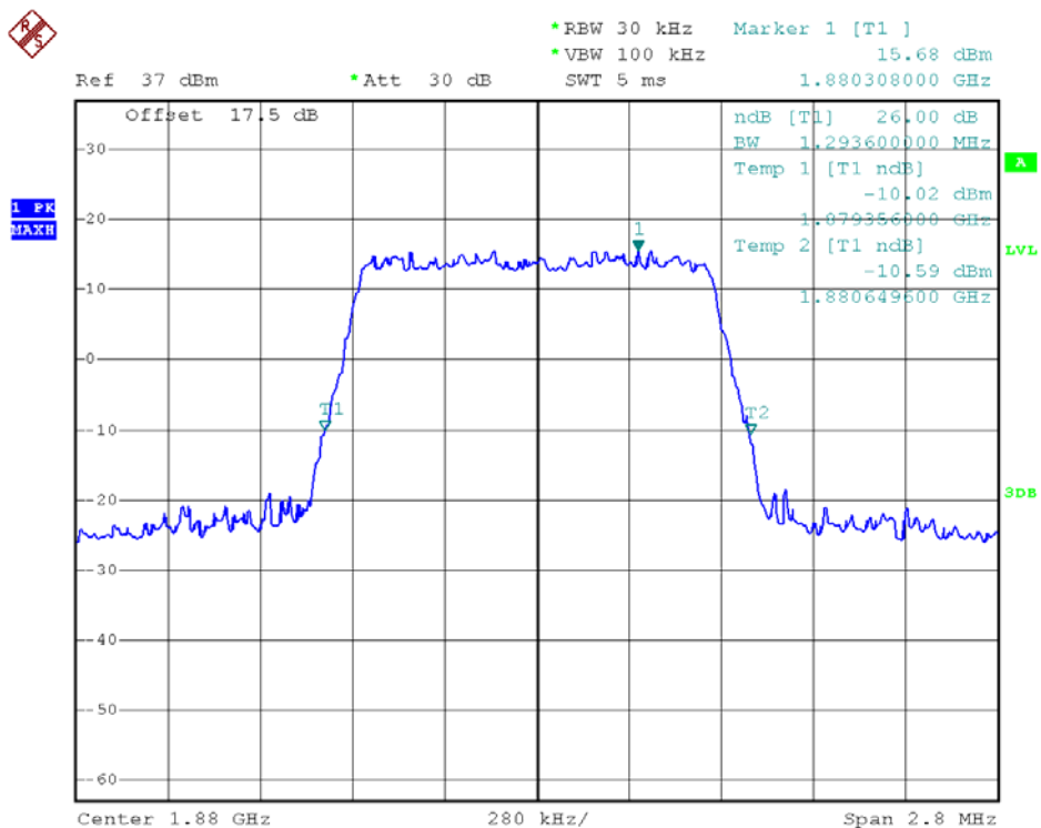
26dB Bandwidth LTE Band 2 1.4MHz/16QAM
