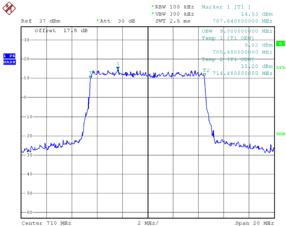
99% Occupied Bandwidth LTE Band 17/10MHz/QPSK
