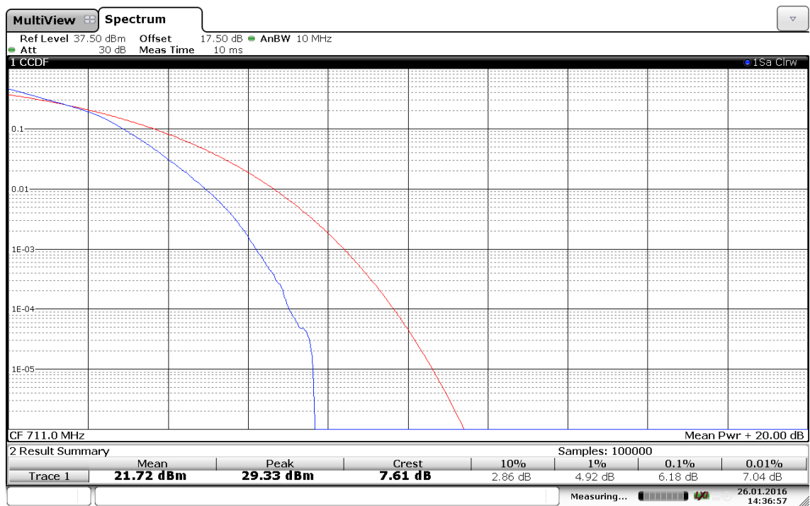
(Plot F5: Band 17/10MHz/16QAM in H Ch 1RB Size)
