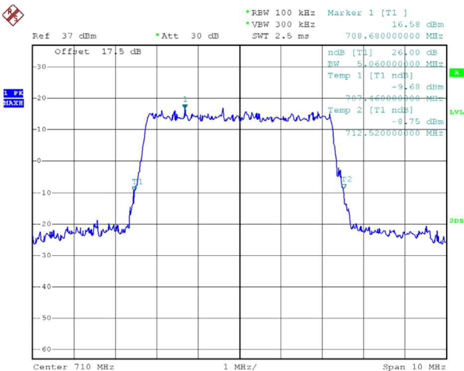
26dB Bandwidth LTE Band 17/5MHz/16QAM
