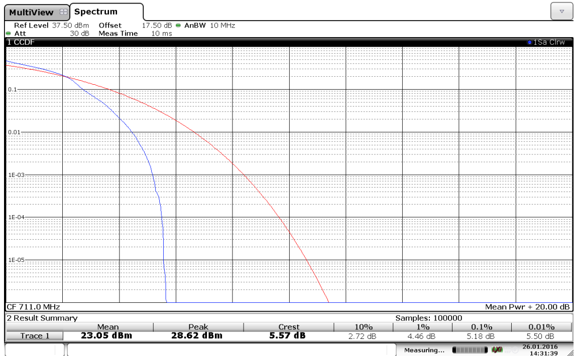
(Plot E5: Band 12/10MHz/16QAM in H Ch 1RB Size)
