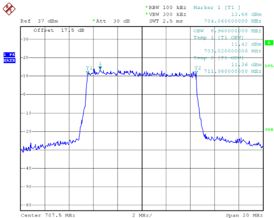
99% Occupied Bandwidth LTE Band 12/10MHz/16QAM
