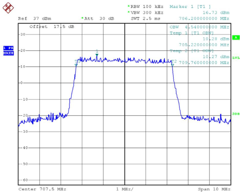
99% Occupied Bandwidth LTE Band 12/5MHz/16QAM
