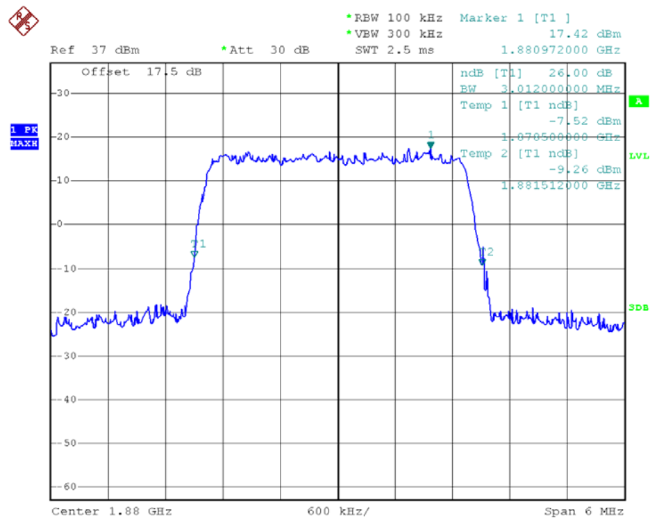
26dB Bandwidth LTE Band 2/3MHz/16QAM
