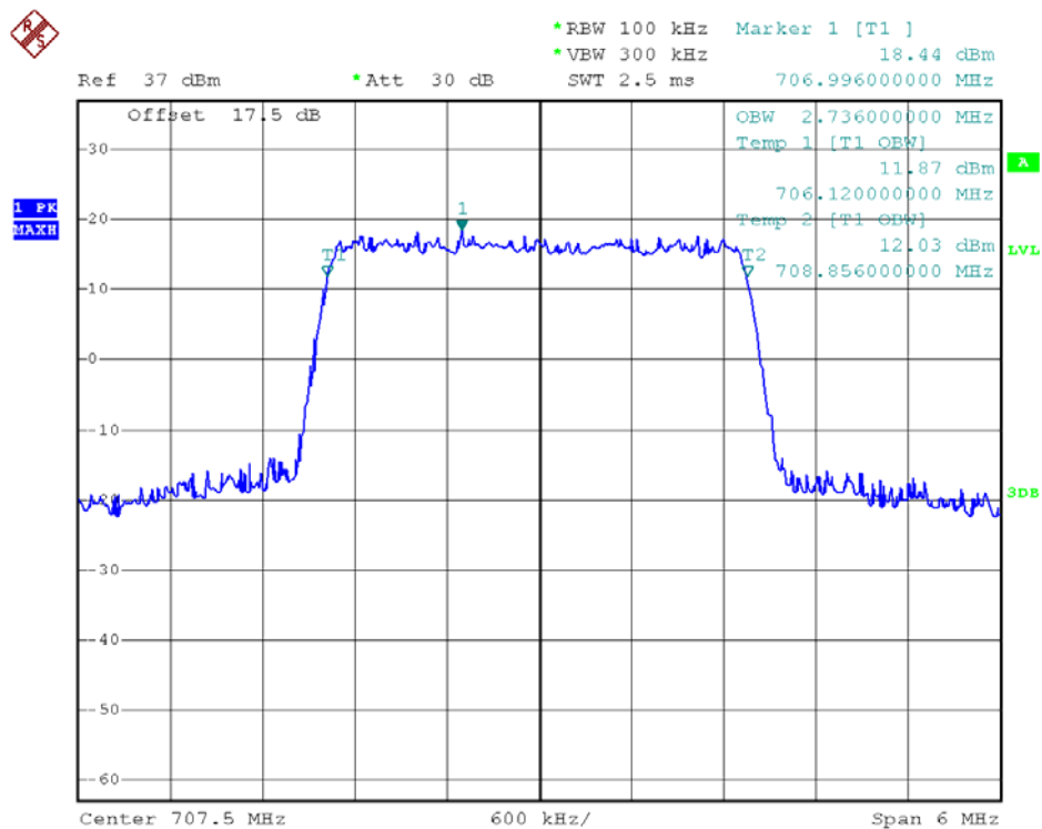
99% Occupied Bandwidth LTE Band 12/3MHz/16QAM
