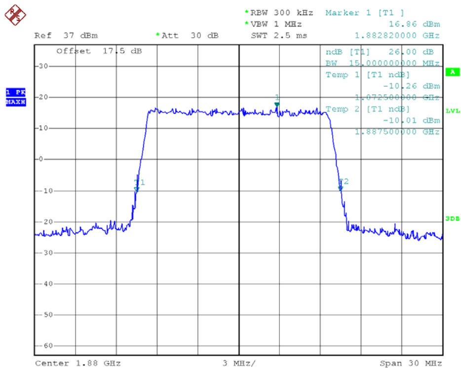
26dB Bandwidth LTE Band 2/15MHz/QPSK
