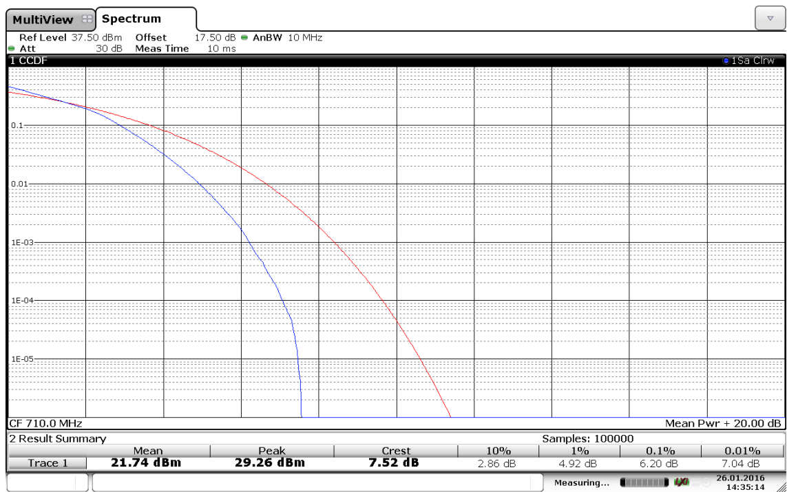
(Plot F3: Band 17/10MHz/16QAM in M Ch 1RB Size)
