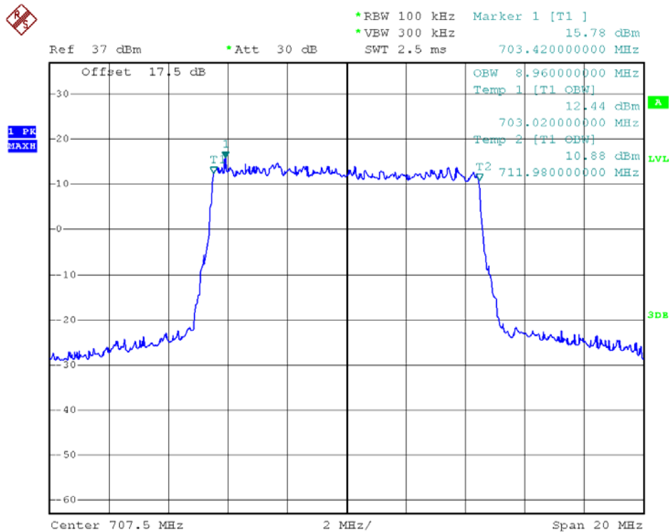
99% Occupied Bandwidth LTE Band 12/10MHz/QPSK
