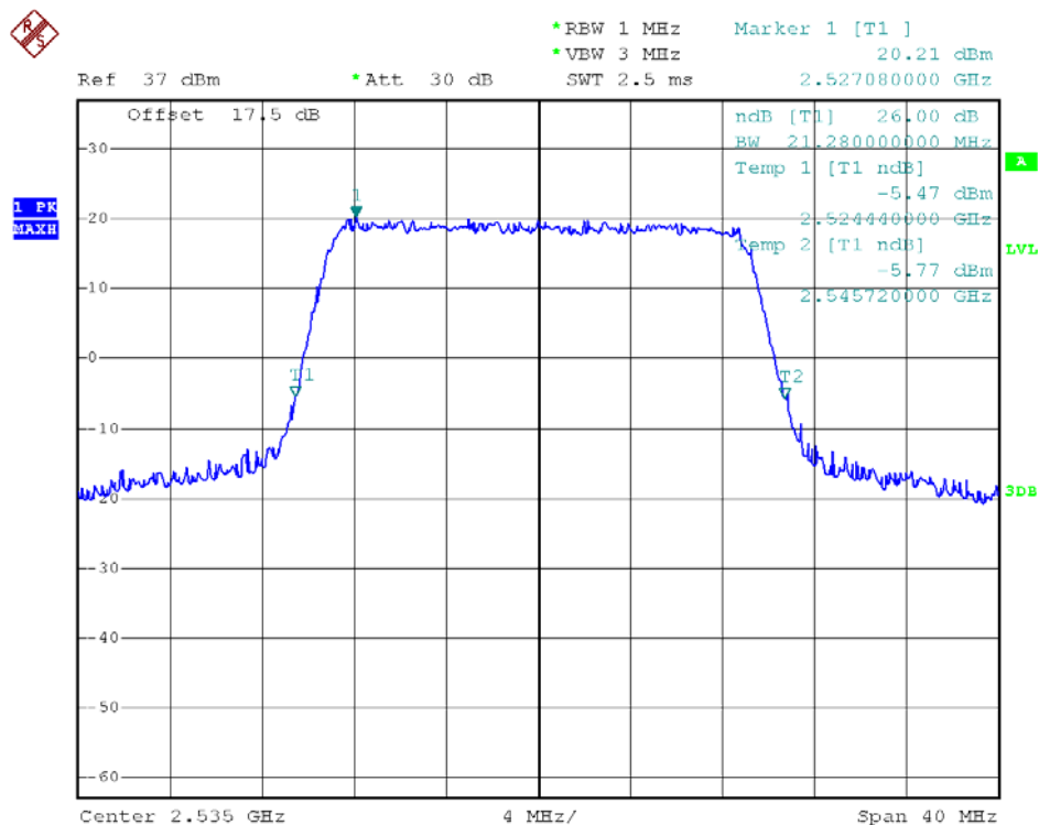
26dB Bandwidth LTE Band 7/20MHz/QPSK
