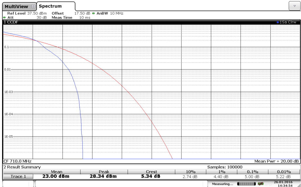
(Plot F3: Band 17/10MHz/16QAM in M Ch 1RB Size)
