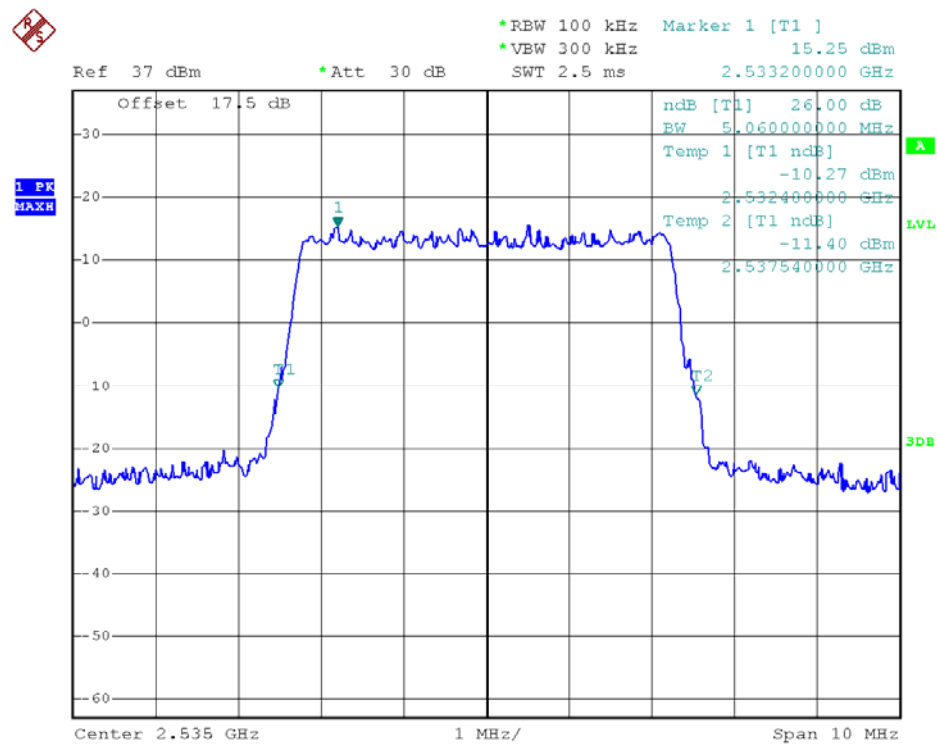
26dB Bandwidth LTE Band 7/5MHz/QPSK
