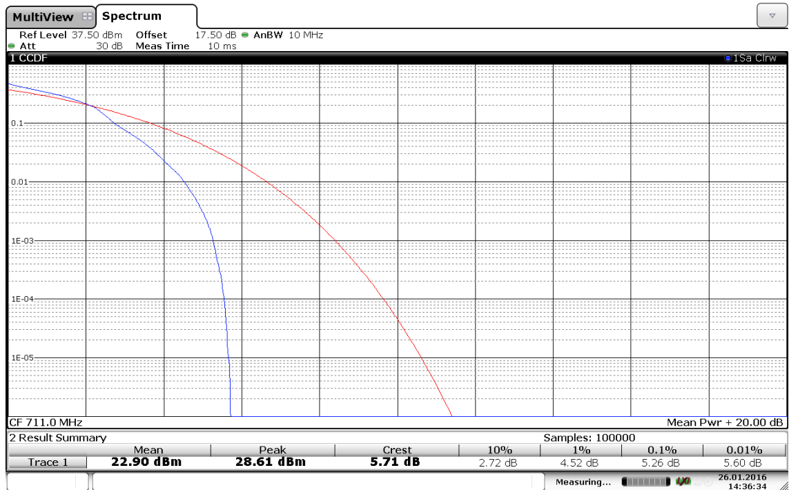
(Plot F5: Band 17/10MHz/16QAM in H Ch 1RB Size)
