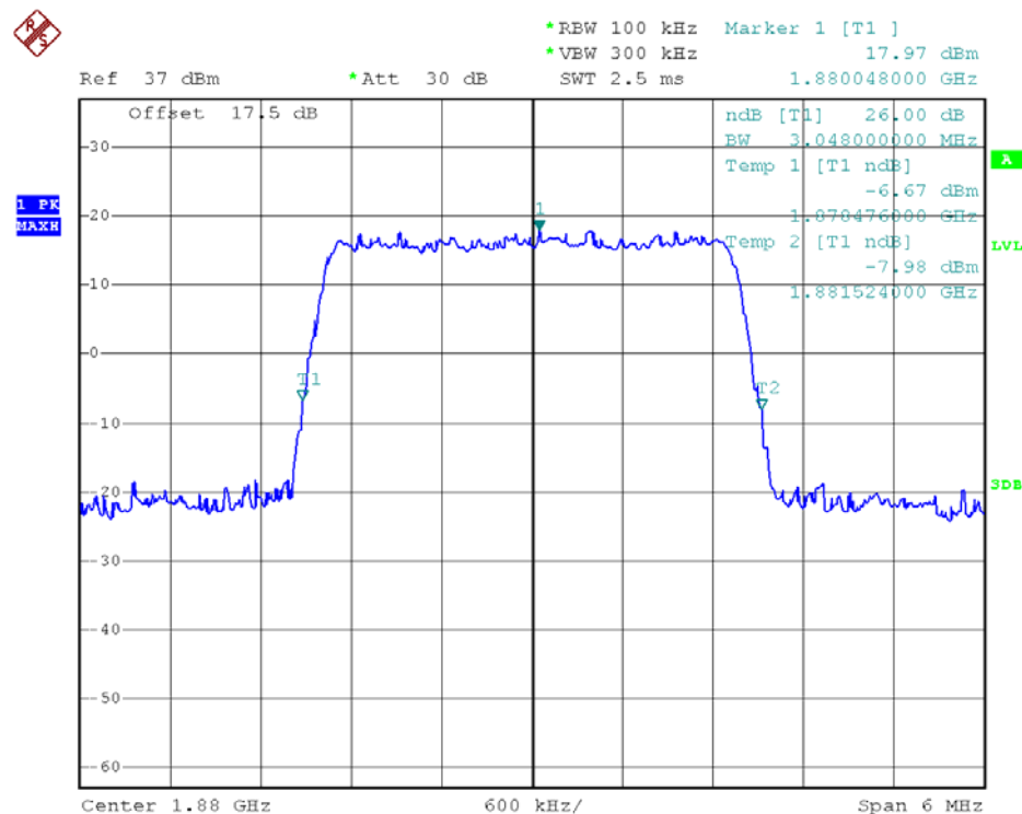
26dB Bandwidth LTE Band 2/3MHz/QPSK
