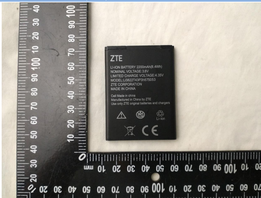
THE PHOTO OF BATTERY (BACK)
