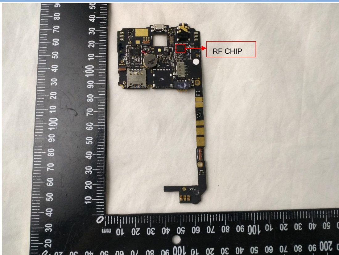
MAIN BOARD 1 FRONT VIEW 2
