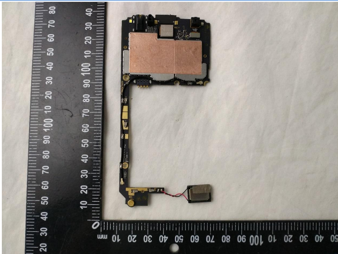
MAIN BOARD 1 BACK VIEW 1
