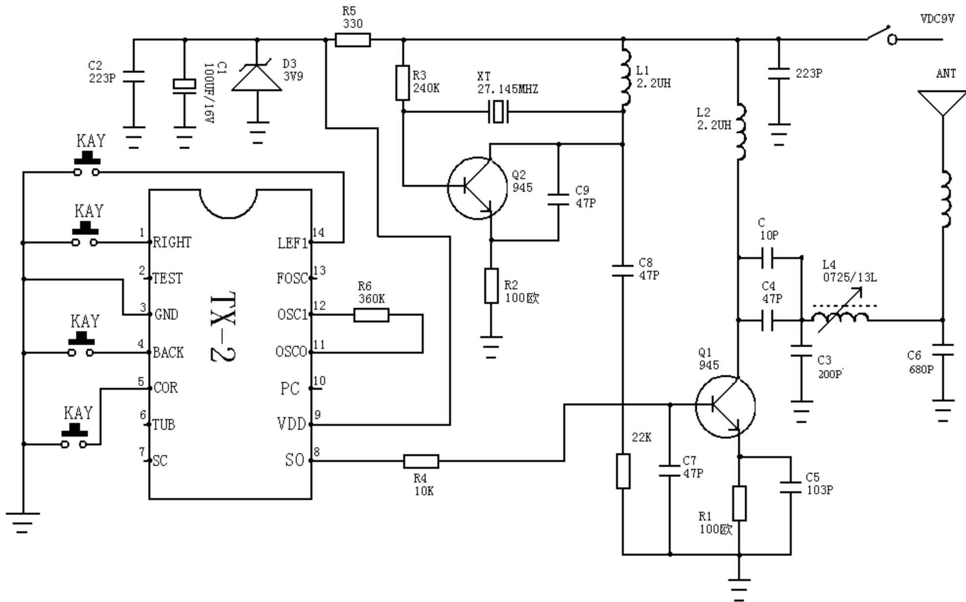
The transmit principle chart
