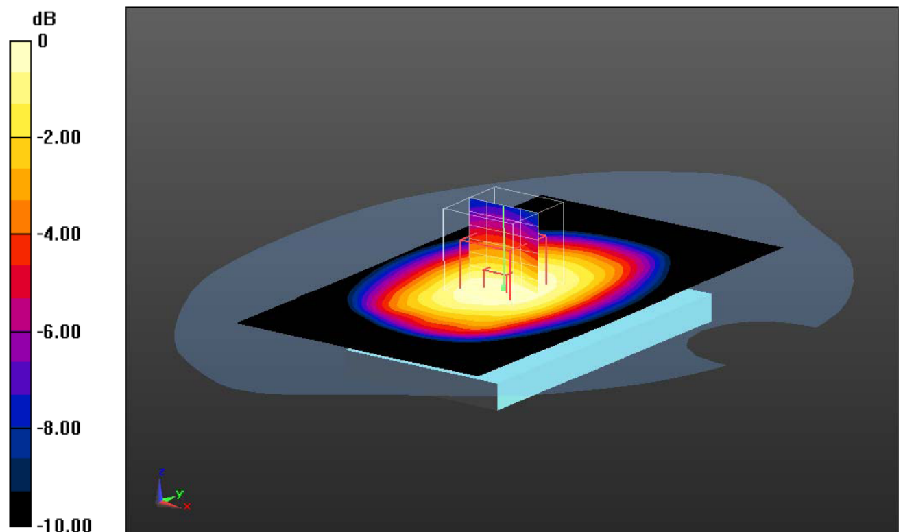
Figure 2: Face held for FRS Analog Front towards Phantom 467.6375 MHz
