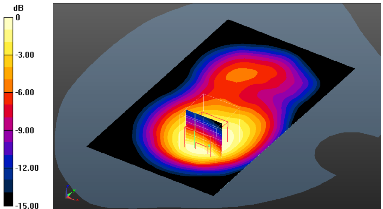
Figure 1: Face held for GMRS Analog Front towards Phantom 462.6375 MHz
