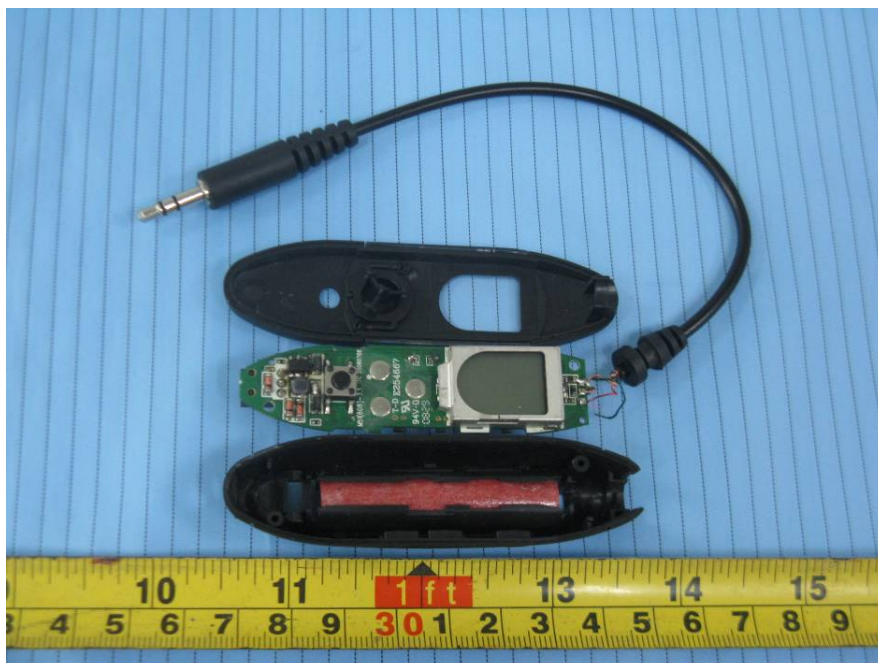
EUT – EUT Uncovered View 2
