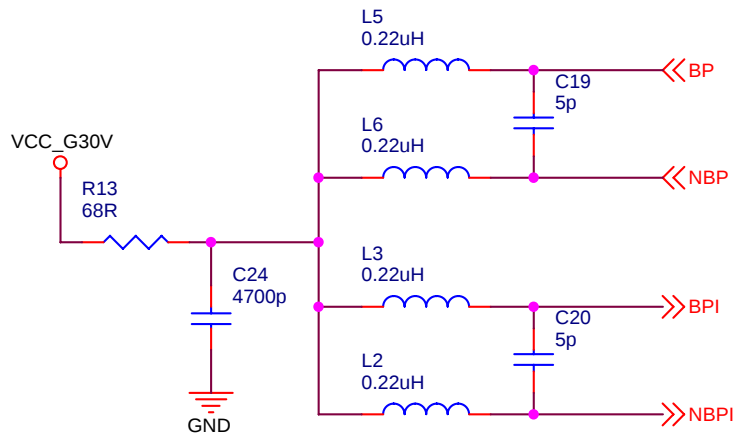
IF-Filter Interface
