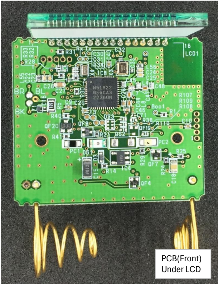
PCB(Front)
